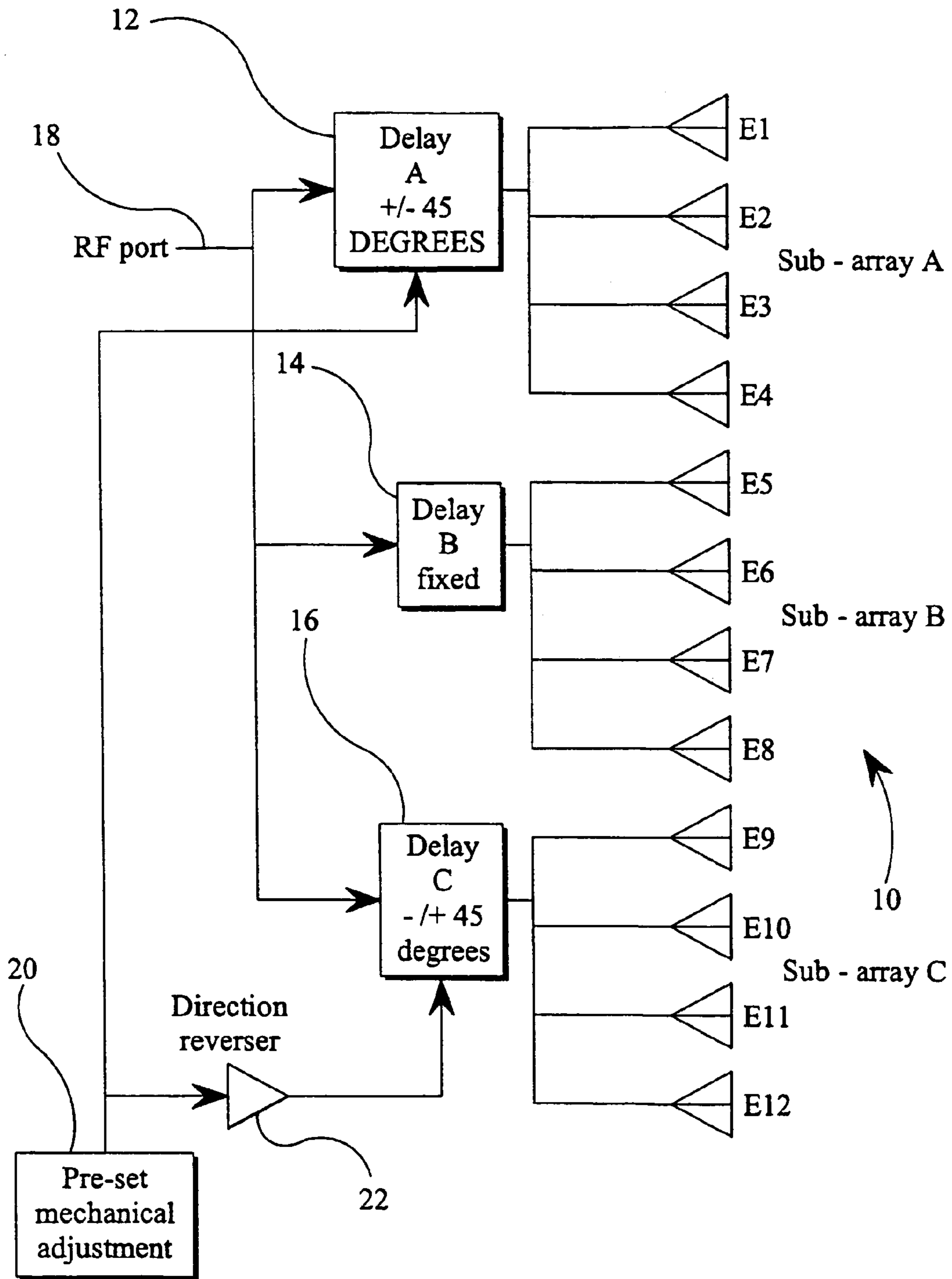
FIG 2 (PRIOR ART)
