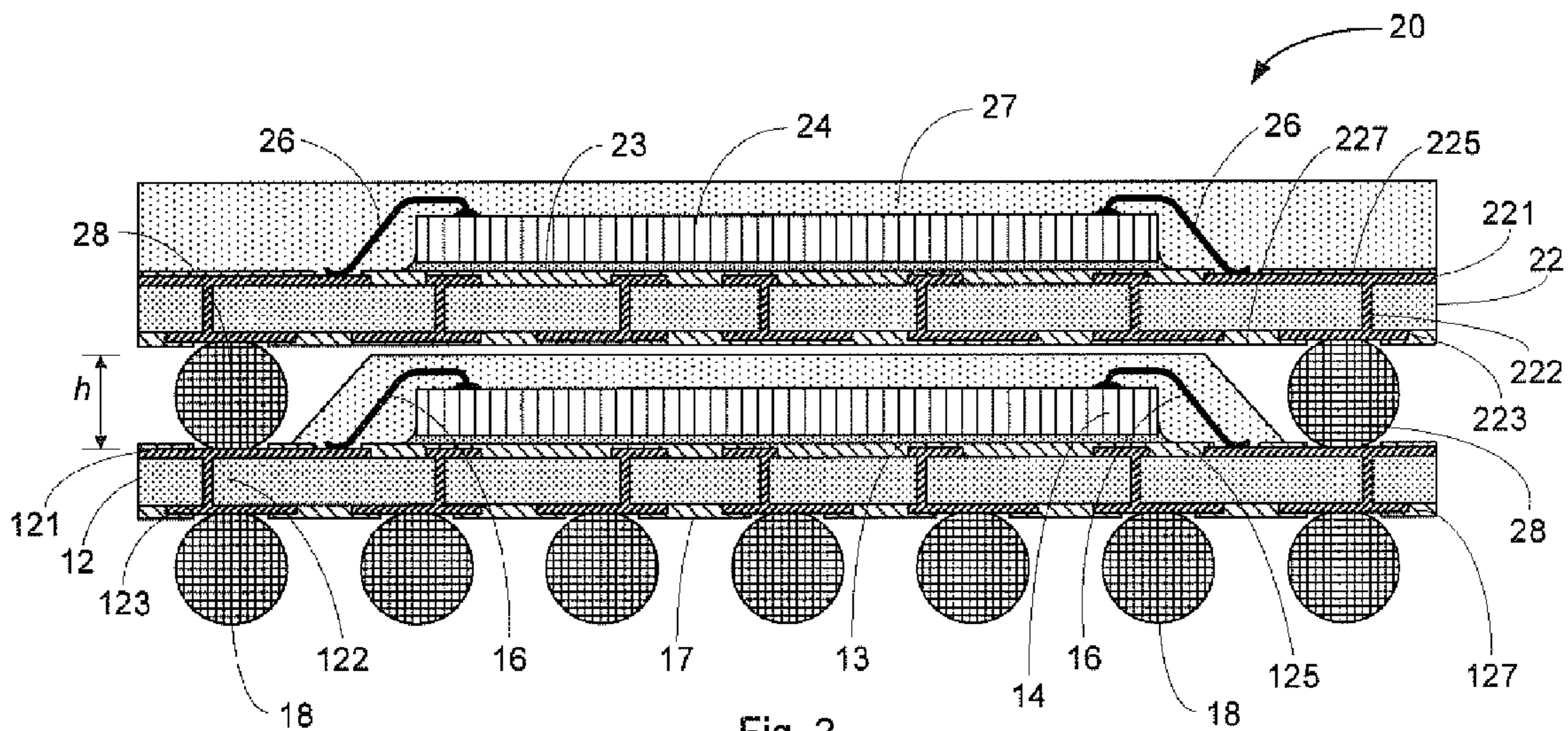
Fig. 2 PRIOR ART
