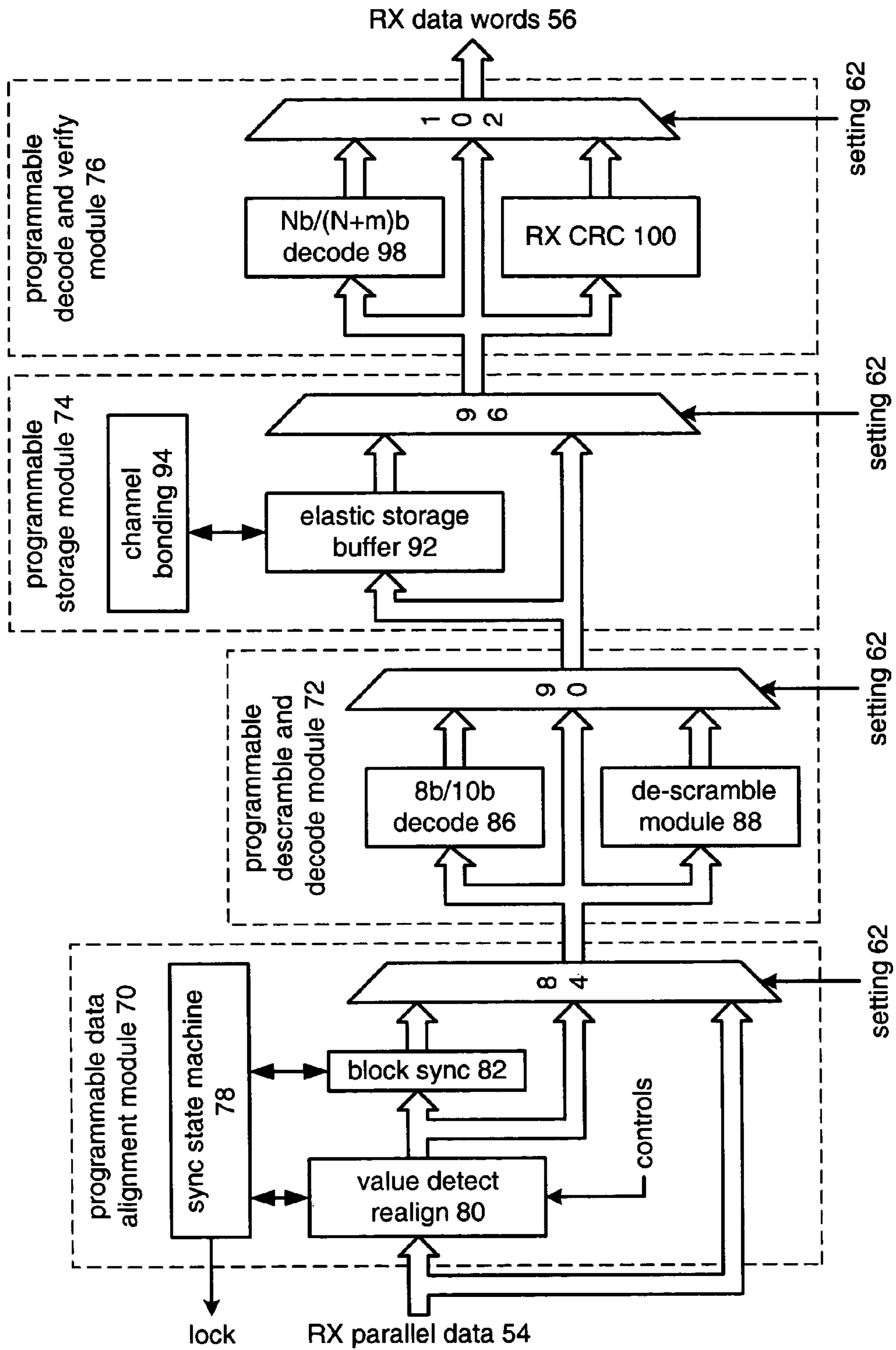
Figure 3 programmable receiver PCS module 44
