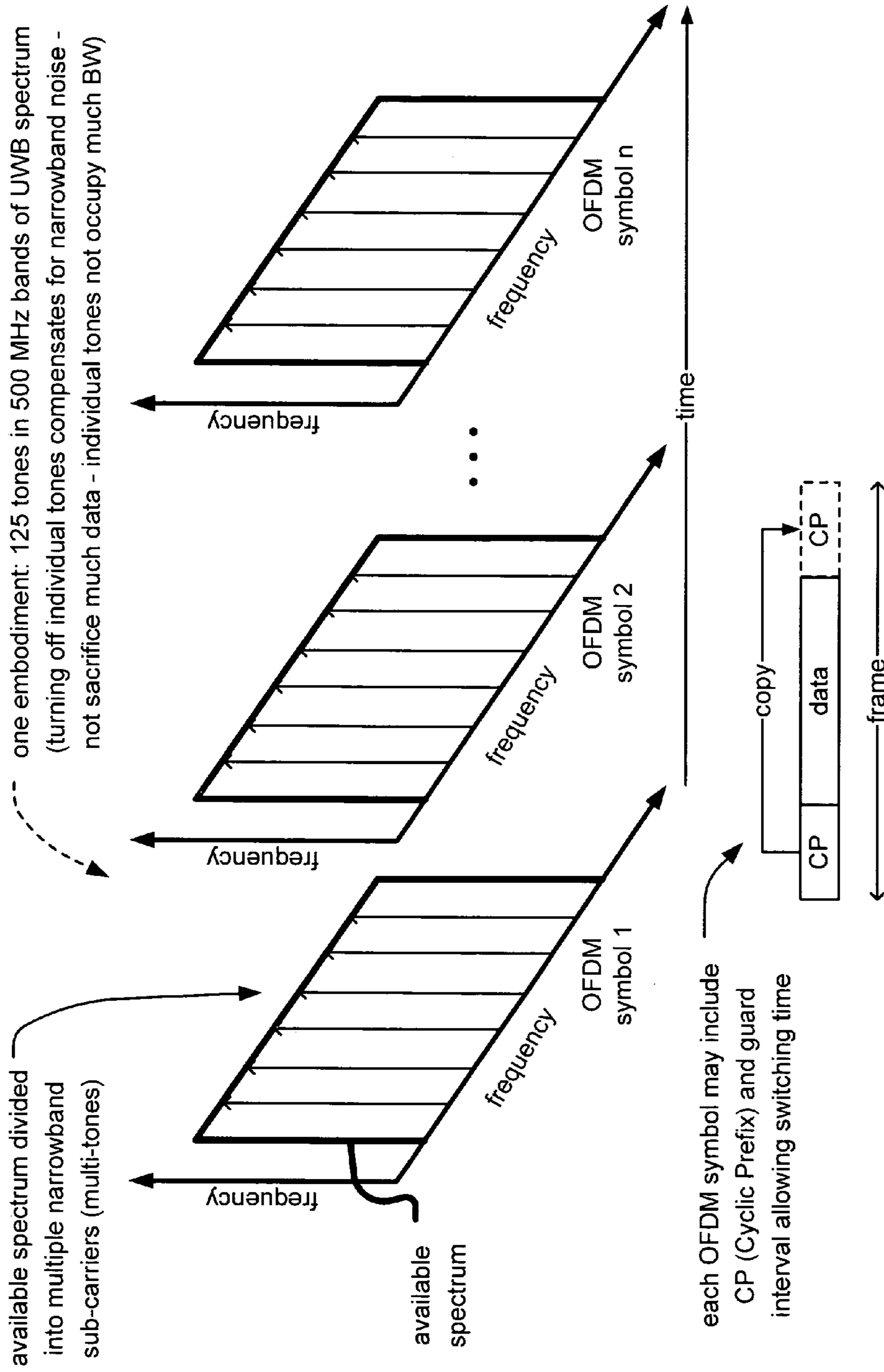
OFDM (Orthogonal Frequency Division Multiplexing) modulation
