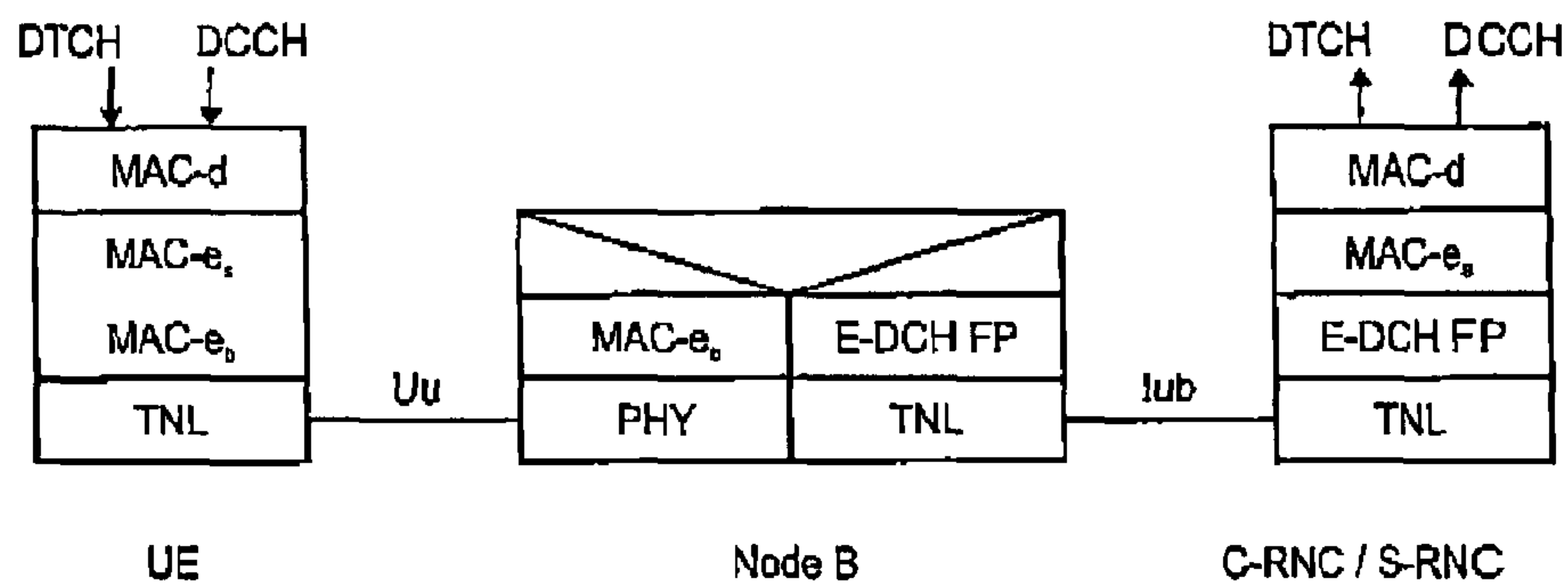
Fig. 9 RELATED ART
