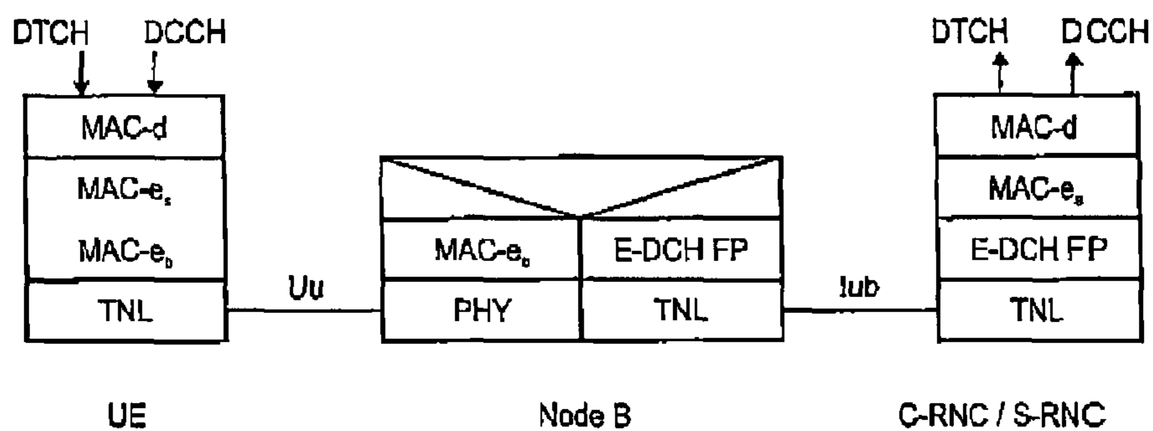
Fig. 9 RELATED ART
