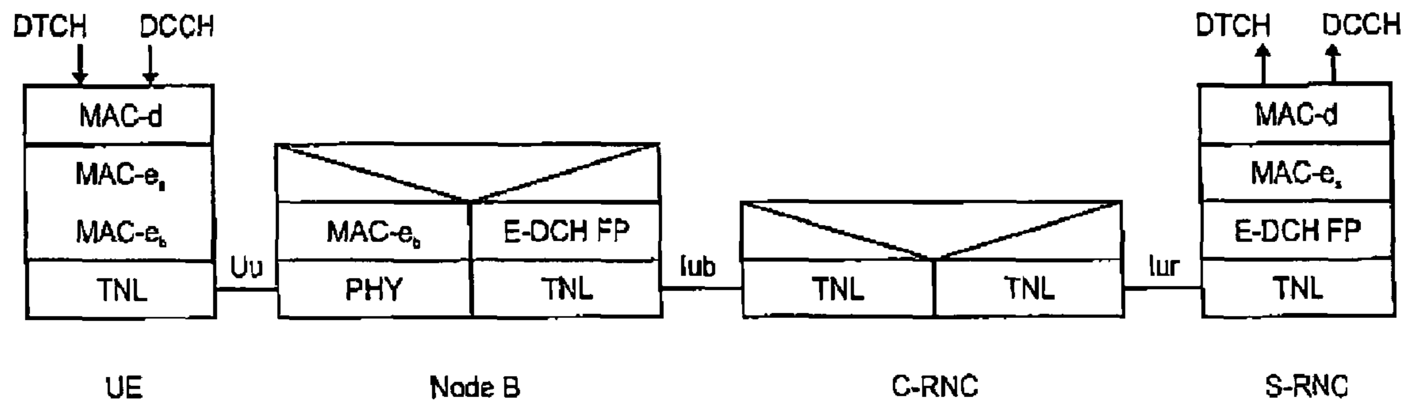
Fig. 10 RELATED ART
