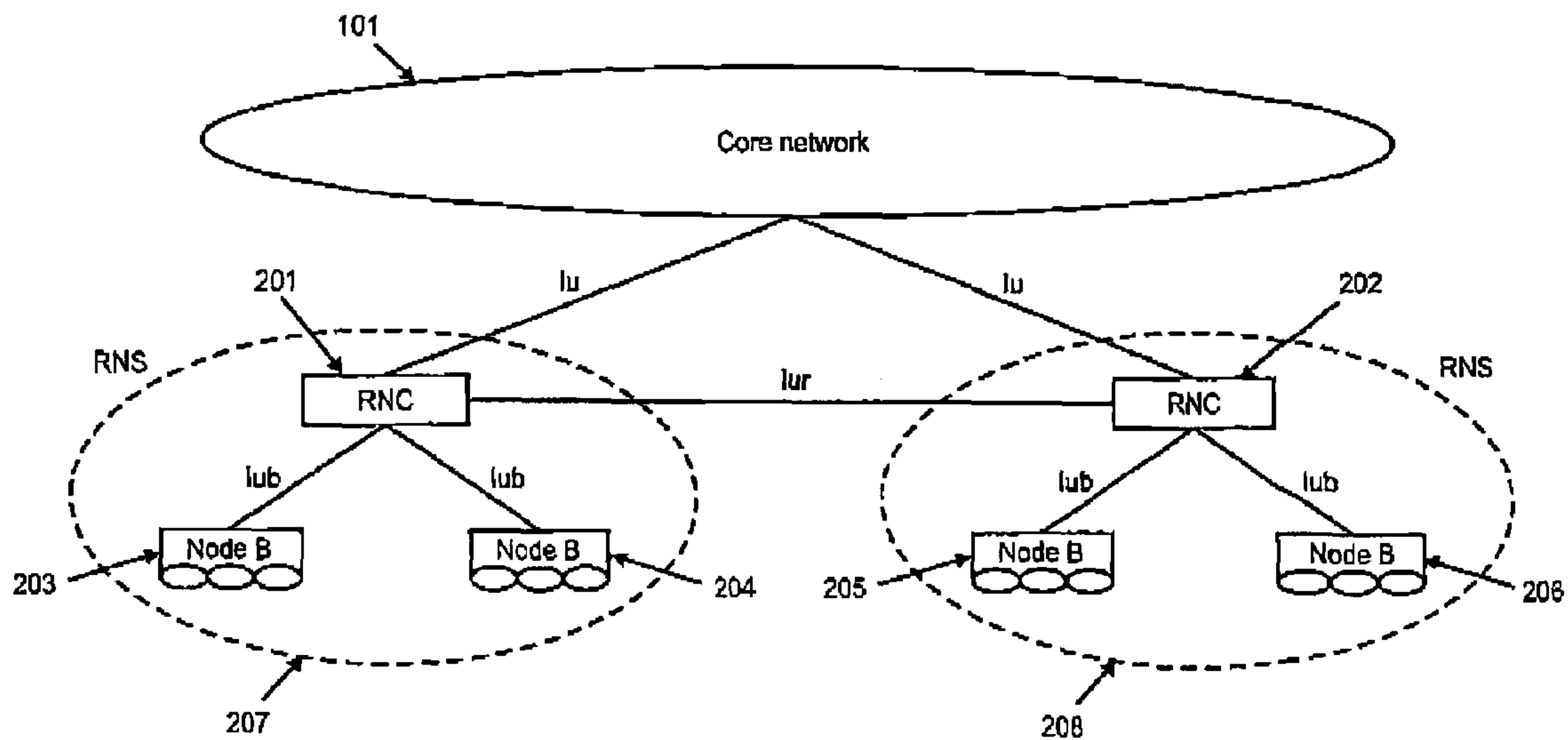
Fig. 2 RELATED ART
