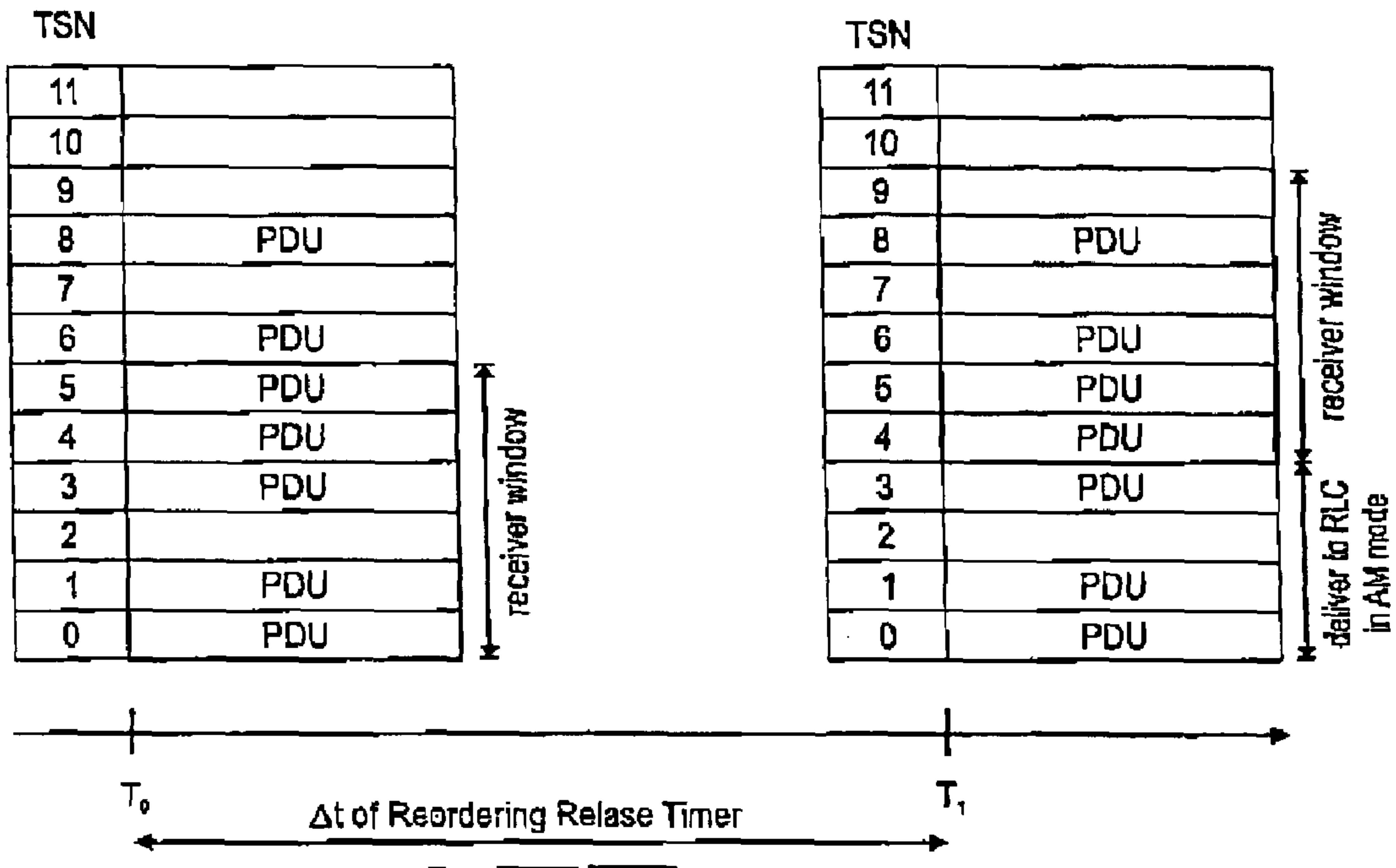
Fig. 8 RELATED ART
