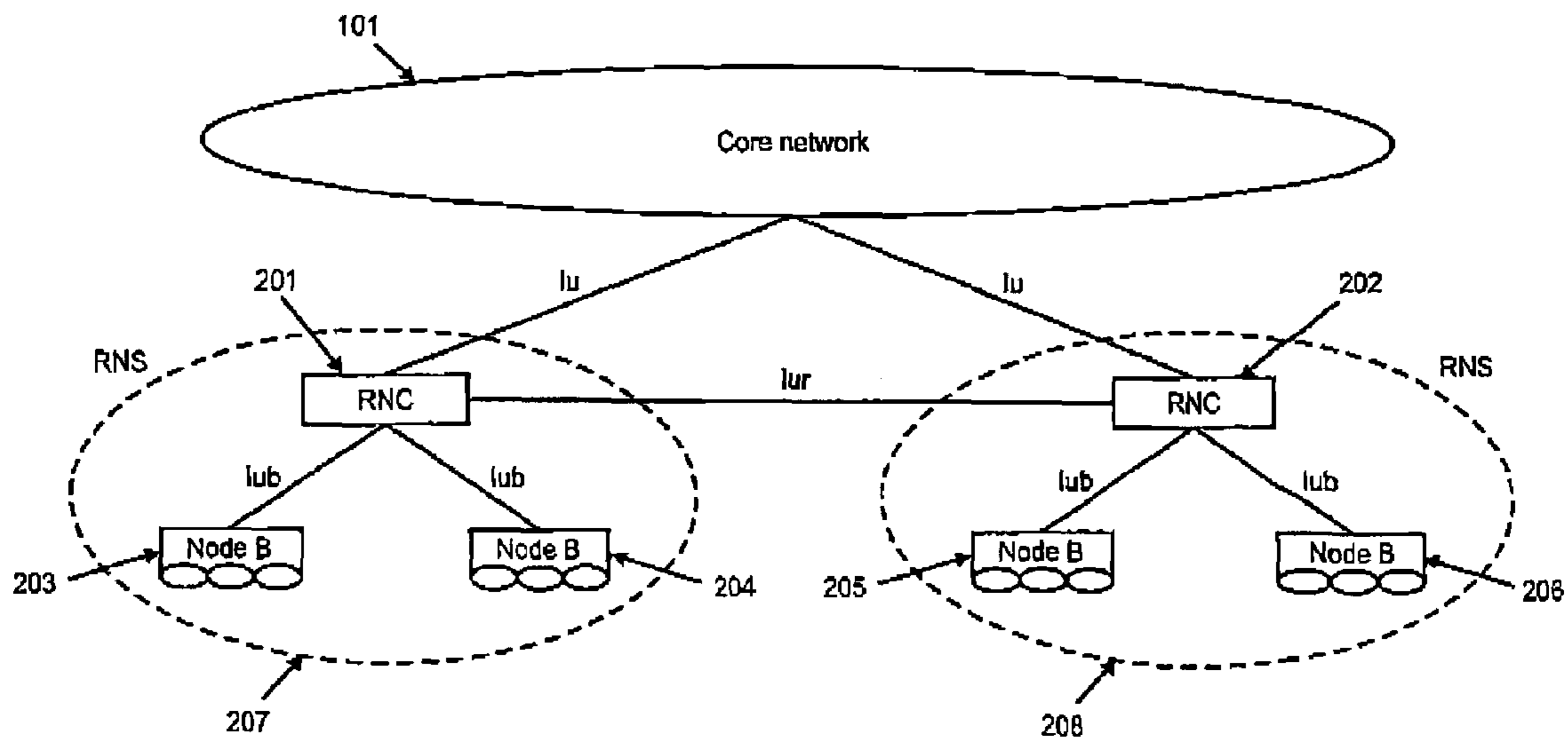
Fig. 2 RELATED ART
