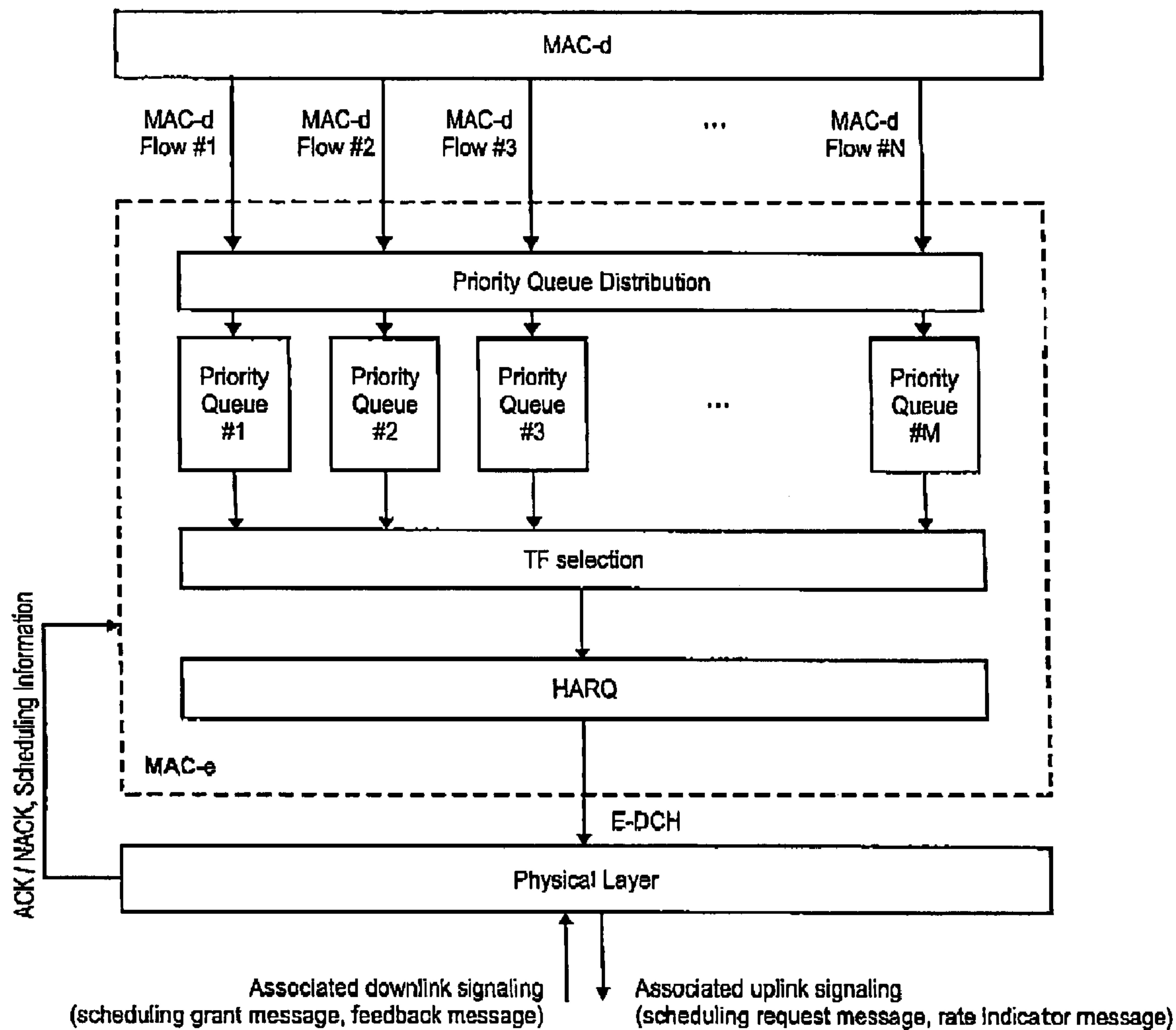
Fig. 4 RELATED ART
