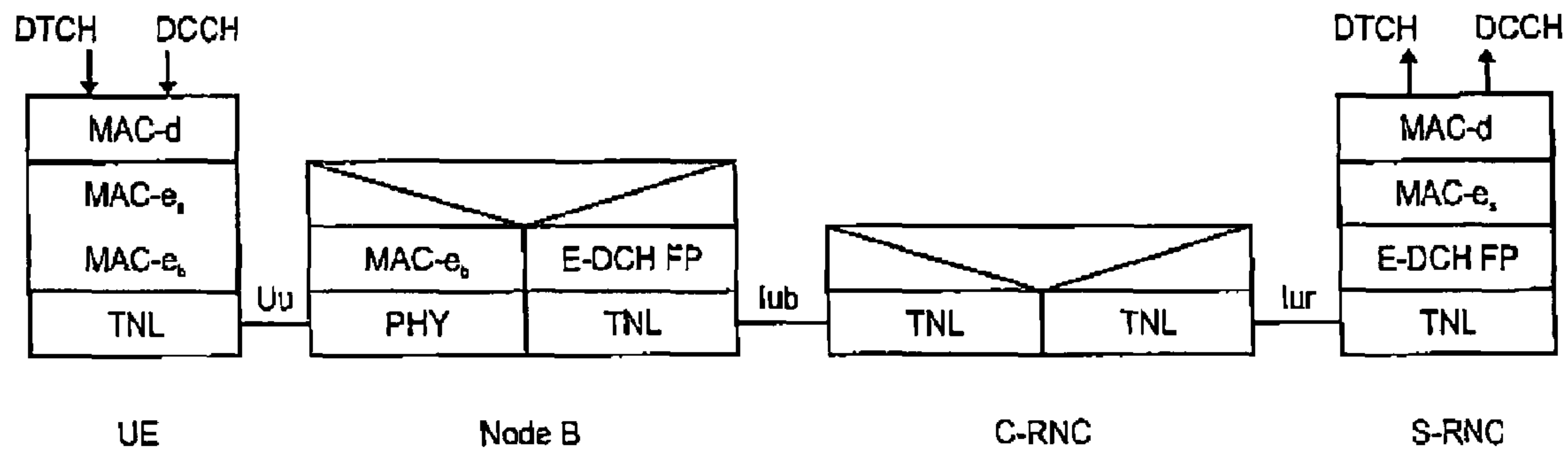
Fig. 10 RELATED ART
