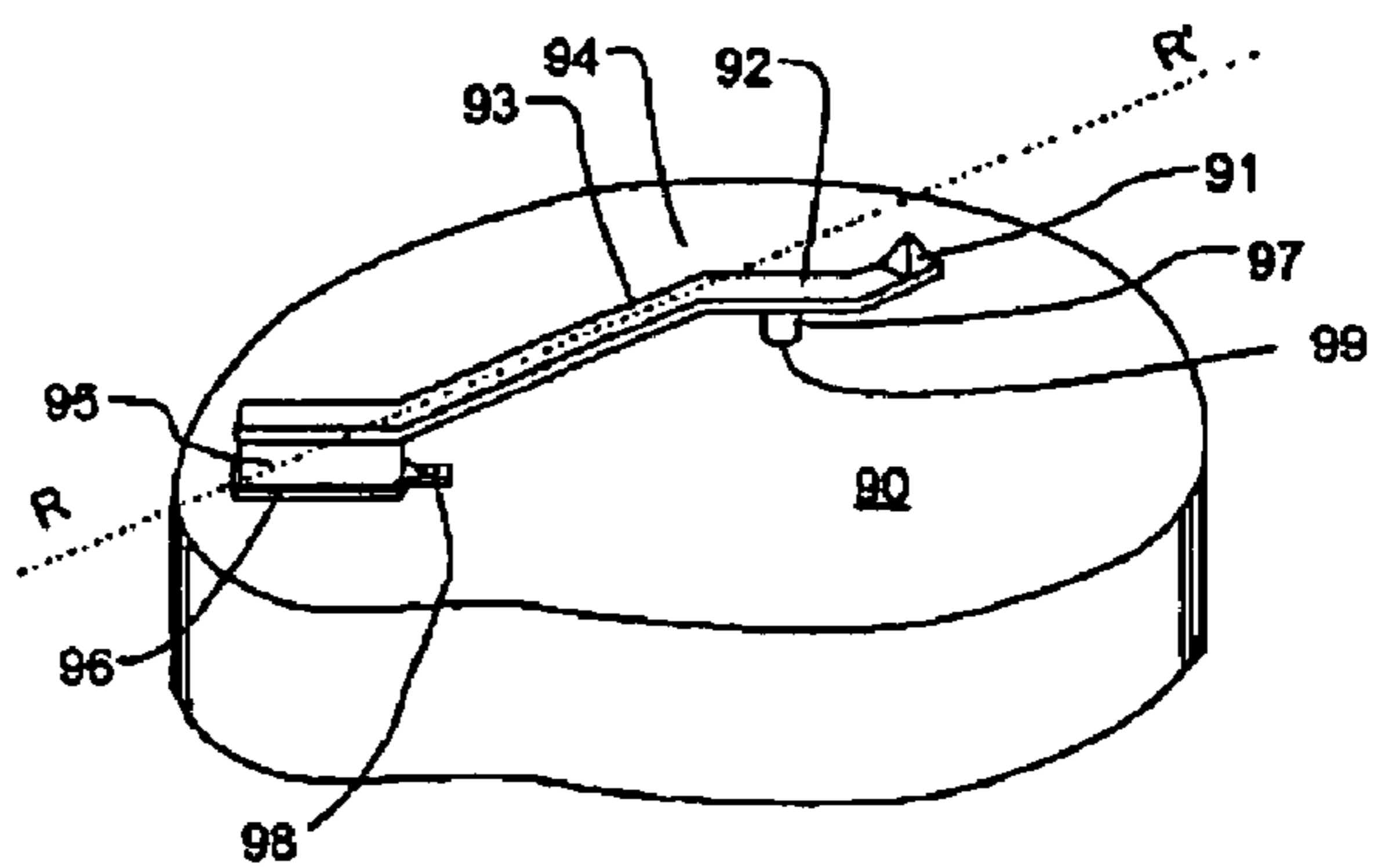
Figure 2B Prior Art
