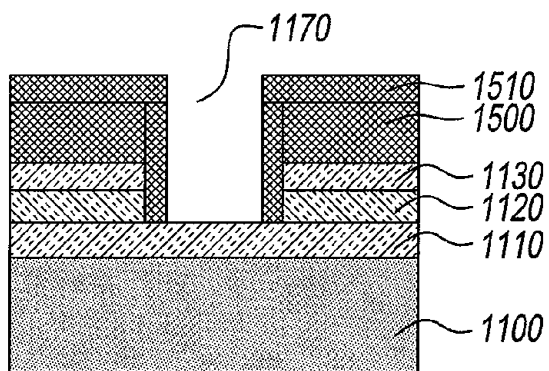
Fig. 1c (Prior Art)
