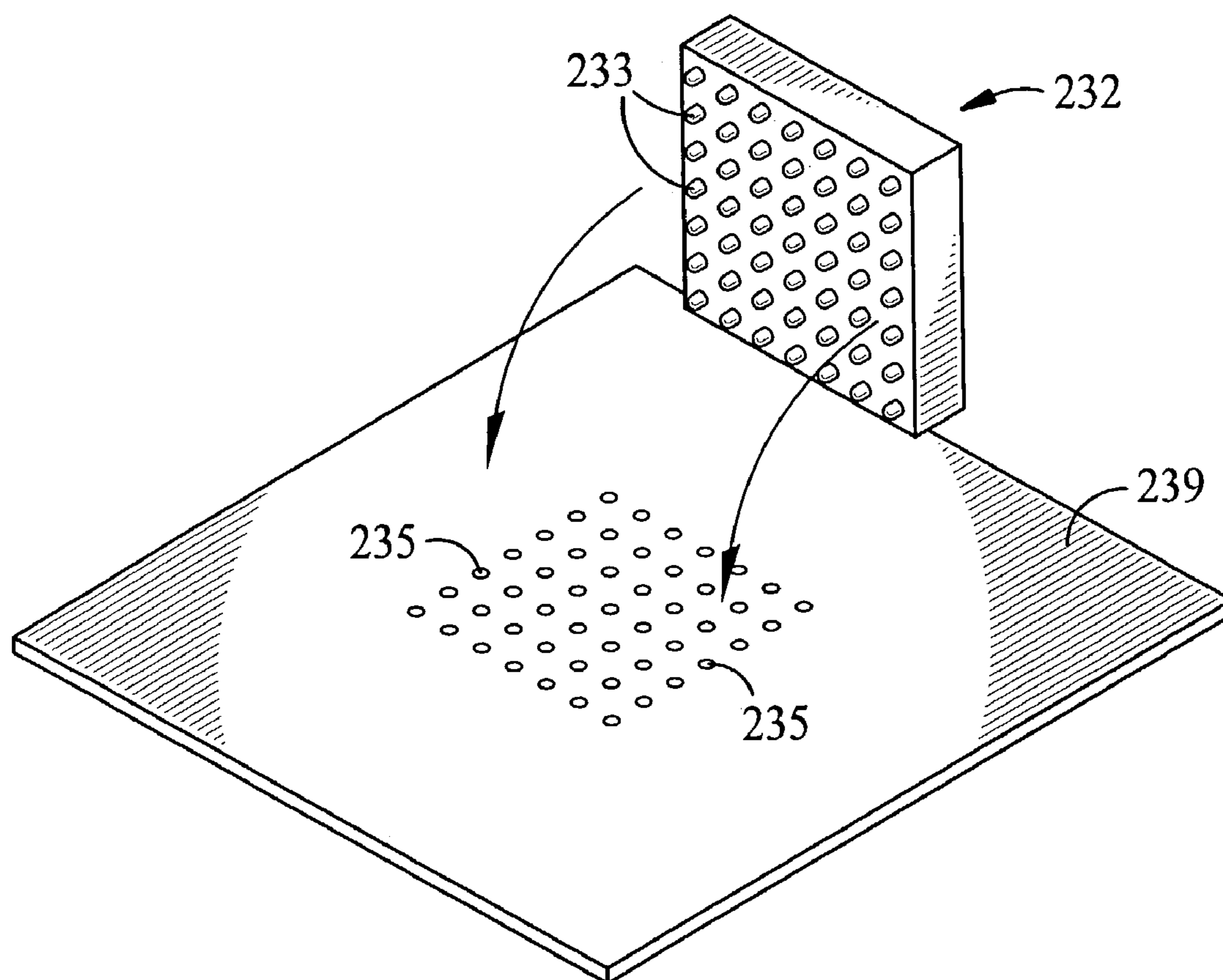
FIG. 13 (Prior Art)
