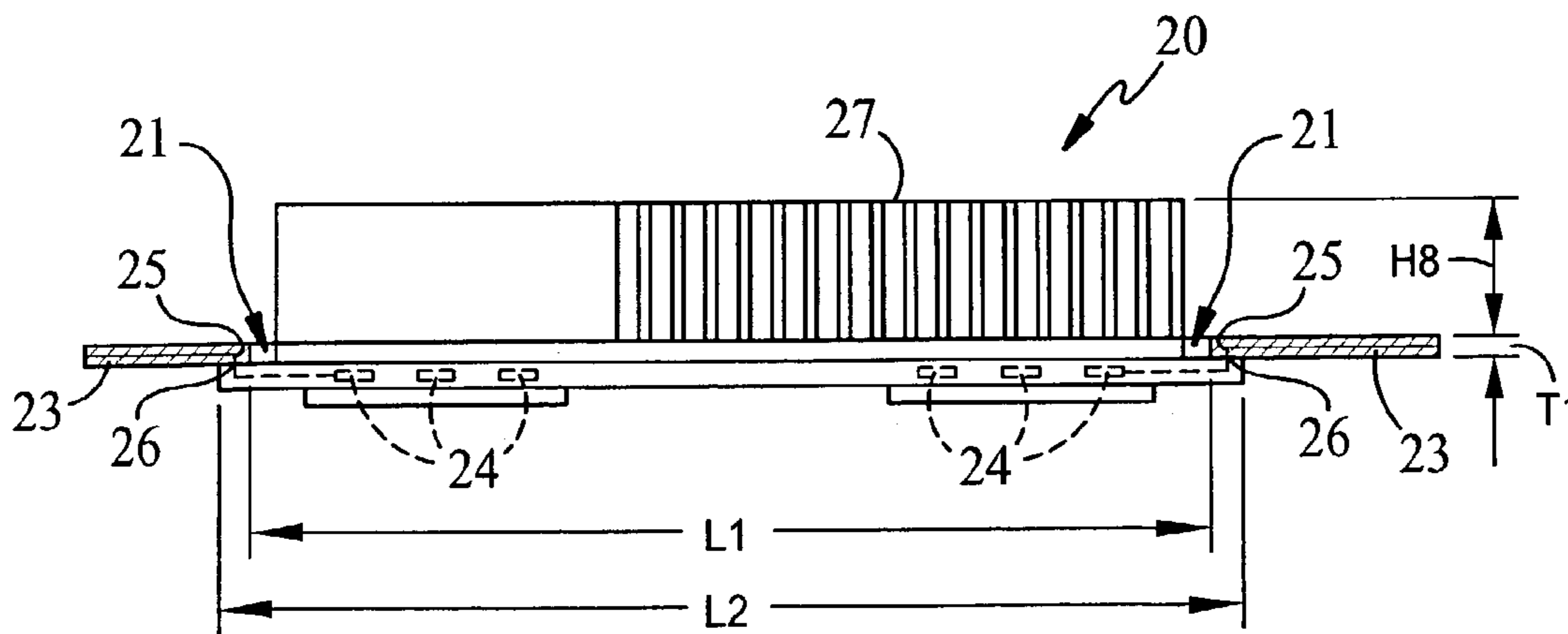
FIG. 2C (Prior Art)
