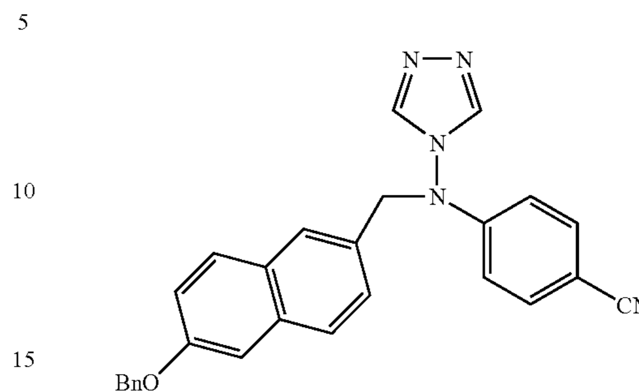
4-[(6-Benzyloxy-naphthalen-2-ylmethyl)-[1,2,4]triazol-4-yl-amino]-benzonitrile (JRL01010)
