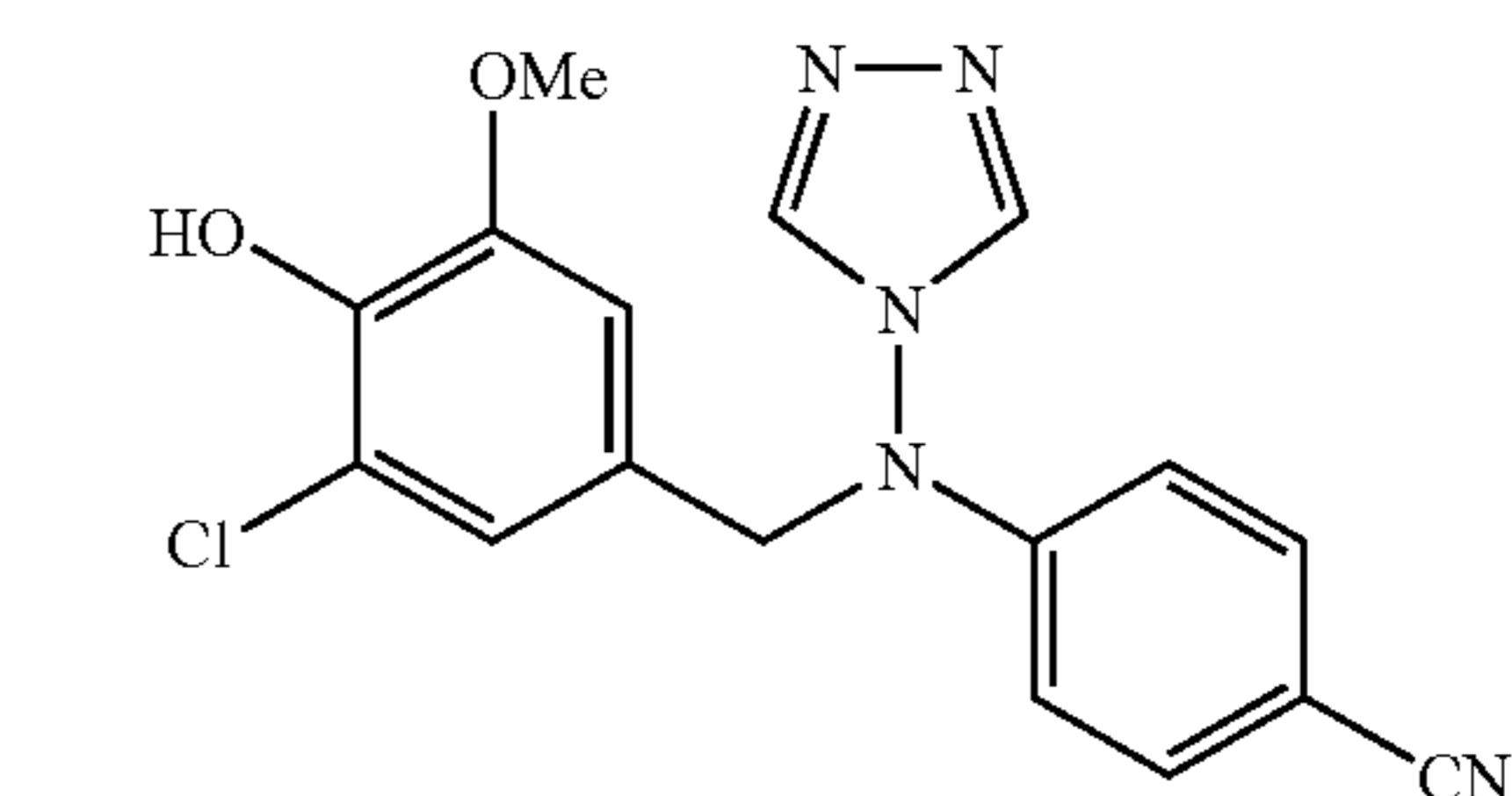
4-[(3-chloro-4-hydroxy-5-methoxy-benzyl)-[1,2,4]triazol-4-yl-amino]-benzotrile (CAB02179, STX600)
