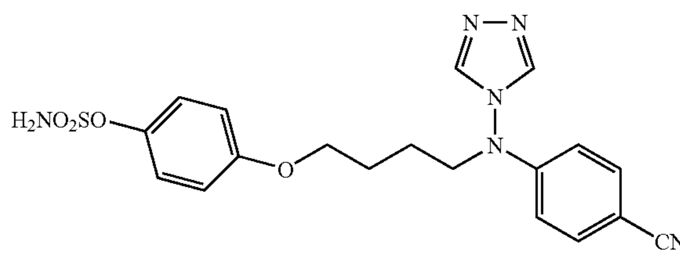
Sulfamic acid 4-[[4-(4-cyanophenyl)-[1,2,4]triazol-4-ylamino]buto]phenyl ester (LWO02068, STX288)
