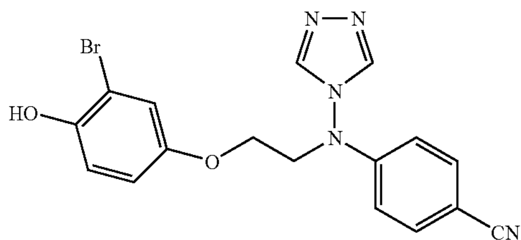
4-{[2-(3-Bromo-4-hydroxyphenoxy)ethyl]-[1,2,4]triazol-4-ylamino}benzonitrile (STX300)
