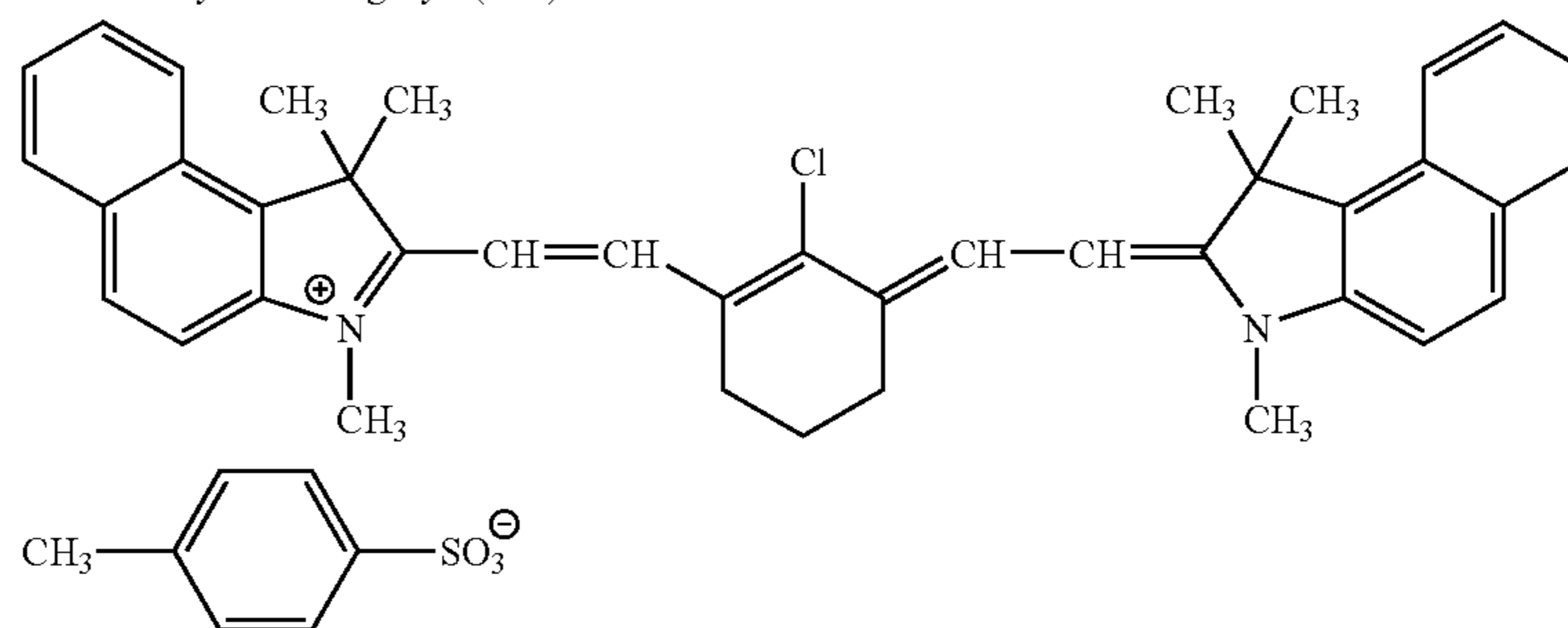
Infrared ray-absorbing dye (D-2)
