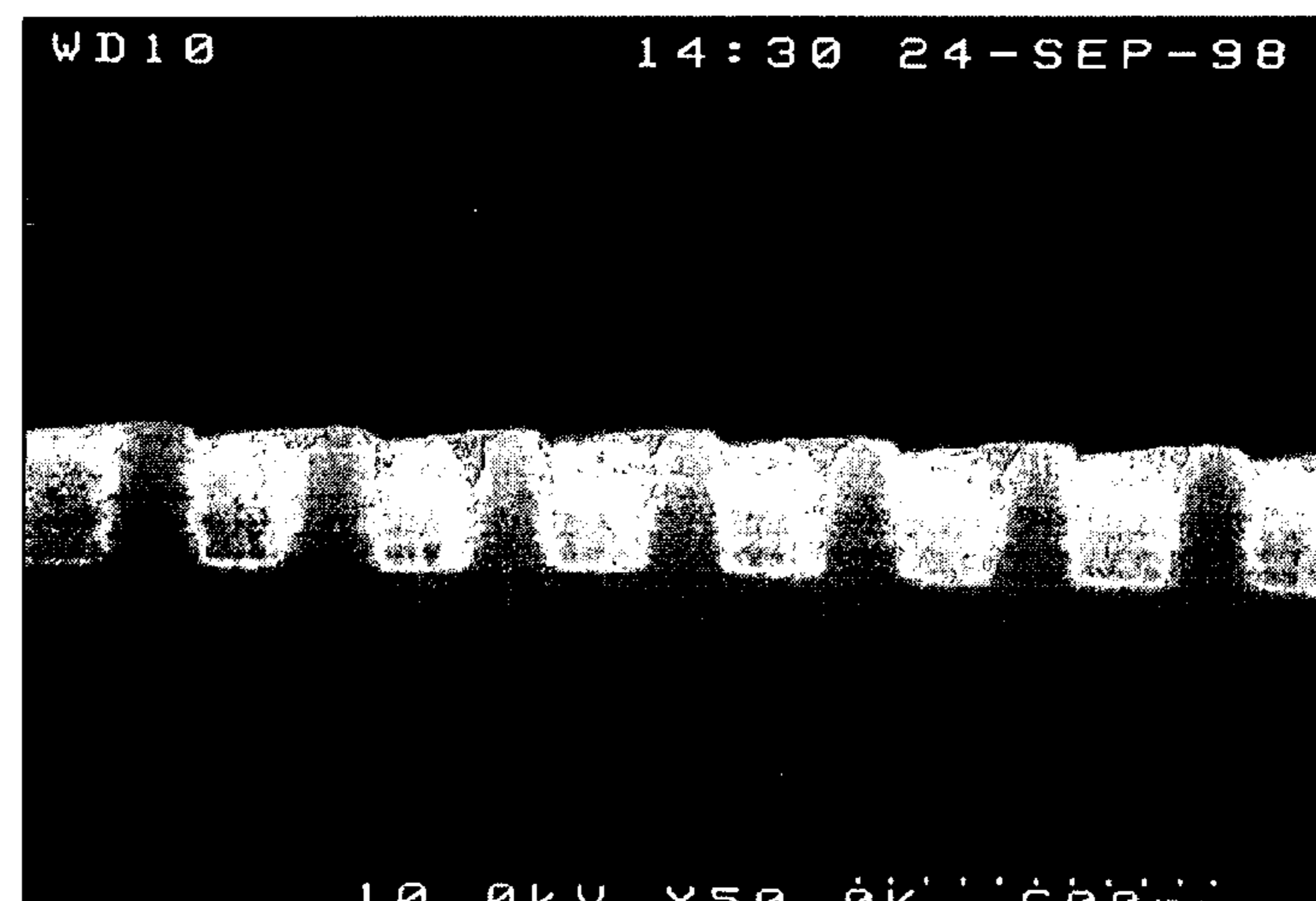
novolak underlayer with k=0.08 at 248nm
