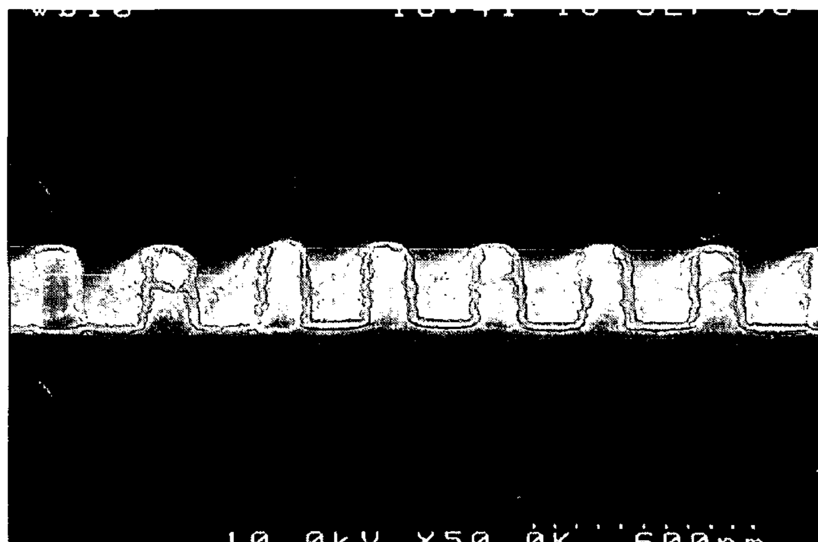
novolak underlayer with k=0.20 at 248nm
