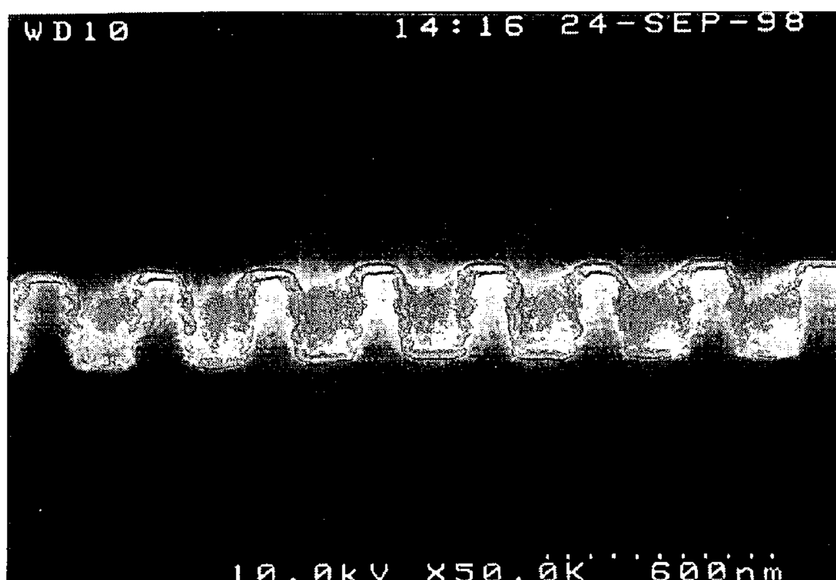
novolak underlayer with k=0.35 at 248nm
