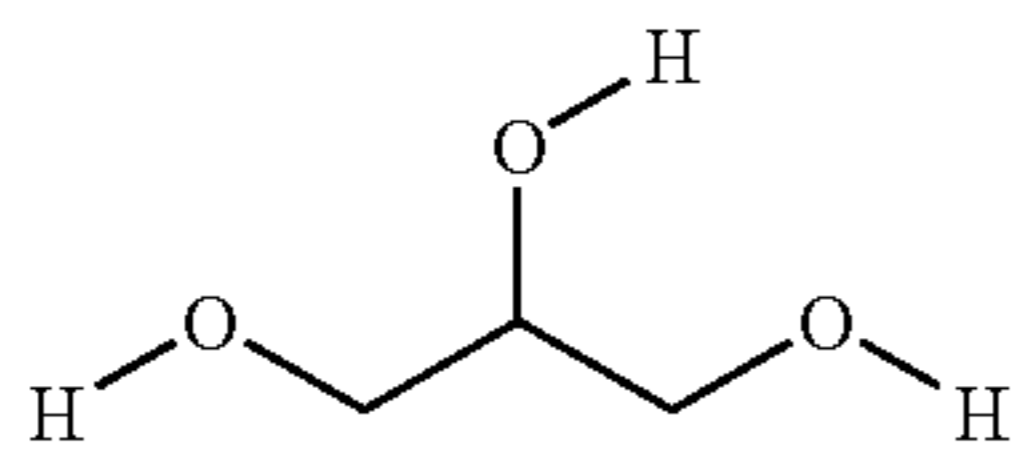
glycerol
