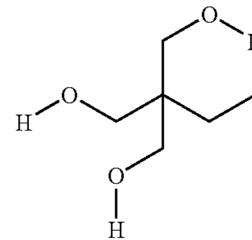
trimethylolpropane
