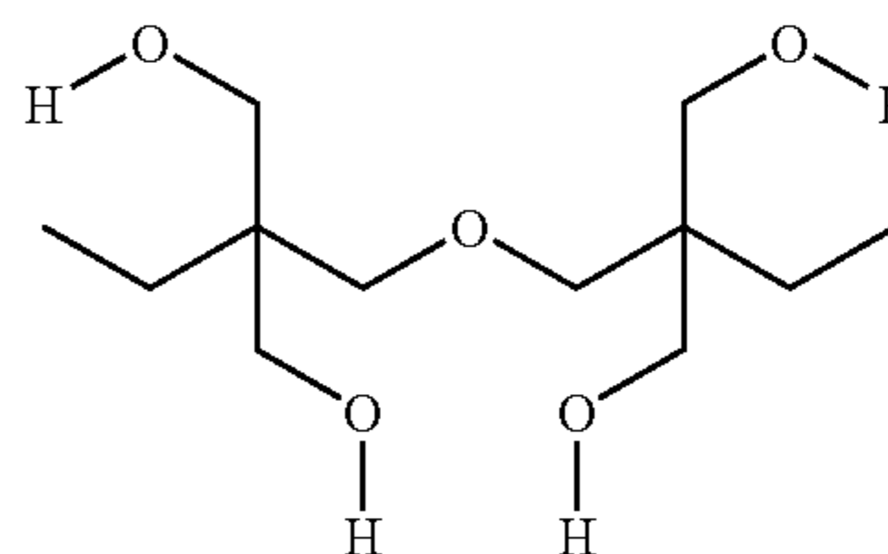
ditrimethylolpropane
