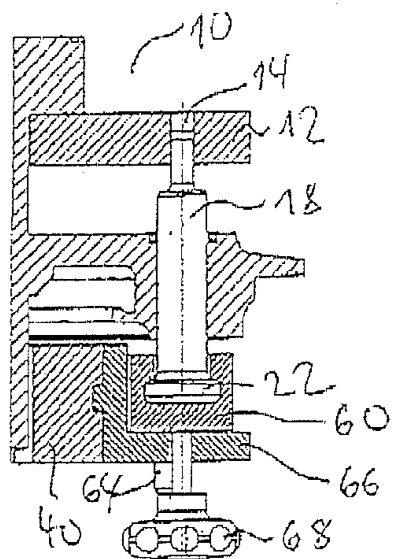
Section D - D
