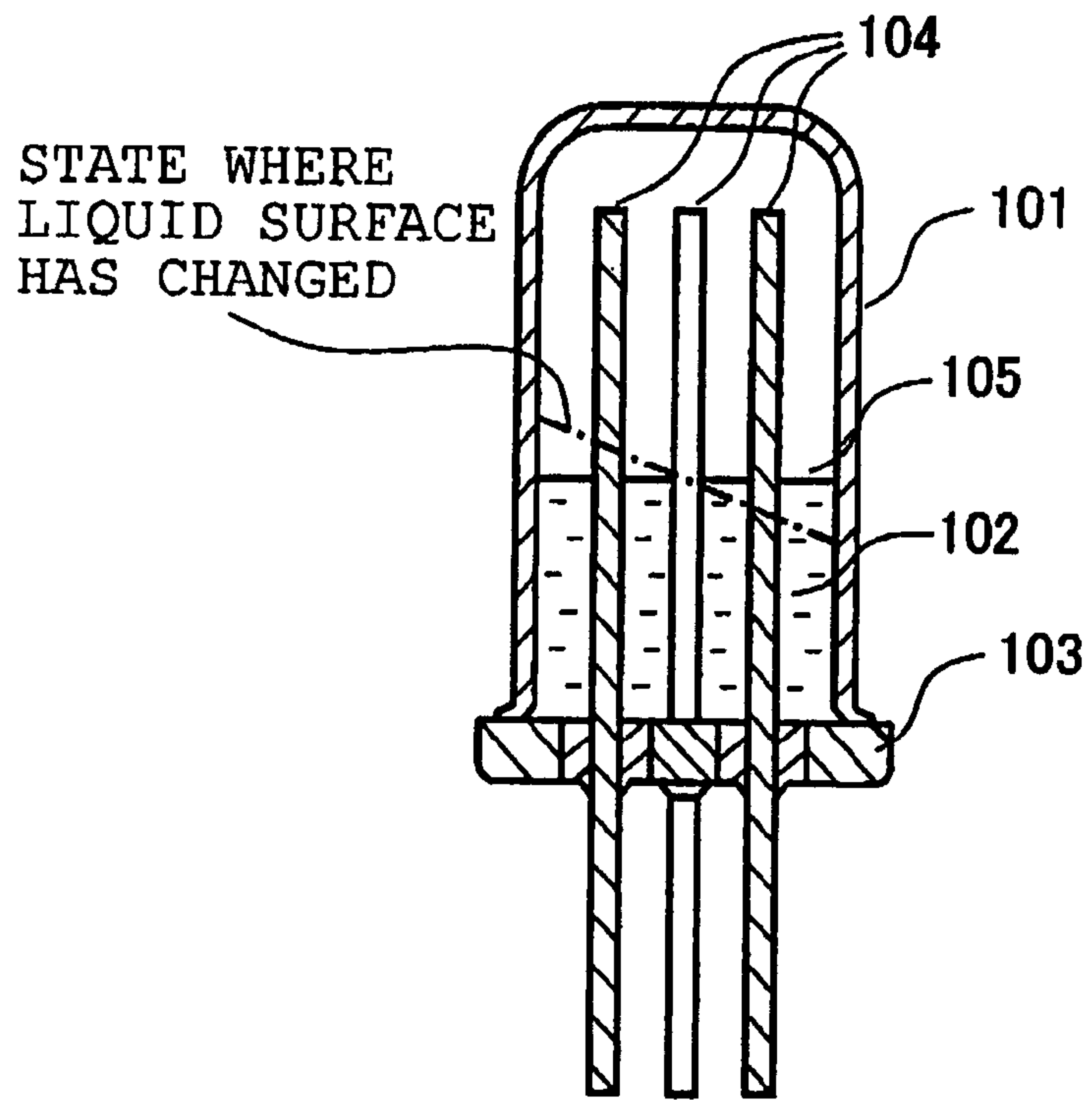
FIG. 20 PRIOR ART
