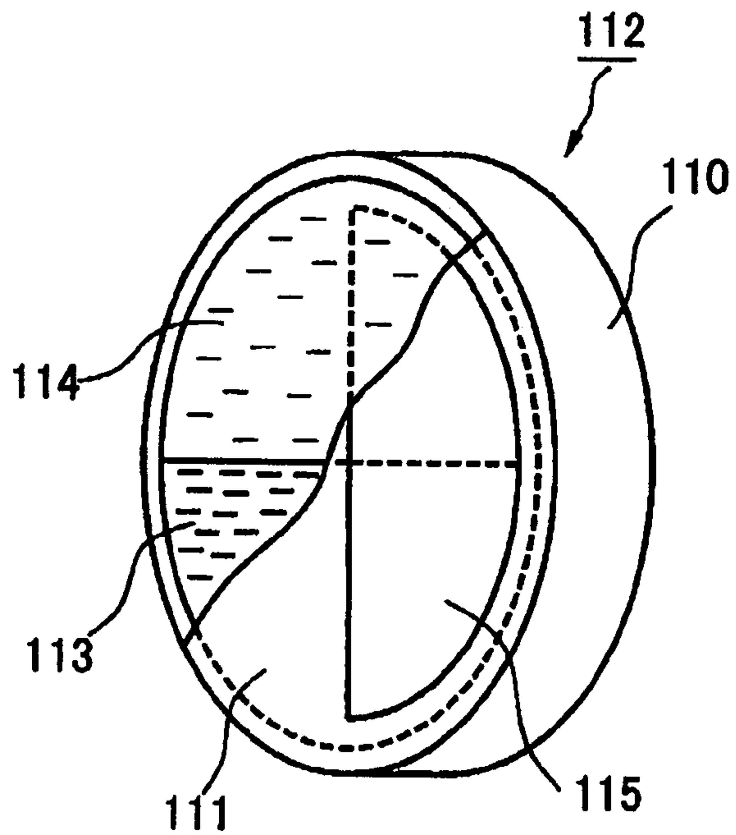
FIG. 21 PRIOR ART
