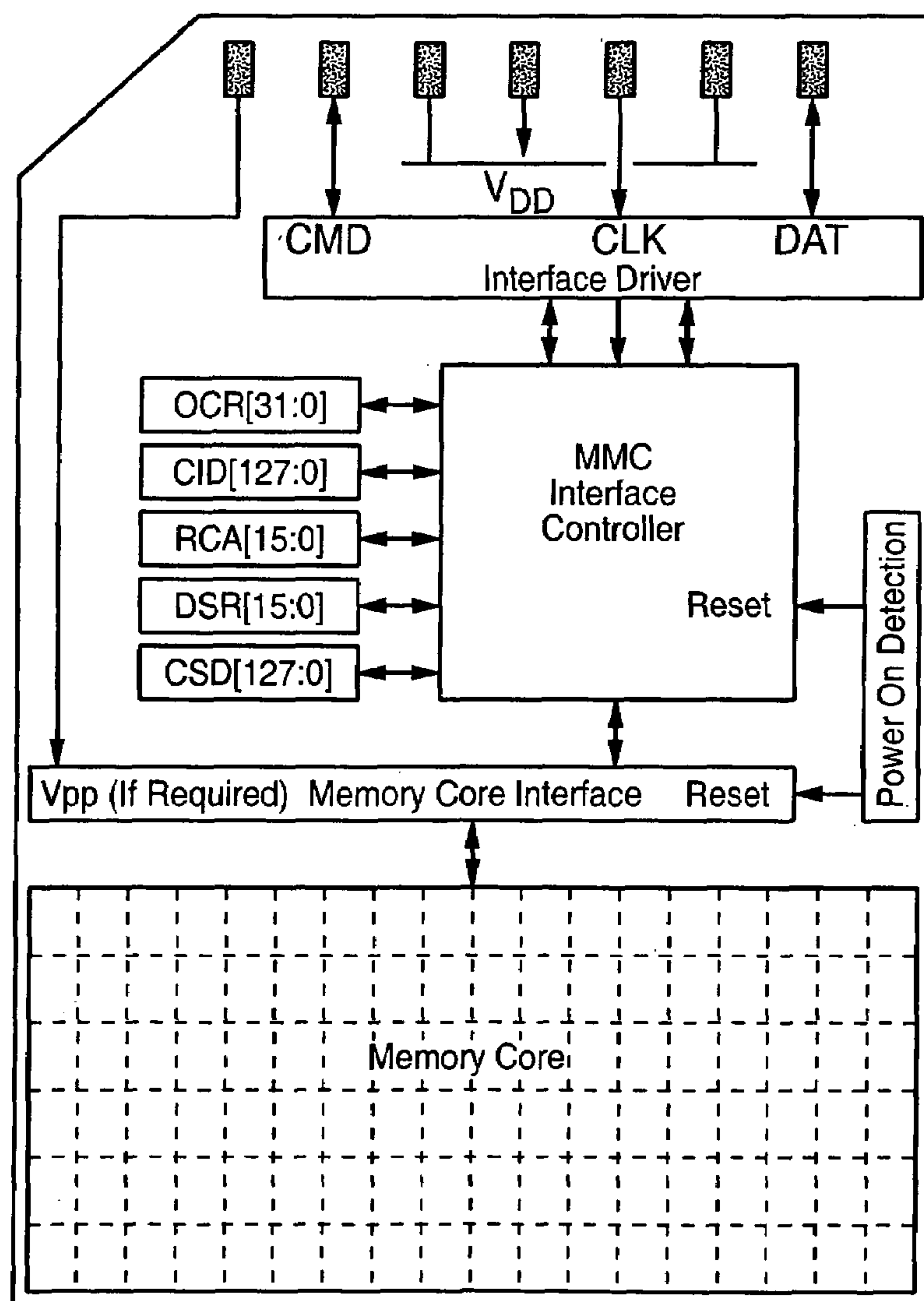
FIG. 2 (PRIOR ART)
