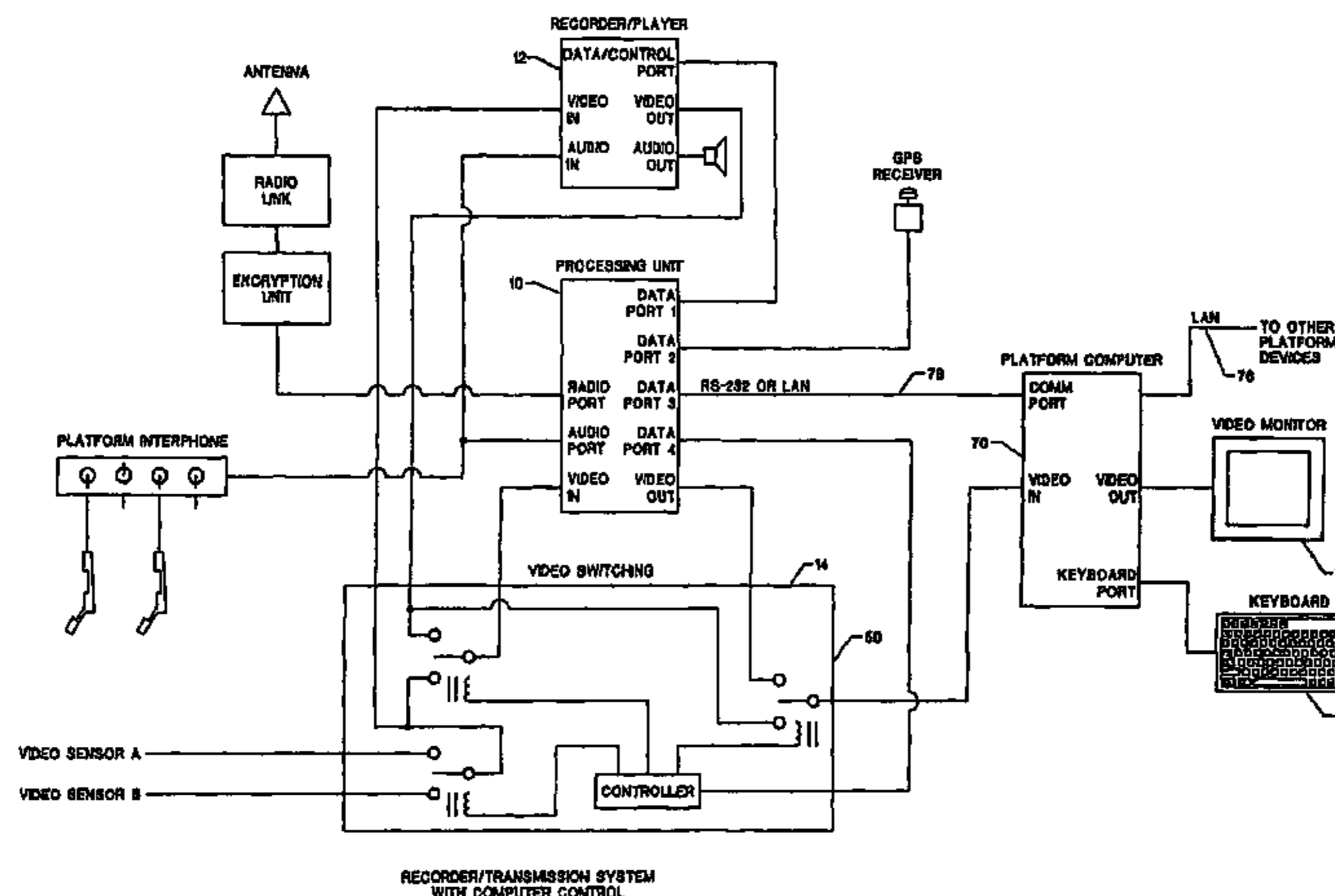
RECORDER/TRANSMISSION SYSTEM WITH COMPUTER CONTROL
