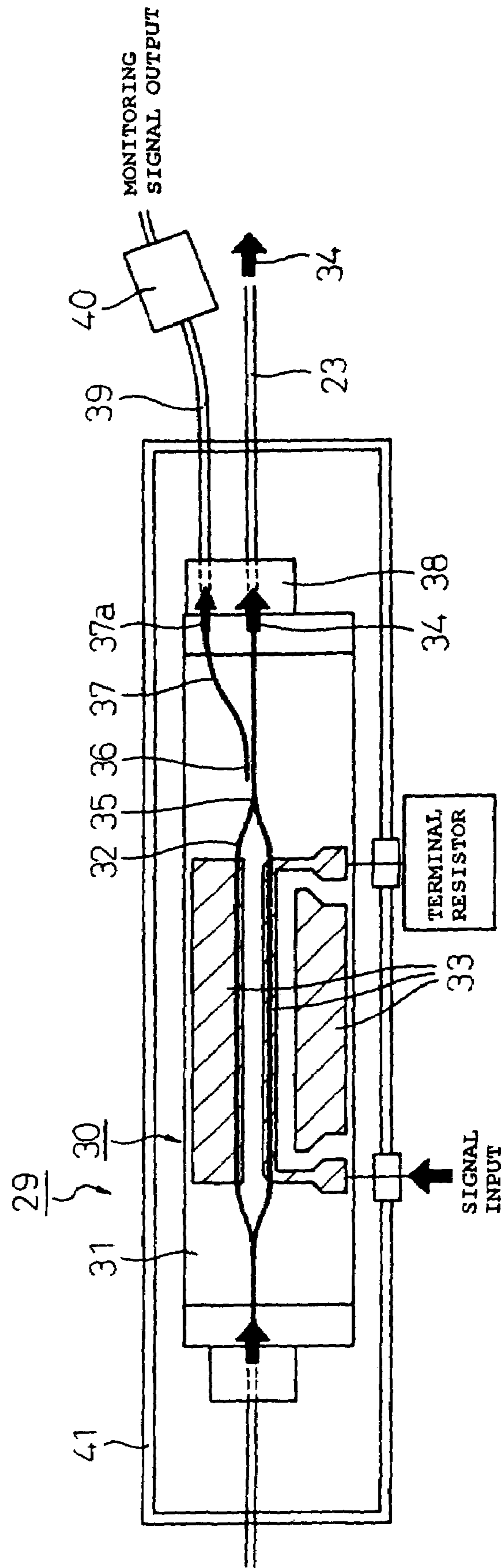
Fig.3 PRIOR ART
