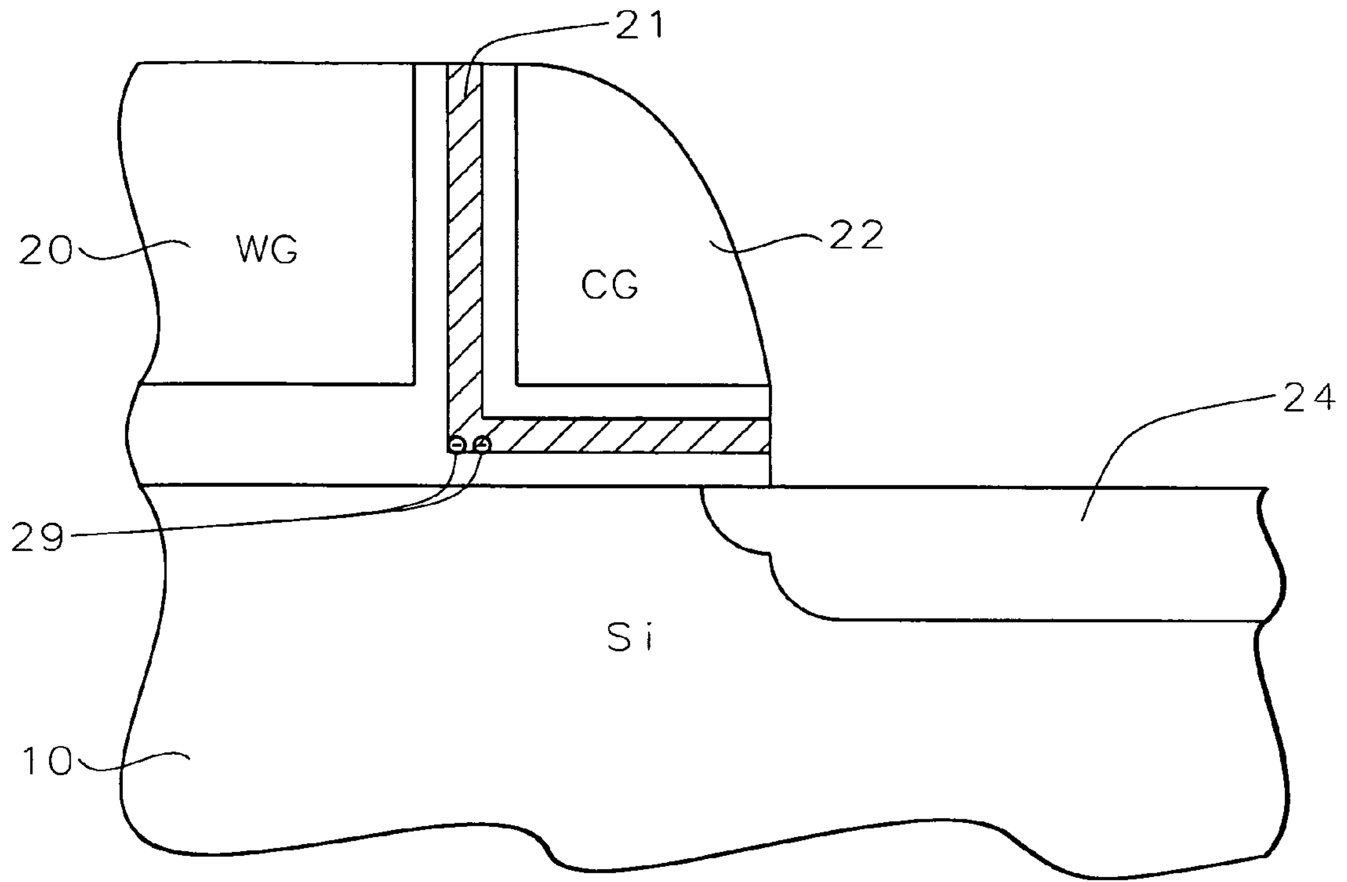
FIG. 4 Prior Art
