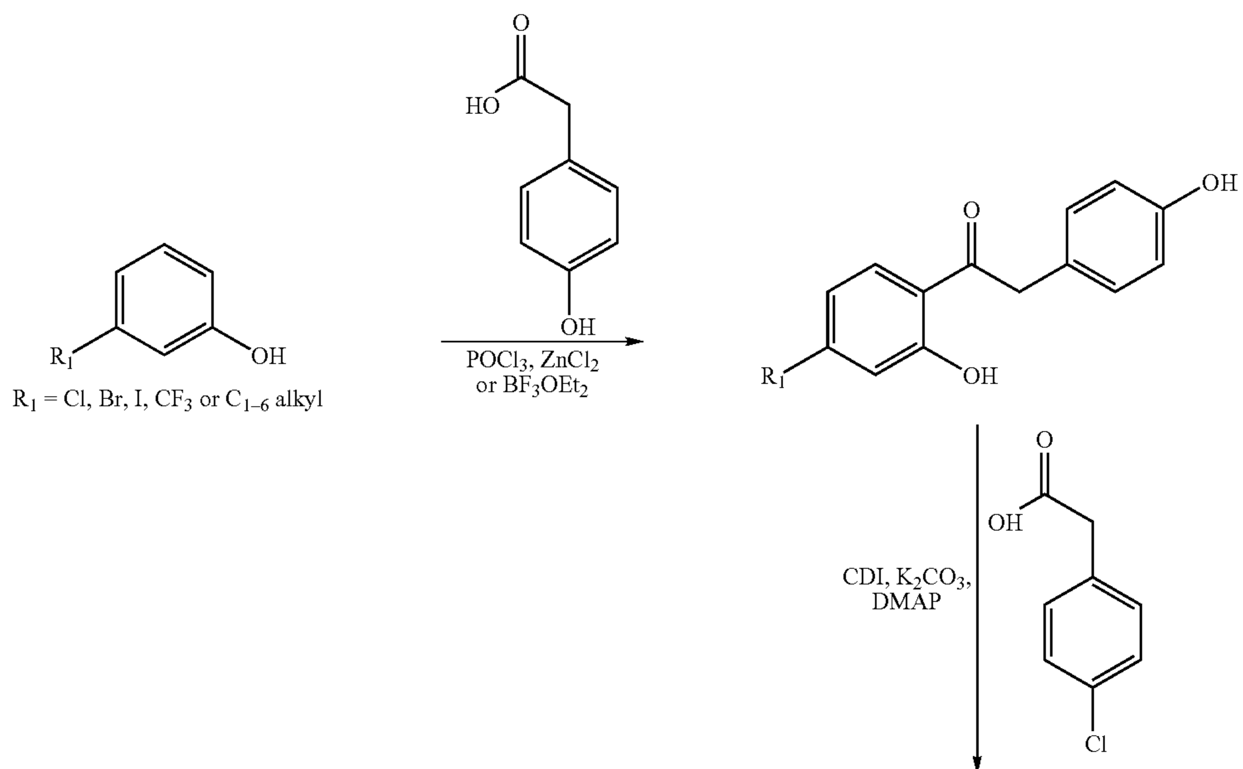
Reaction Scheme 2
