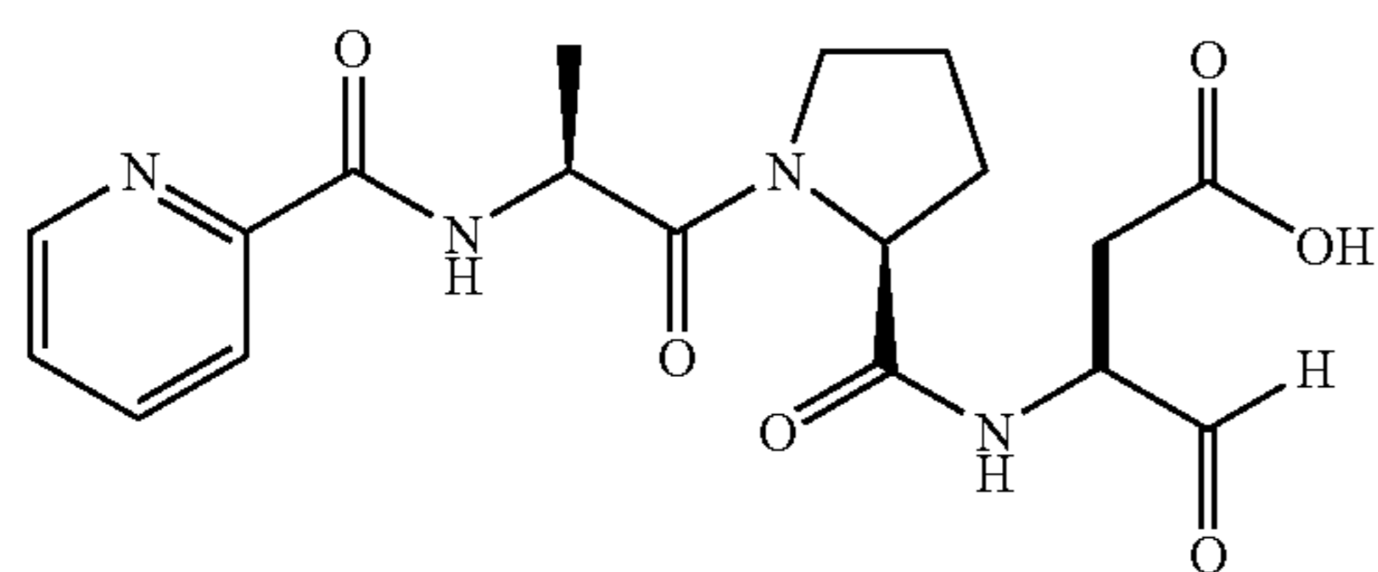
4-Oxo-3-[(1-{2-[pyridine-2-carbonyl]-amino]-propionyl}-pyrrolidine-2-carbonyl)-amino]-butyric acid (122e)
