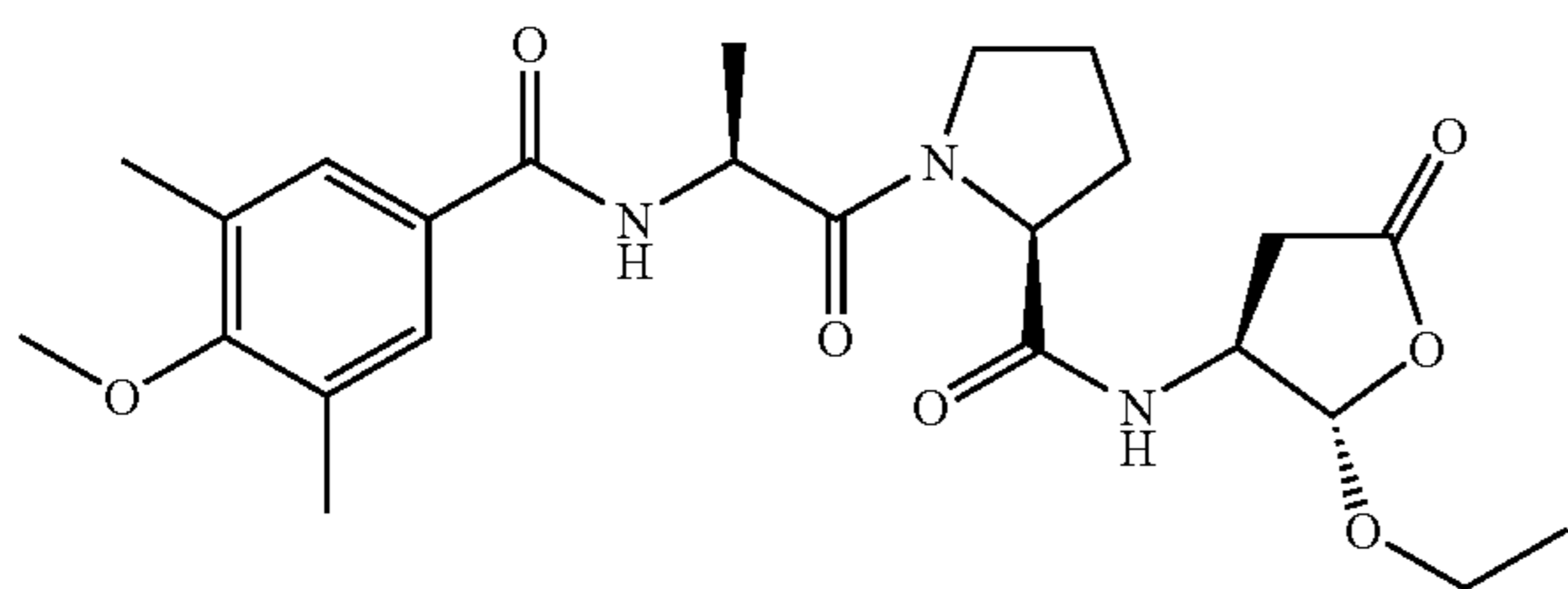
1-[2-(4-Methoxy-3,5-dimethyl-benzoylamino)-propionyl]-pyrrolidine-2-carboxylic acid (2-ethoxy-5-oxo-tetrahydro-furan-3-yl)-amide (98af)
