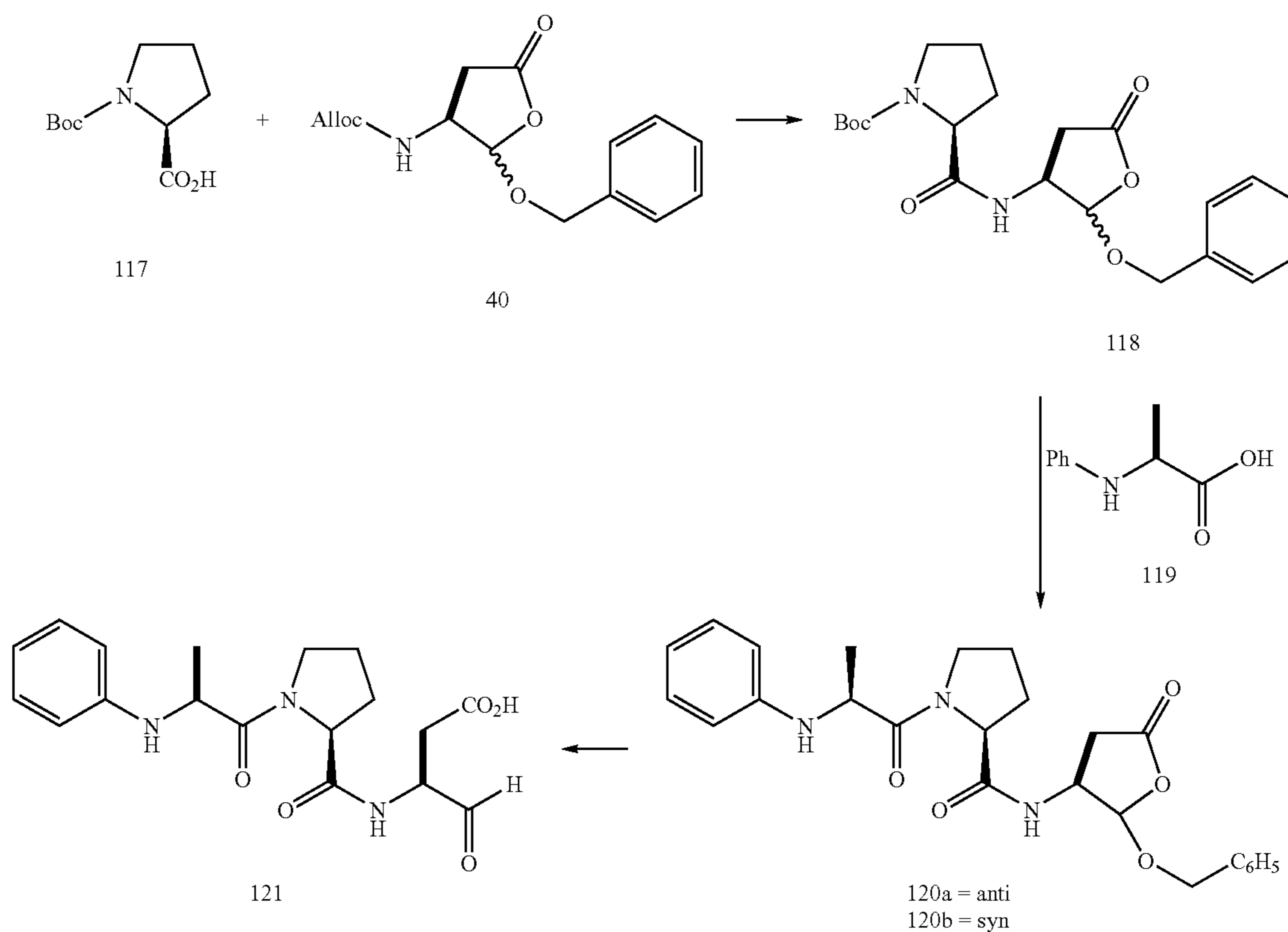
Scheme XXII
