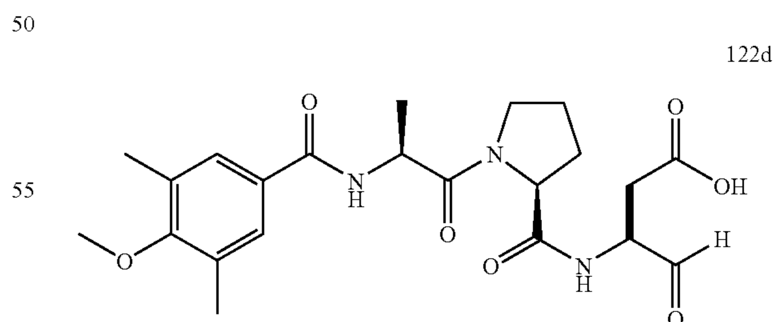
3-({1-[2-(4-Methoxy-3,5-dimethyl-benzoylamino)-propionyl]-pyrrolidine-2-carbonyl}-amino)-4-oxo-butanoic acid (122d)
