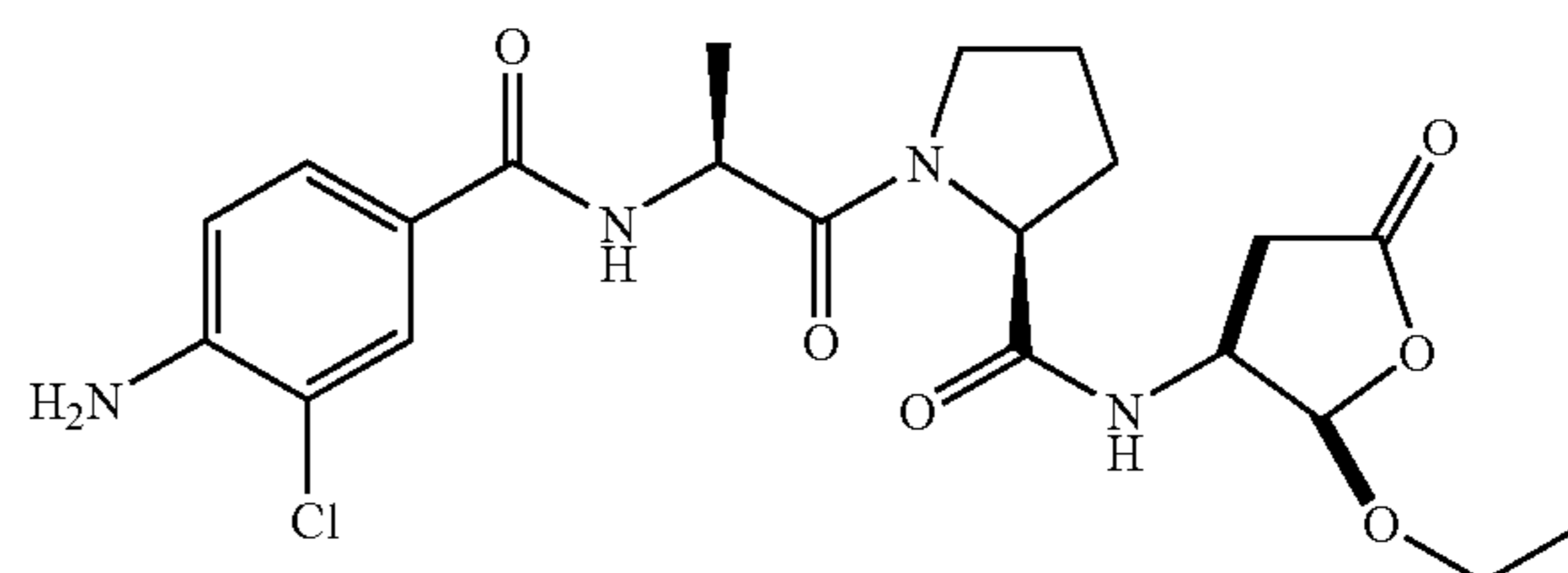
2-(Ethoxy-5-oxo-tetrahydro-furan-3-yl)-carbamic acid allyl ester
