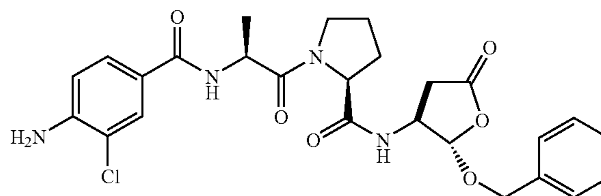
1-[2-(4-Amino-3-chloro-benzoylamino)-propionyl]-pyrrolidine-2-carboxylic acid (2-benzyloxy-5-oxo-tetrahydro-furan-3-yl)-amide (98c)
