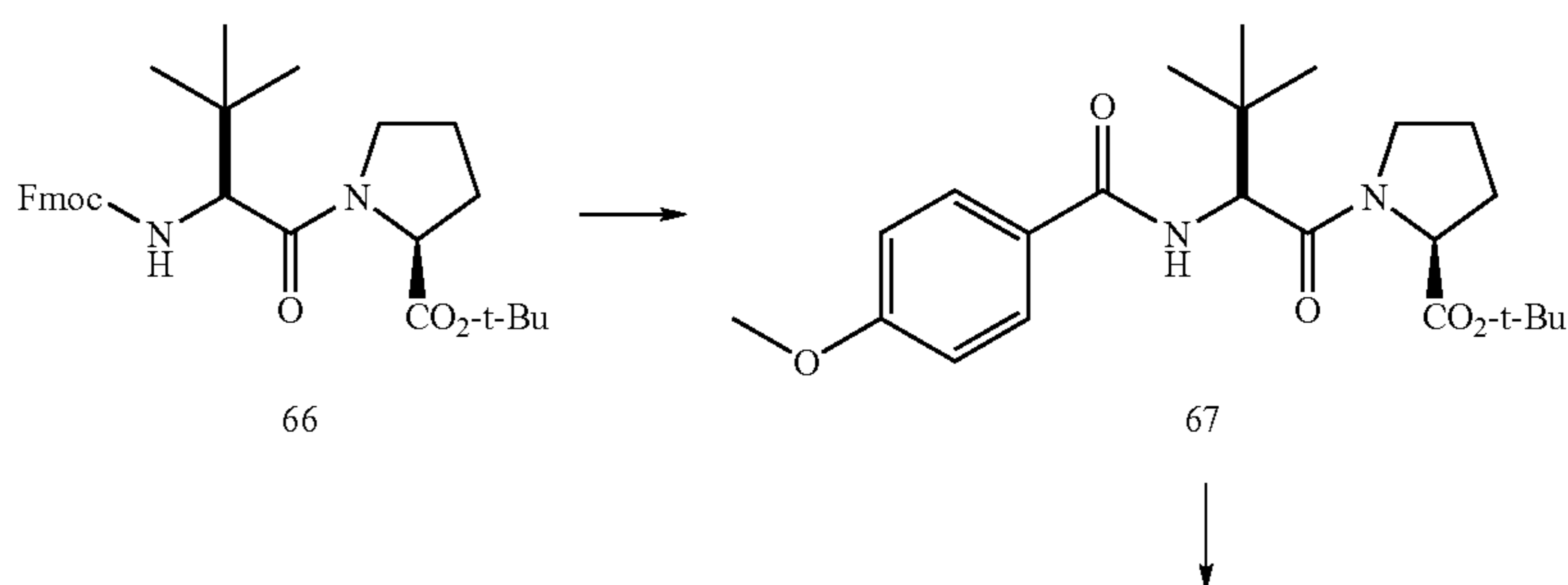
Scheme XIV
