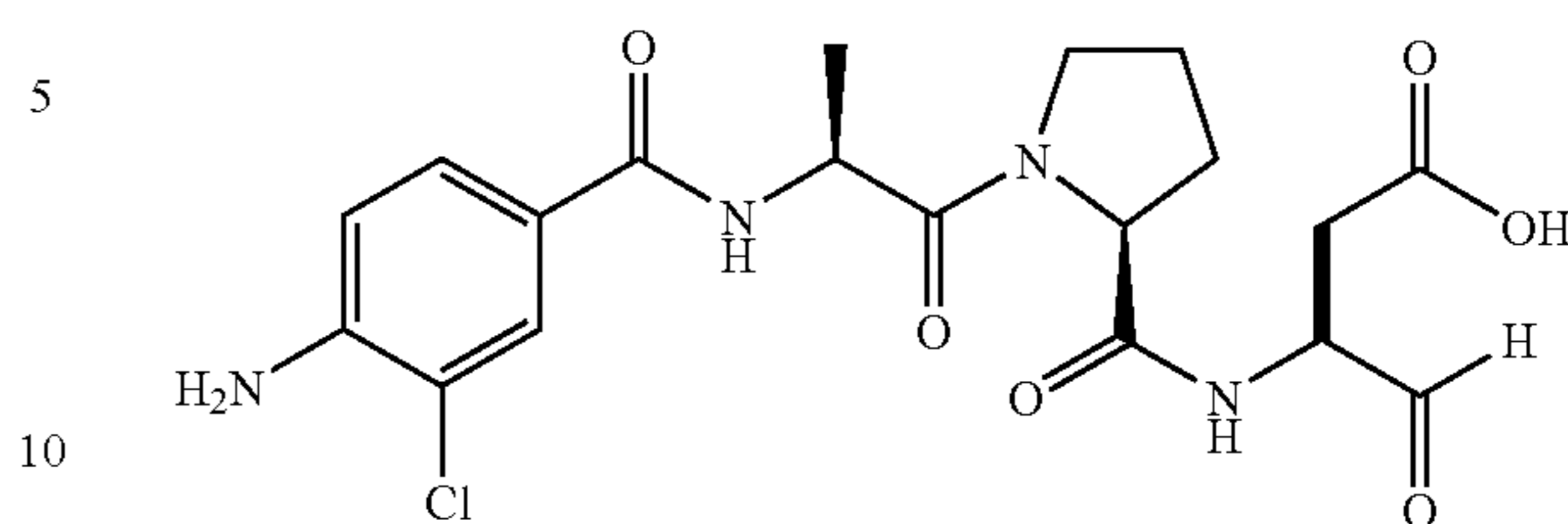
3-({1-[2-(4-Amino-3-chloro-benzoylamino)-propionyl]-pyrrolidine-2-carbonyl}-amino)-4-oxo-butanoic acid (122b)
