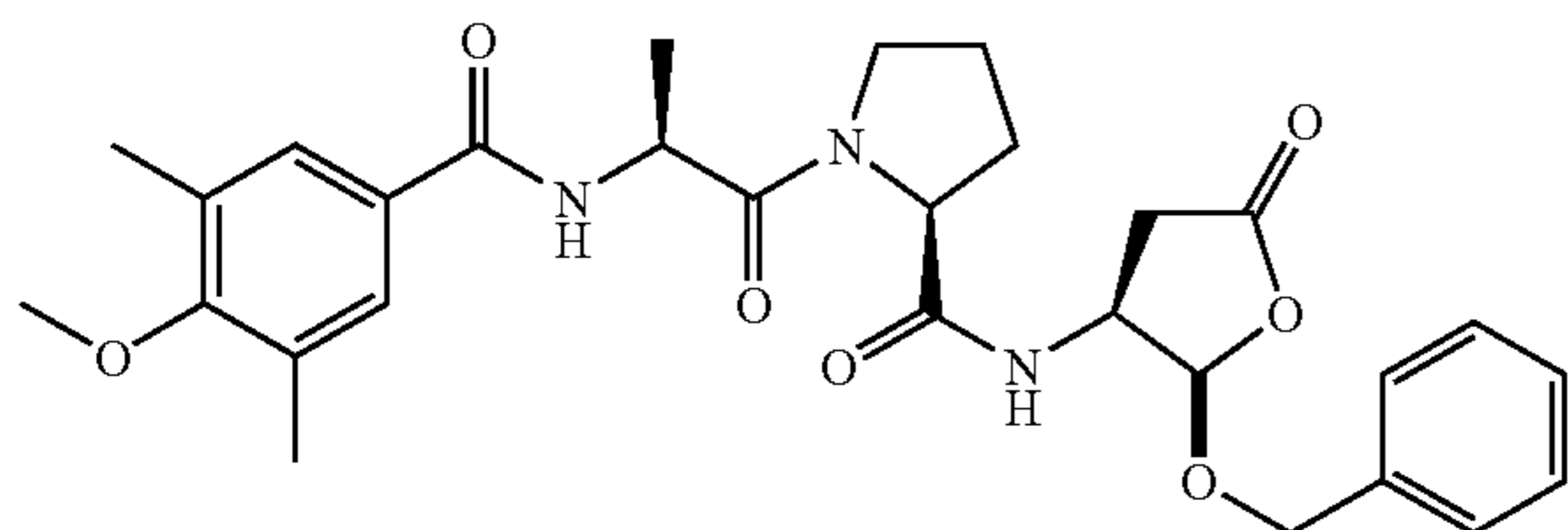
1-[2-(4-Methoxy-3,5-dimethyl-benzoylamino)-propionyl]-pyrrolidine-2-carboxylic acid (2-benzyloxy-5-oxo-tetrahydro-furan-3-yl)-amide (98ag)
