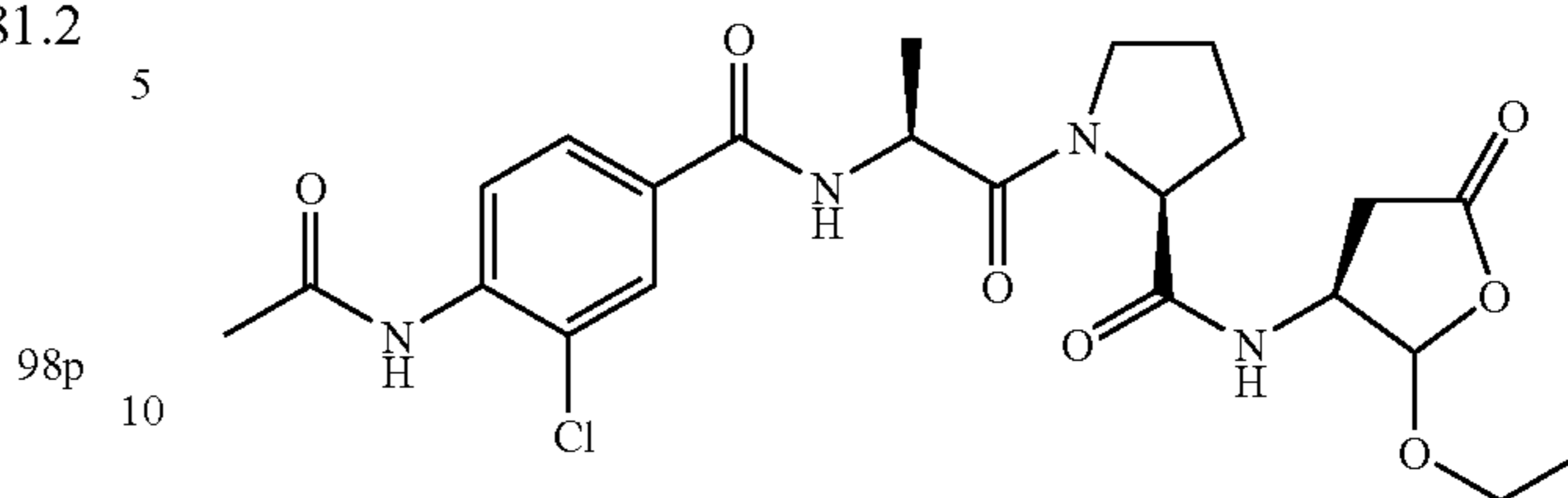
Synthesis of 1-[2-(4-acetylamino-3-chloro-benzoylamino)-propionyl]-pyrrolidine-2-carboxylic acid (2-ethoxy-5-oxo-tetrahydro-furan-3-yl)-amide (98r)
