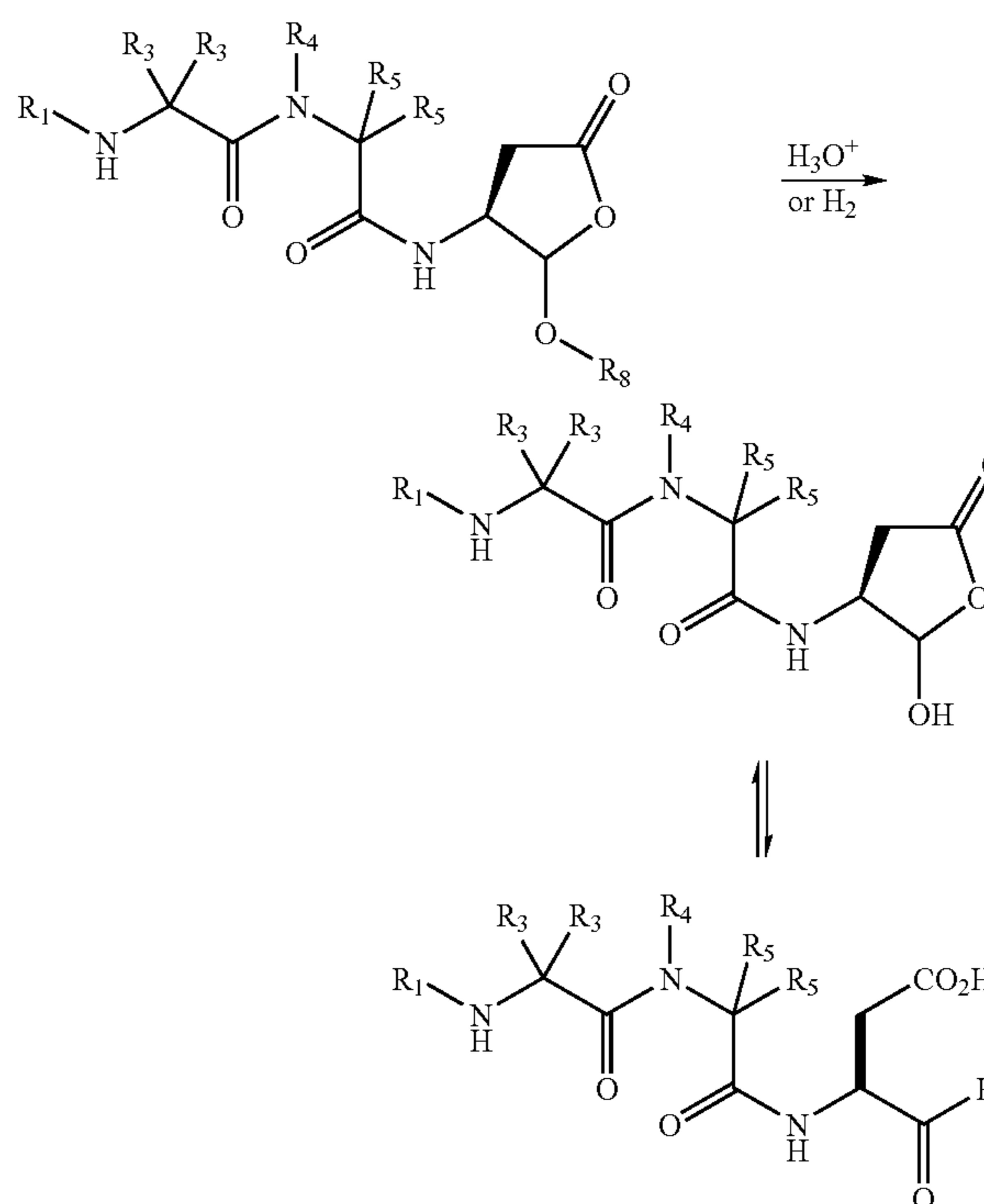
Scheme XXIII
