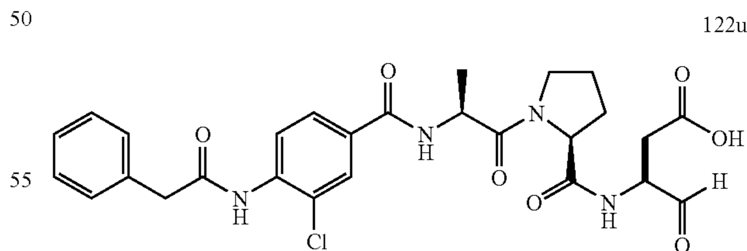
3-({1-[2-(3-Chloro-4-phenylacetylamino-benzoylamino)-propionyl]-pyrrolidine-2-carbonyl}-amino)-4-oxo-butyric acid (122u)
