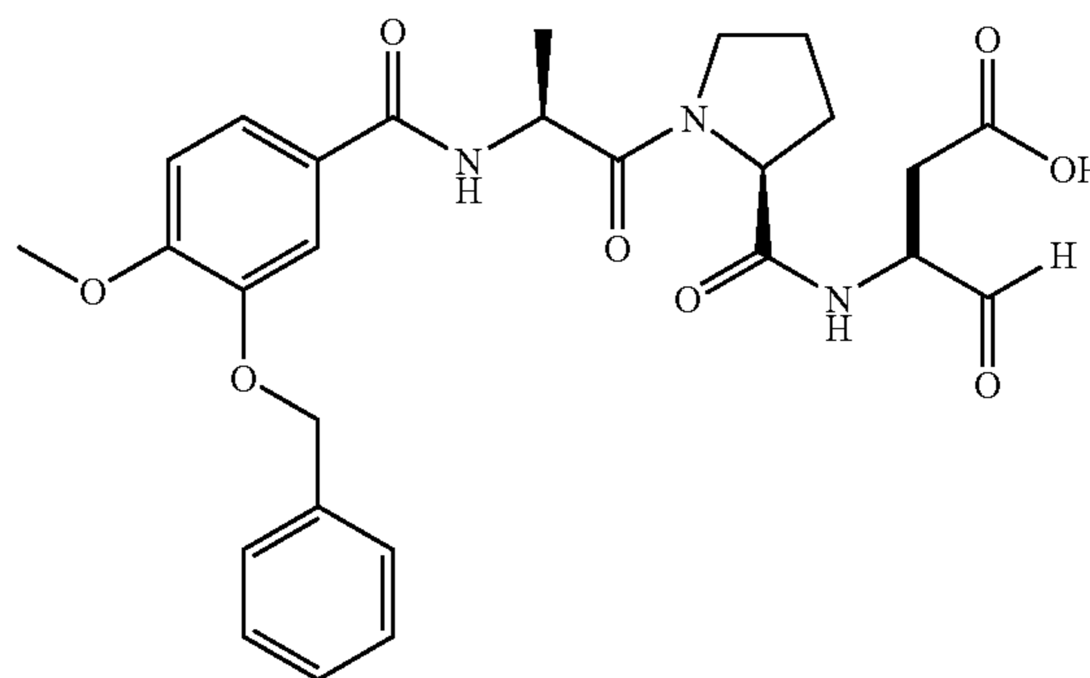
3-({1-[2-(3-benzyloxy-4-methoxy-benzoylamino)-propionyl]-pyrrolidine-2-carbonyl}-amino)-4-oxo-butylbutyric acid (122i)
