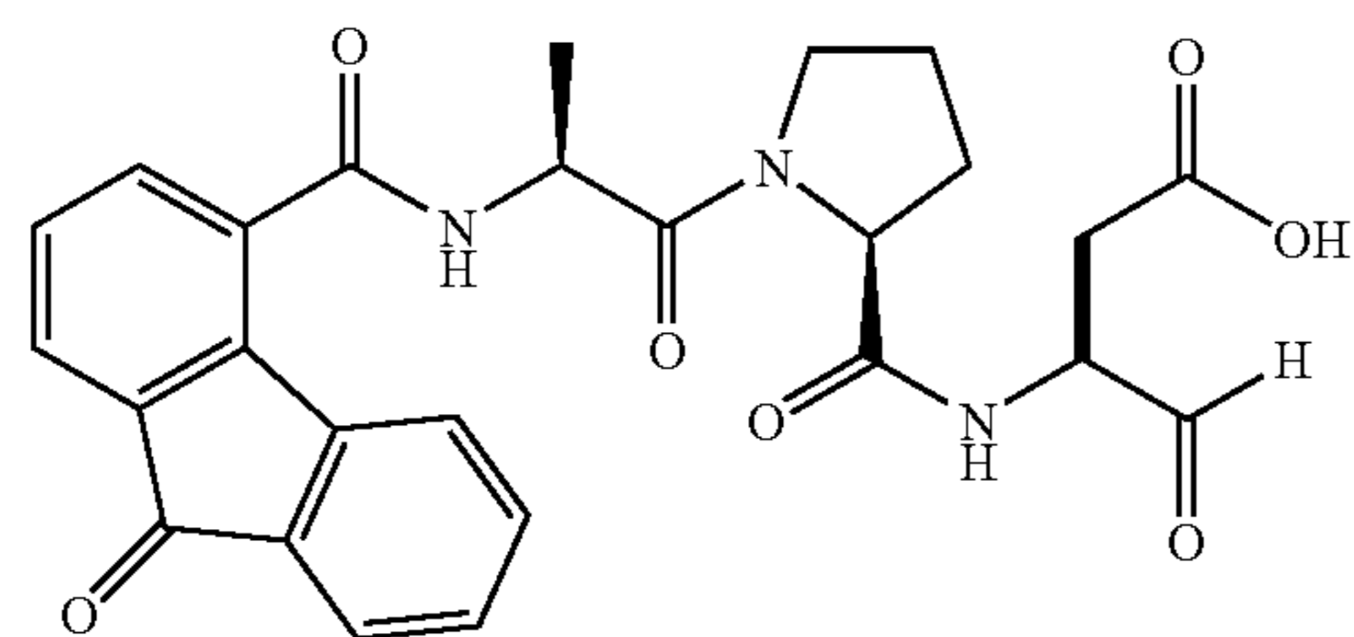
4-Oxo-3-[(1-{2-[9-oxo-9H-fluorene-4-carbonyl]-amino}-propionyl)-pyrrolidine-2-carbonyl]-amino]-butyric acid (122a)
