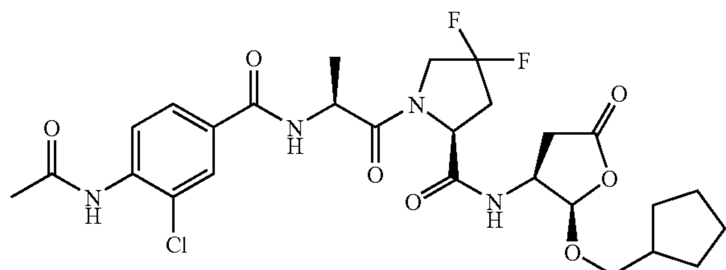
1-[2-(4-Acetylamino-3-chloro-benzoylamino)-propionyl]-4,4-difluoro-pyrrolidine-2-carboxylic acid (2-cyclopentylmethoxy-5-oxo-tetrahydro-furan-3-yl)-amide (116g)
