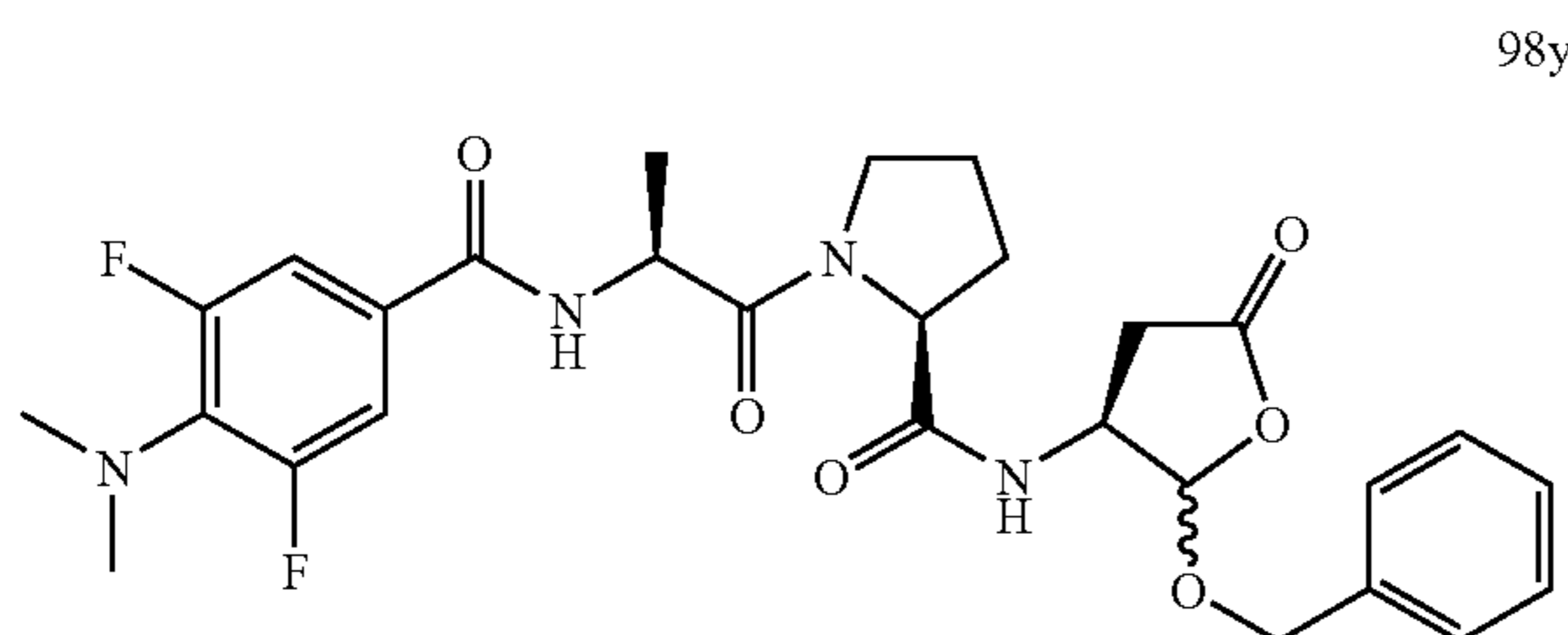
1-[2-(4-dimethylamino-3,5-difluoro-benzoylamino)-propionyl]-pyrrolidine-2-carboxylic acid (2-benzyloxy-5-oxo-tetrahydro-furan-3-yl)-amide (98y)
