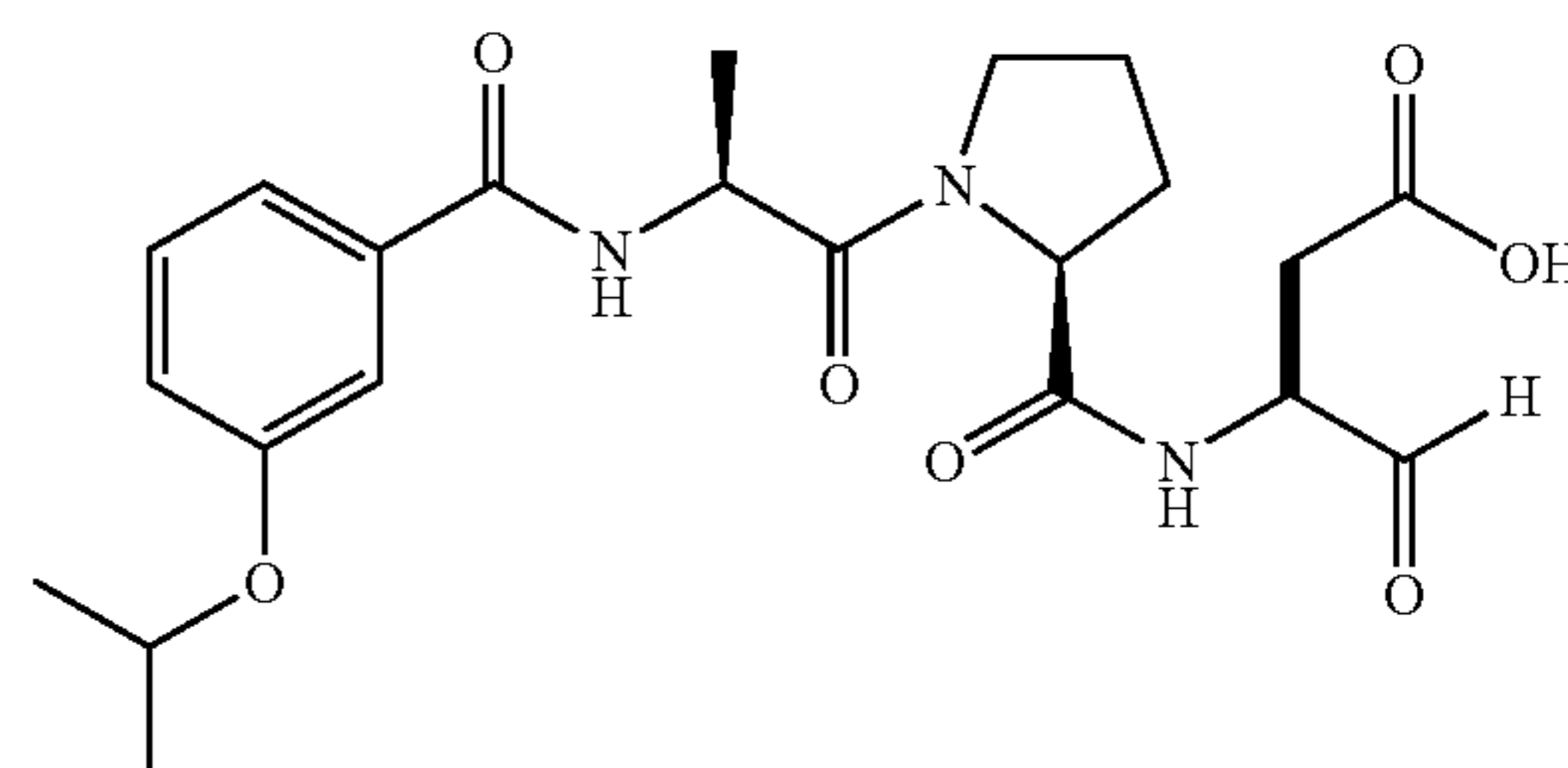
3-({1-[2-(3-Isopropoxy-benzoylamino)-propionyl]-pyrrolidine-2-carbonyl}-amino)-4-oxo-butylbutyric acid (122h)
