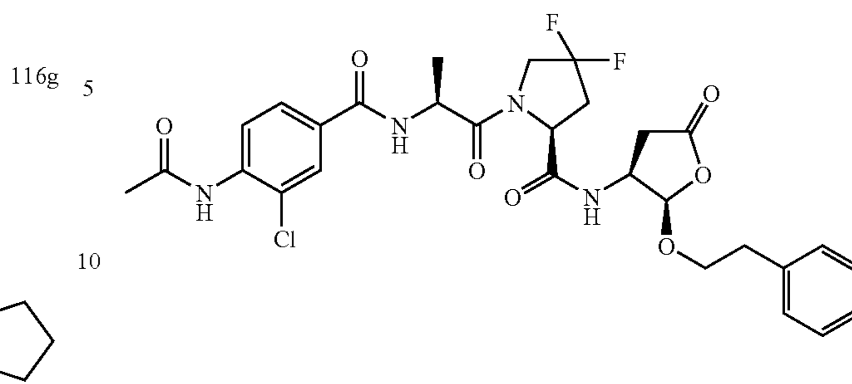
1-[2-(4-Acetylamino-3-chloro-benzoylamino)-propionyl]-4,4-difluoro-pyrrolidine-2-carboxylic acid (2-phenylethoxy-5-oxo-tetrahydro-furan-3-yl)-amide (116h)
