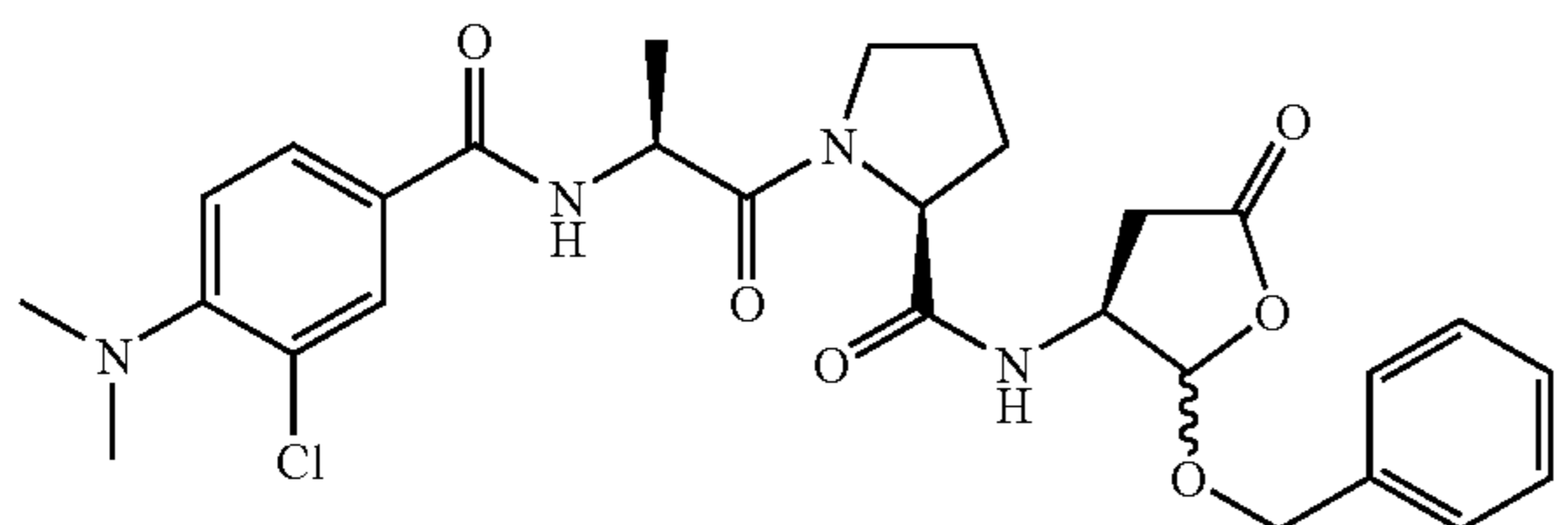
1-[2-(3-chloro-4-dimethylamino-benzoylamino)-propionyl]-pyrrolidine-2-carboxylic acid (2-benzyloxy-5-oxo-tetrahydro-furan-3-yl)-amide (98x)
