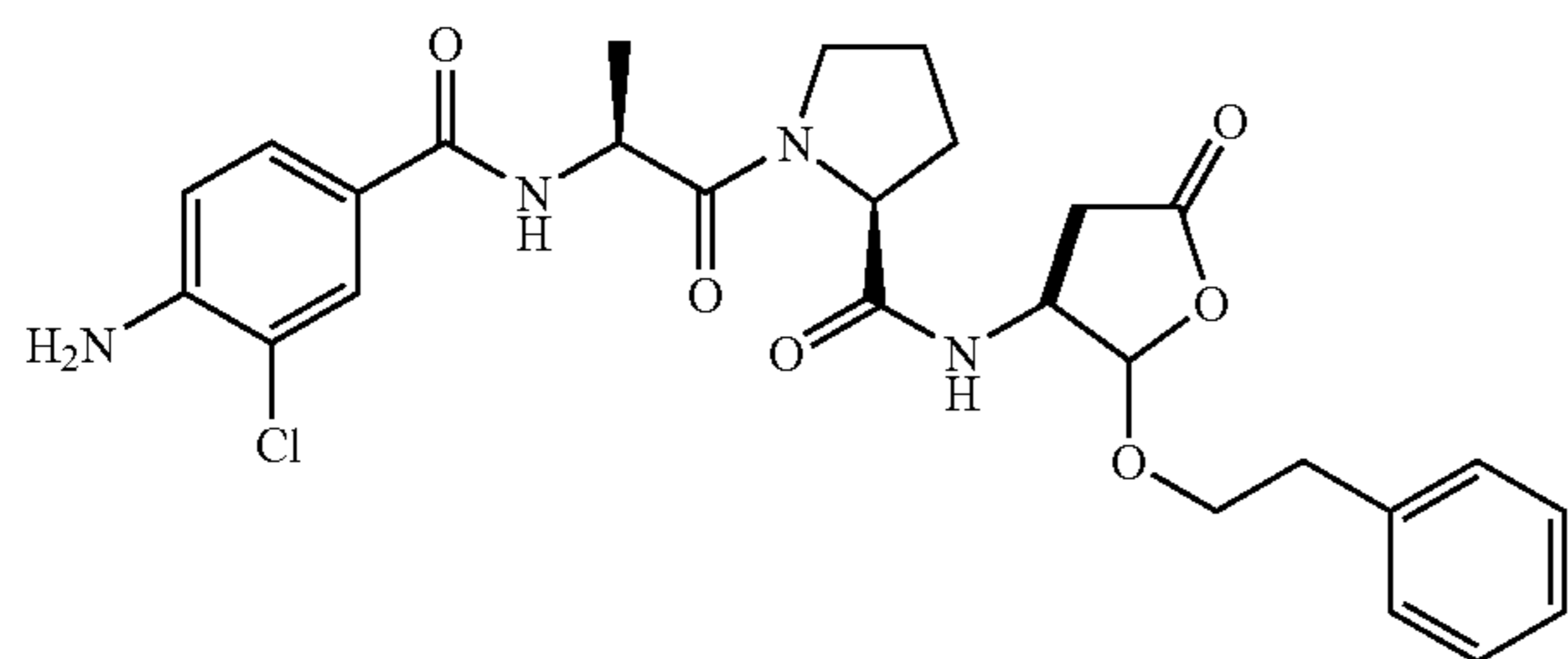
1-[2-(4-Amino-3-chloro-benzoylamino)-propionyl]-pyrrolidine-2-carboxylic acid (5-oxo-2-phenethyloxy-tetrahydro-furan-3-yl)-amide (98a)
