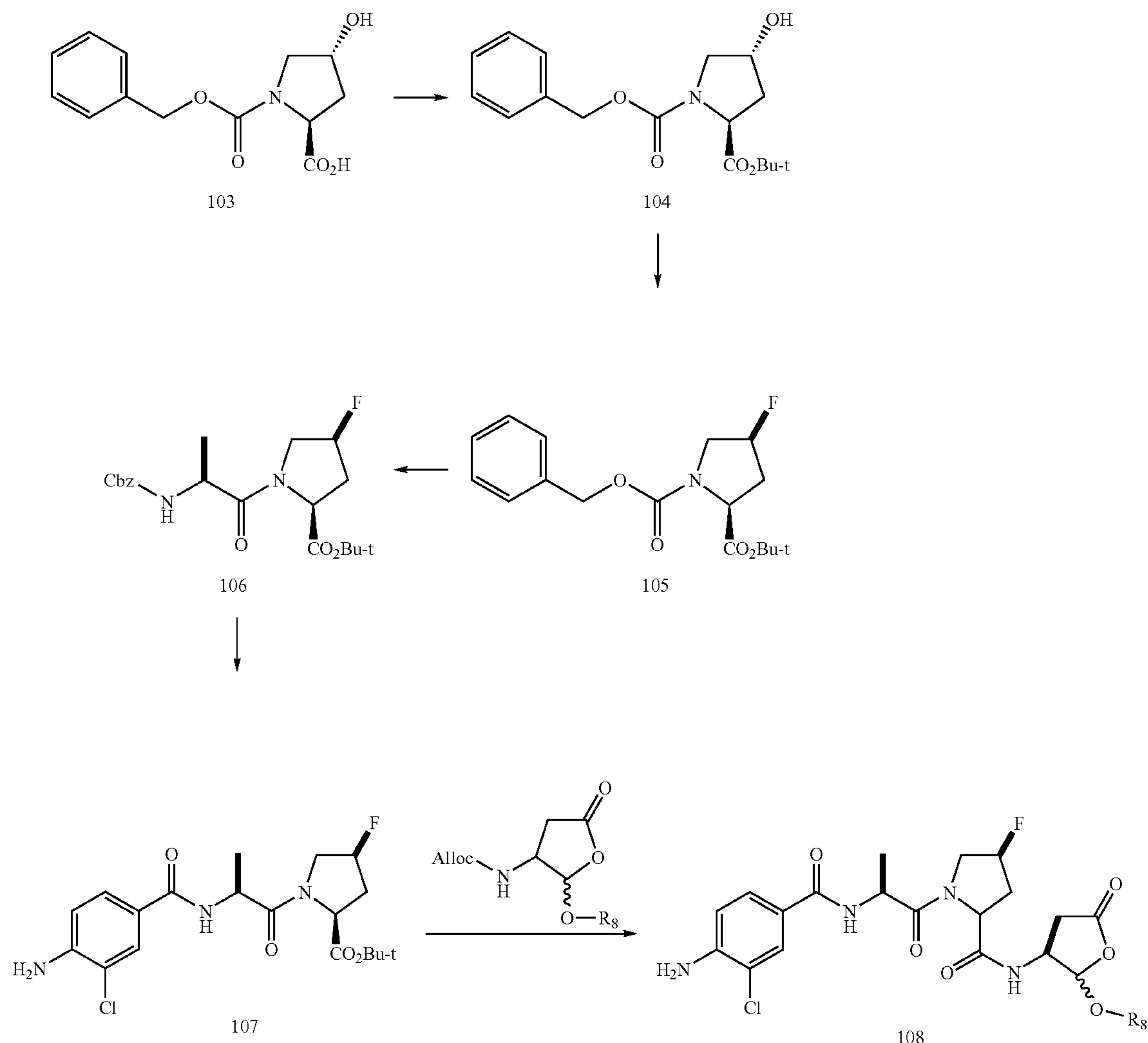
Scheme XIX
