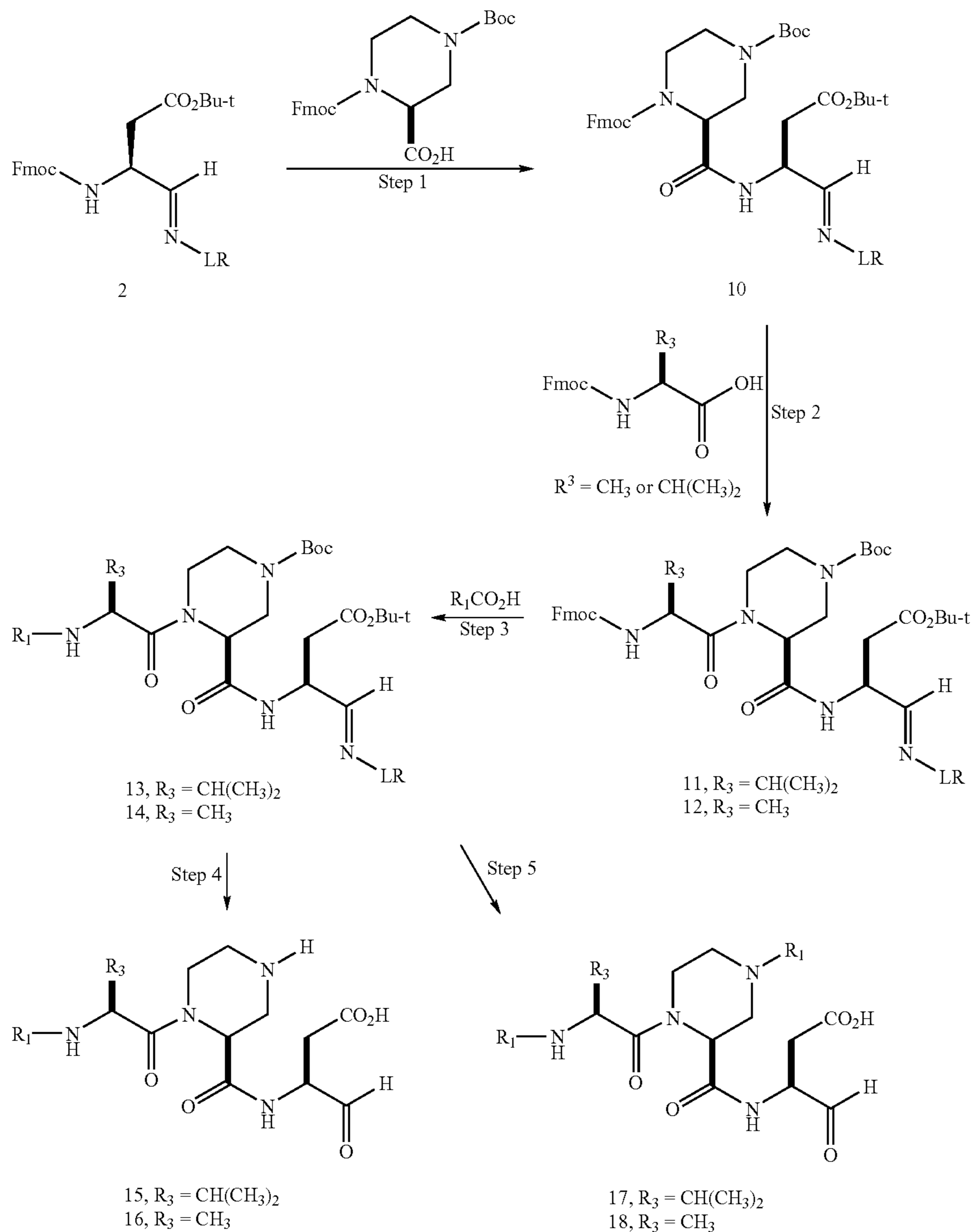
Scheme IV
