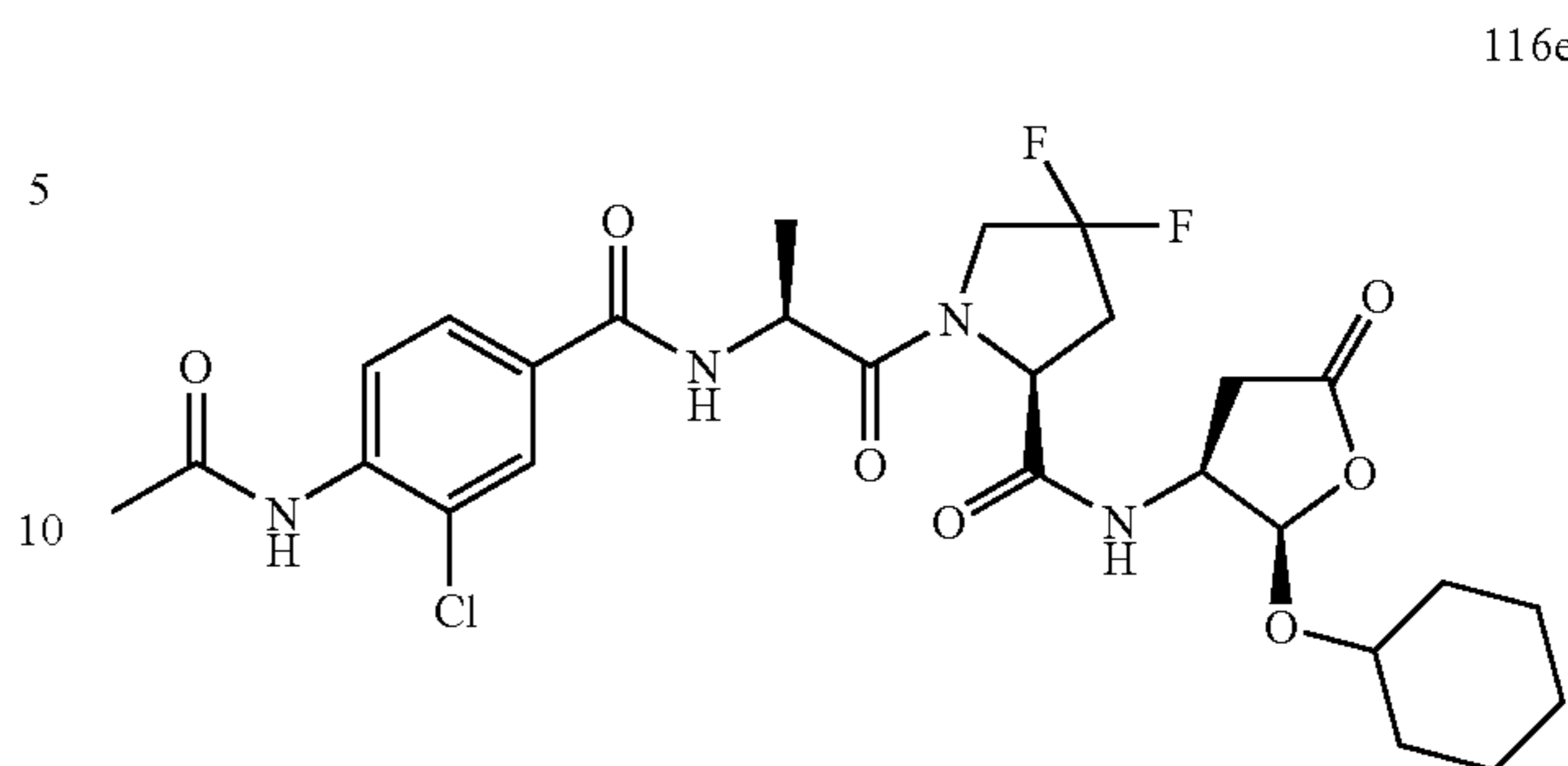
1-[2-(4-Acetylamino-3-chloro-benzoylamino)-propionyl]-4,4-difluoro-pyrrolidine-2-carboxylic acid (2-cyclohexyloxy-5-oxo-tetrahydro-furan-3-yl)-amide (116e)
