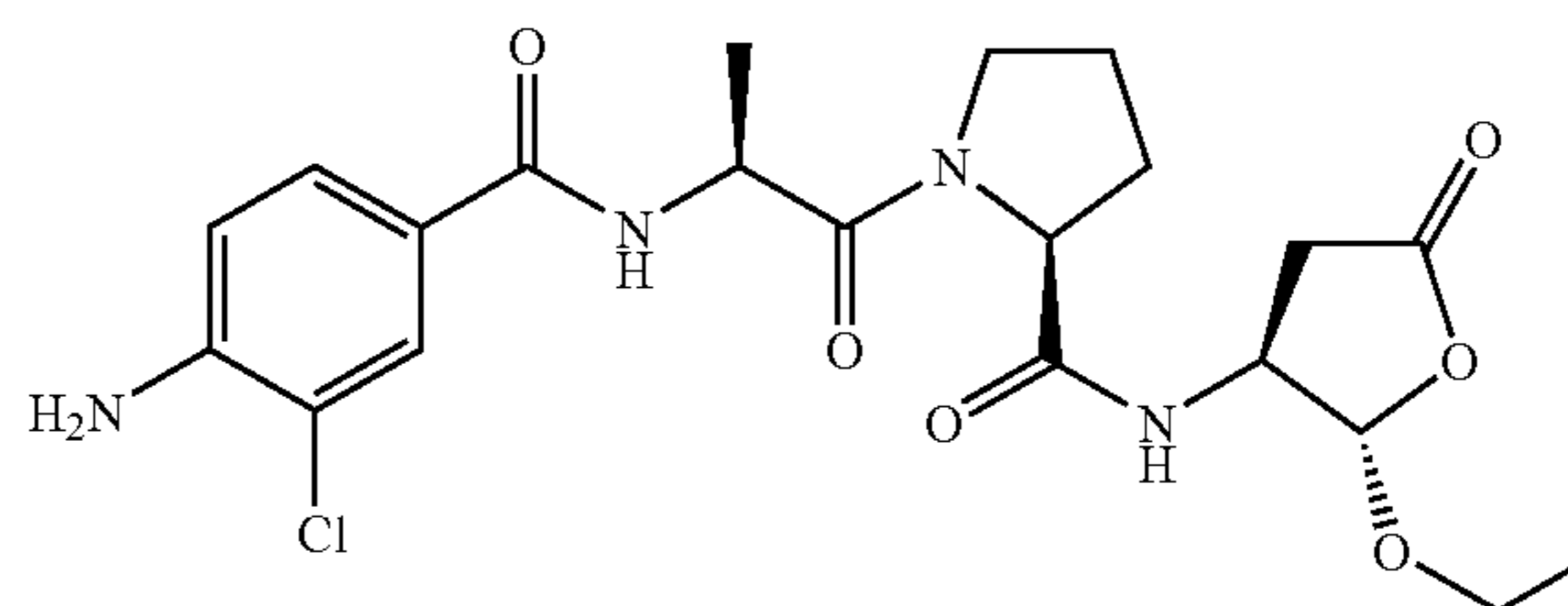
Synthesis of 1-[2-(4-amino-3-chloro-benzoylamino)-propionyl]-pyrrolidine-2-carboxylic acid (2-ethoxy-5-oxo-tetrahydro-furan-3-yl)-amide (98k)
