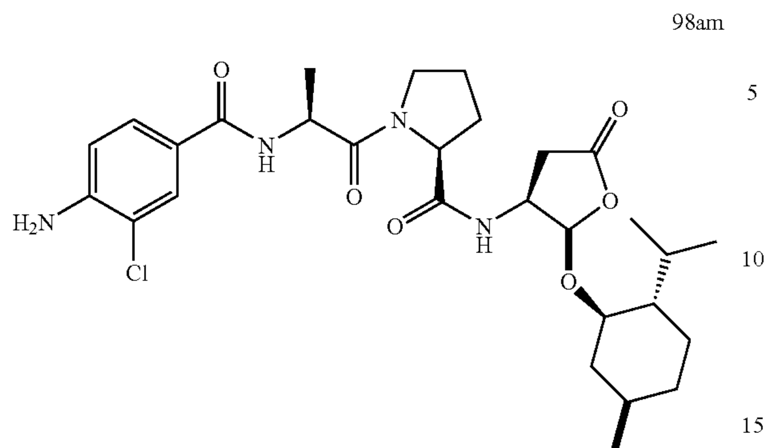
1-[2-(4-Amino-3-chloro-benzoylamino)-propionyl]-pyrrolidine-2-carboxylic acid {2R-[1R-(2S-isopropyl-5R-methyl-cyclohexyloxy)]-5-oxo-tetrahydro-furan-3-yl}-amide (98am)
