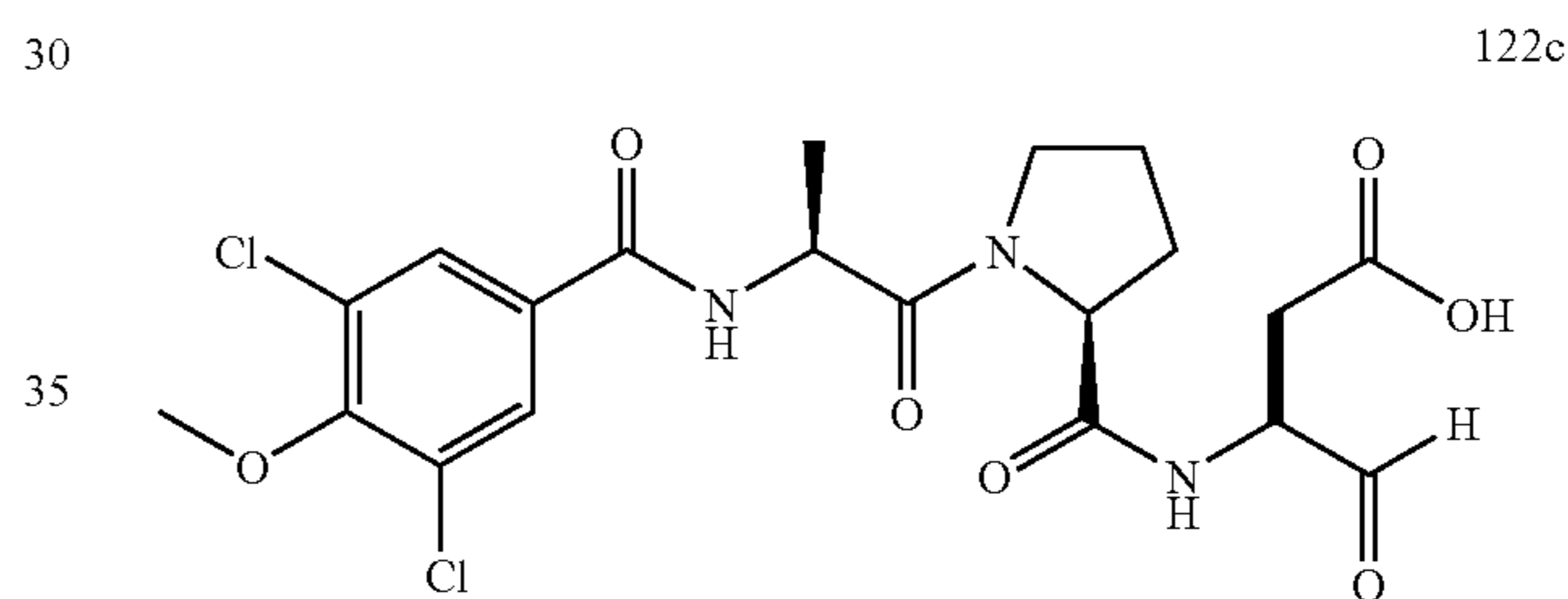
3-({1-[2-(3,5-Dichloro-4-methoxy-benzoylamino)-propionyl]-pyrrolidine-2-carbonyl}-amino)-4-oxo-butanoic acid (122c)
