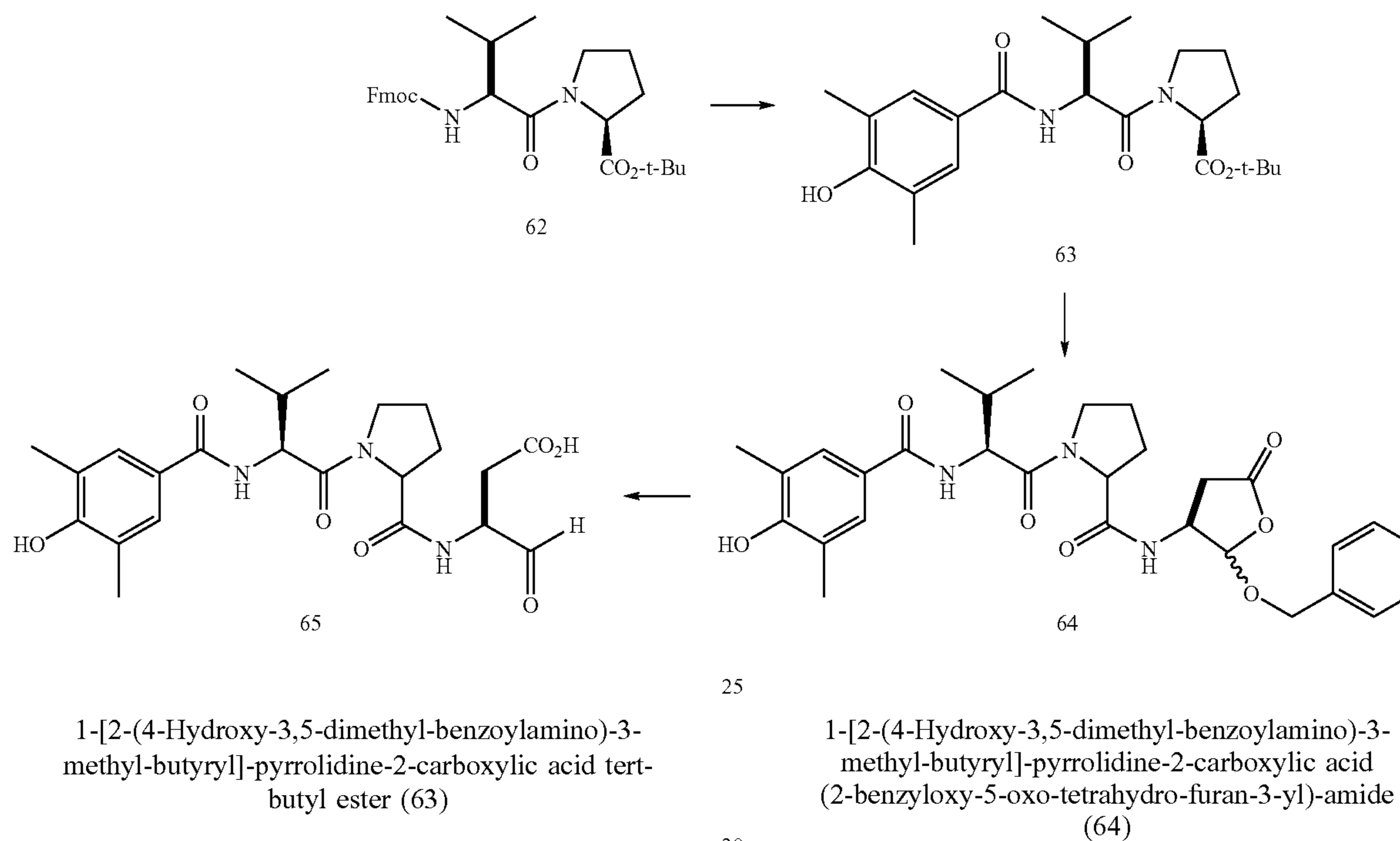
Scheme XIII
