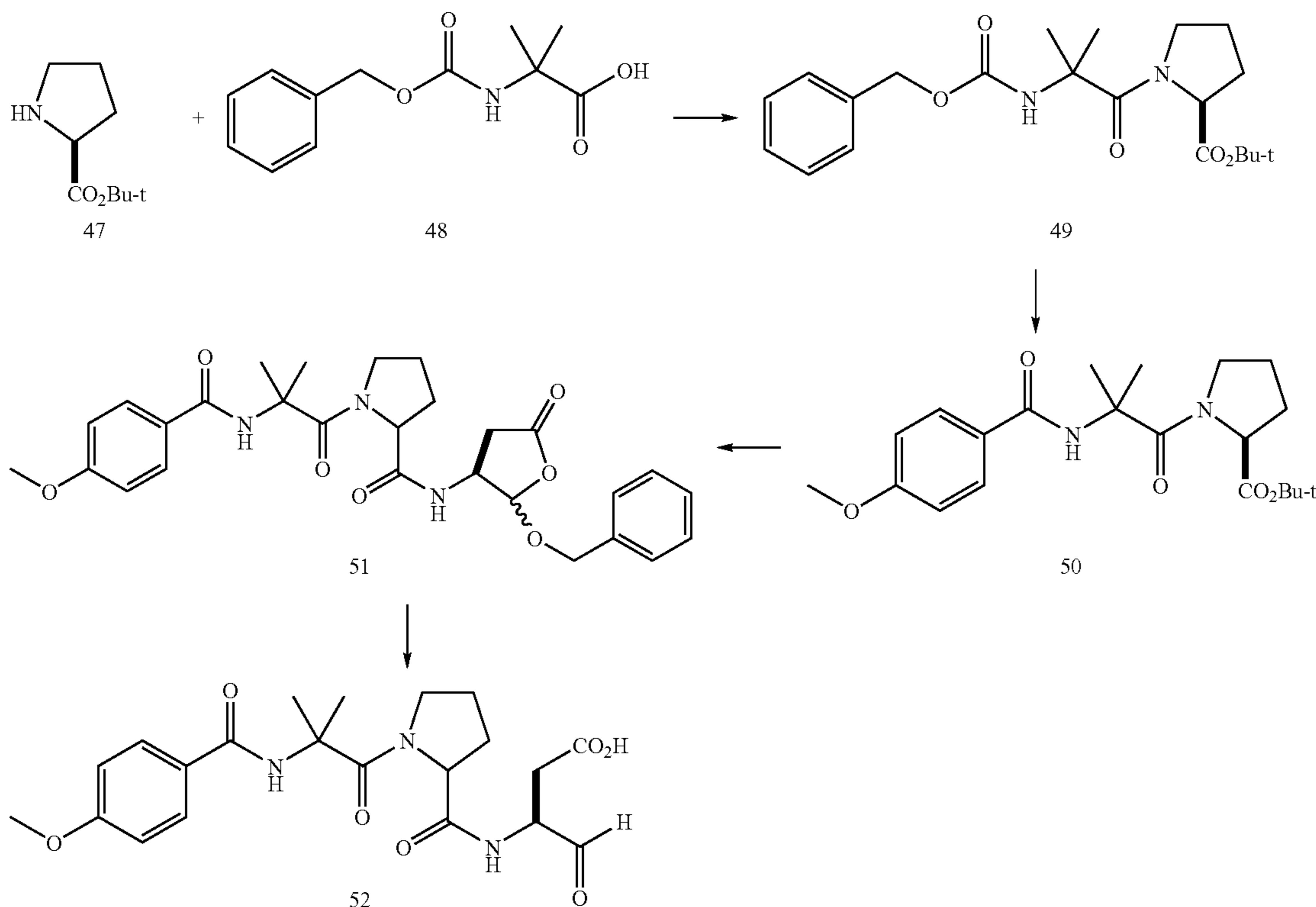
Scheme XI
