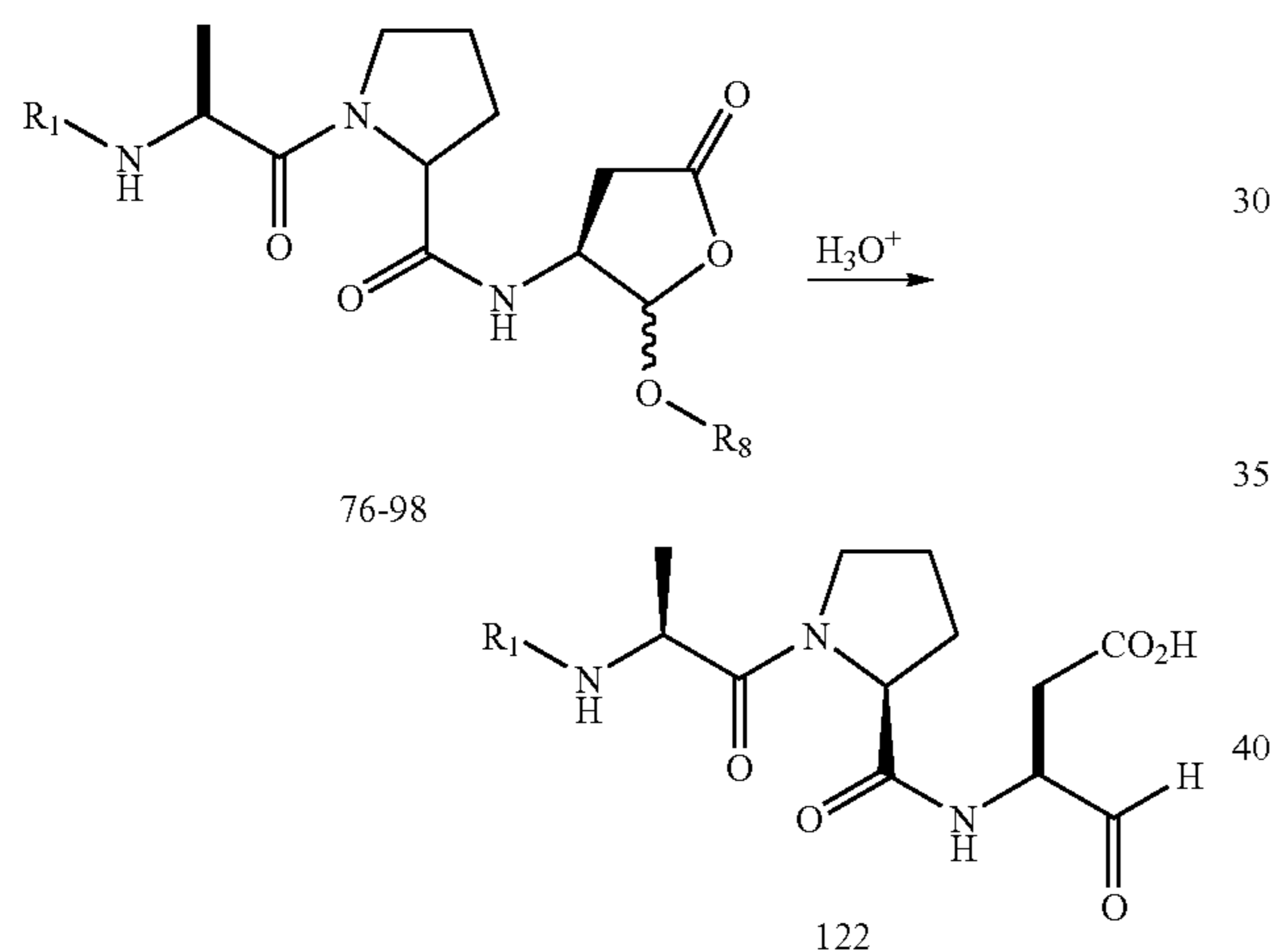
Scheme XXIV
