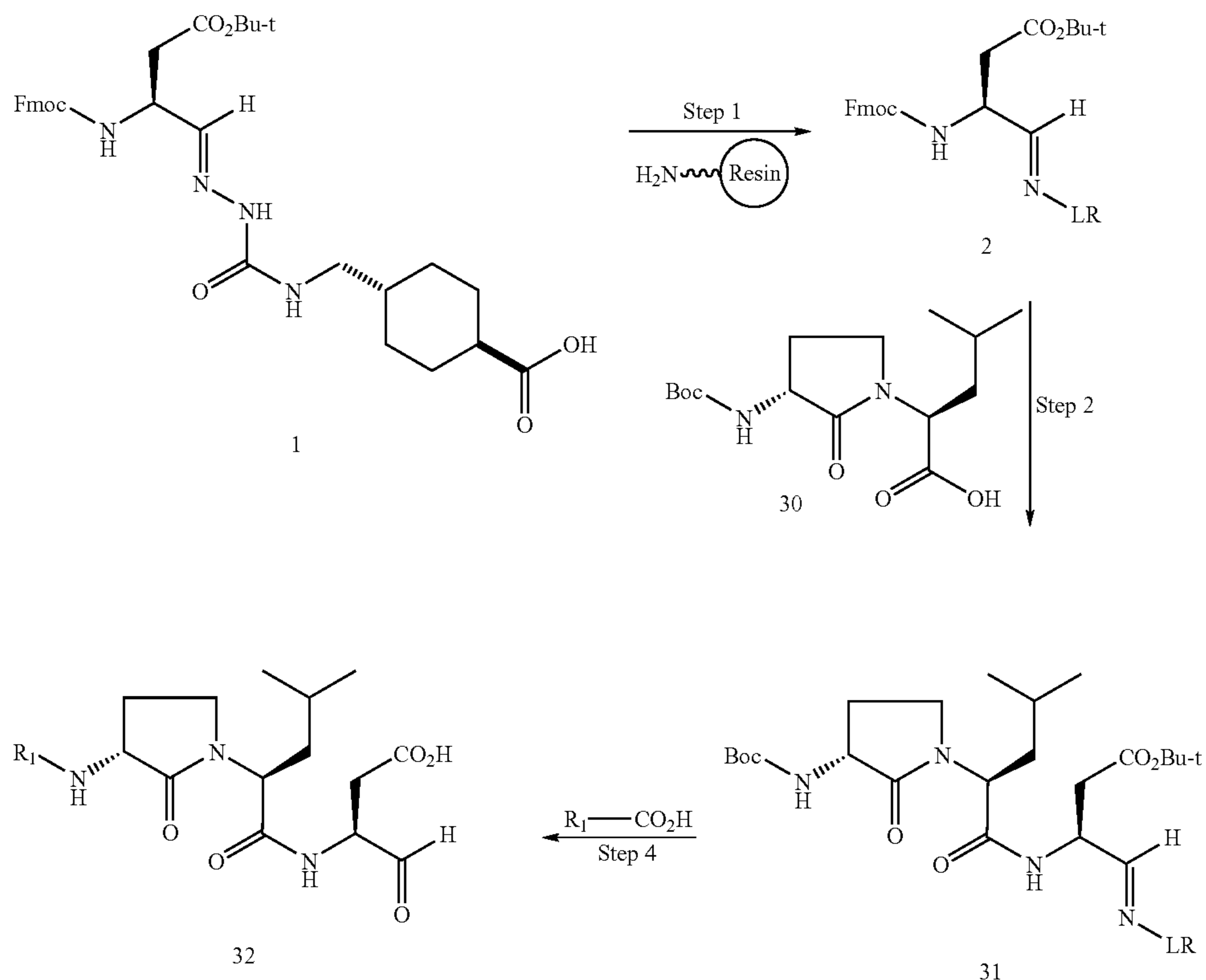
Scheme VII
