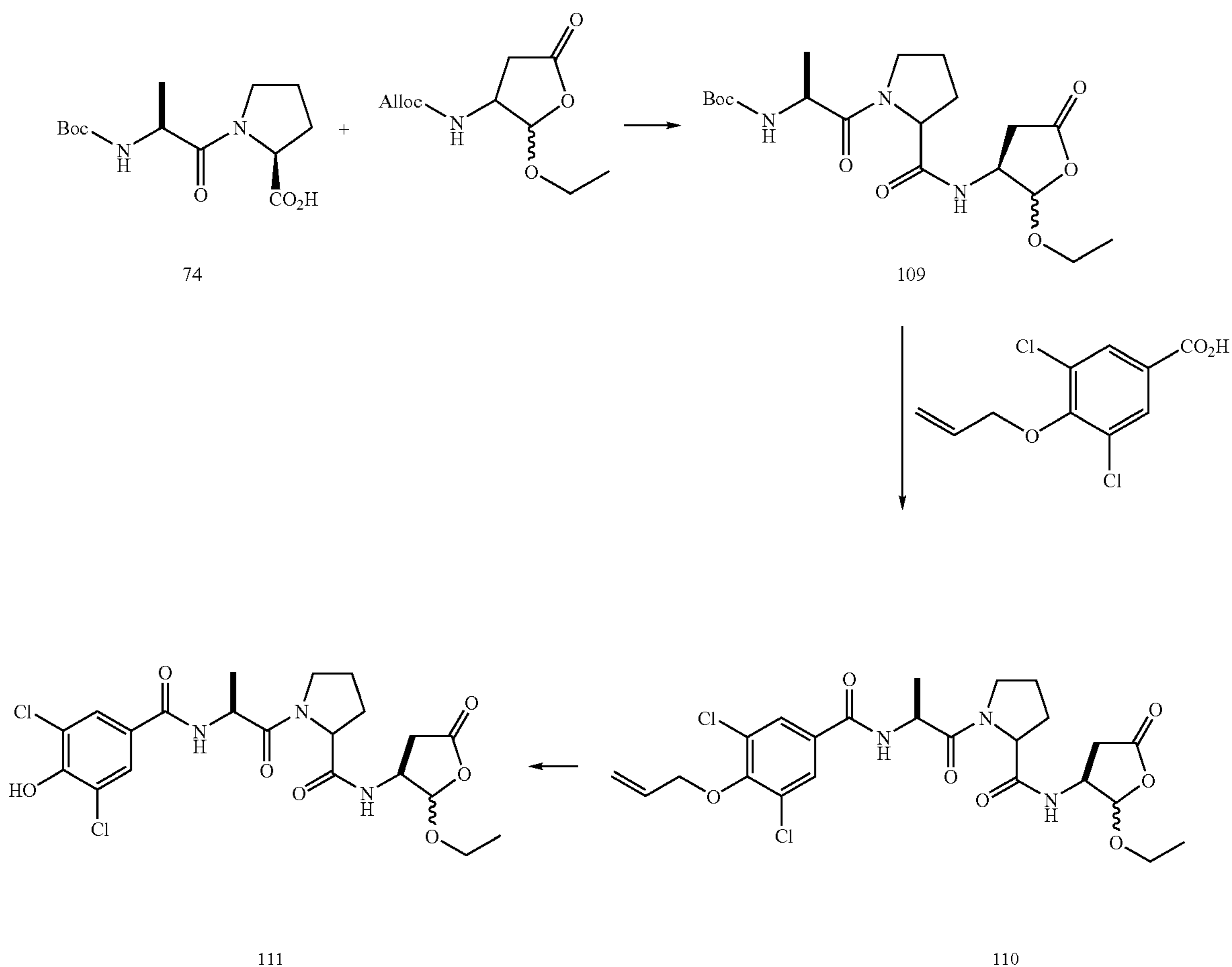
Scheme XX
