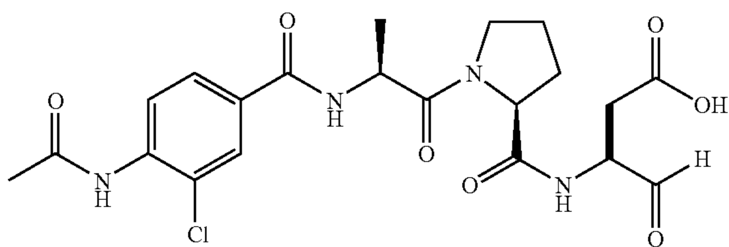
3-({1-[2-(4-Acetylamino-3-chloro-benzoylamino)-propionyl]-pyrrolidine-2-carbonyl}-amino)-4-oxo-butylbutyric acid (122f)
