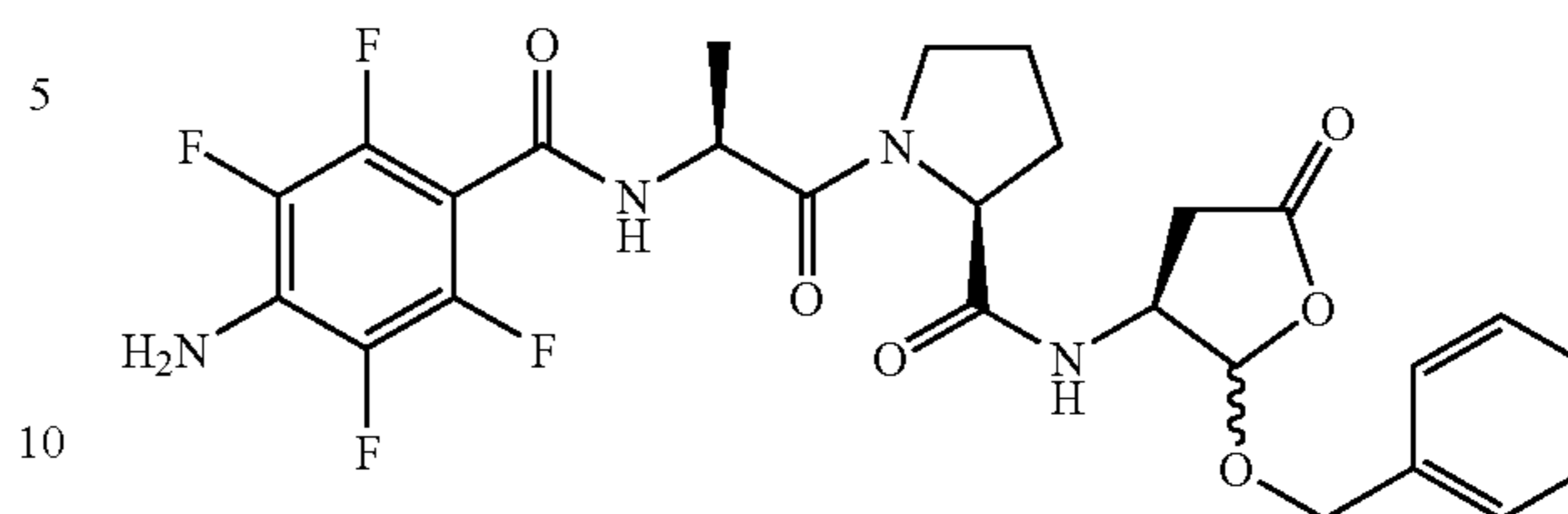
1-[2-(4-amino-2,3,5,6-tetrafluoro-benzoylamino)-propionyl]-pyrrolidine-2-carboxylic acid (2-benzyloxy-5-oxo-tetrahydro-furan-3-yl)-amide (98z)
