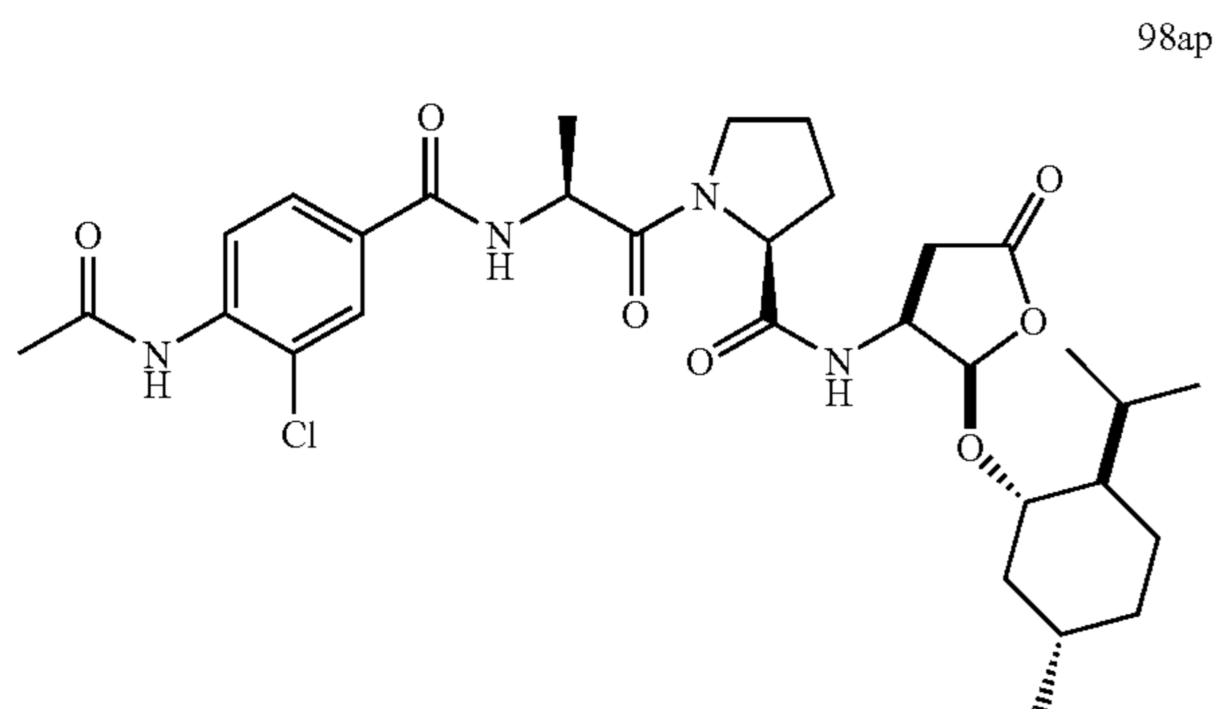
1-[2-(4-Acetylamino-3-chloro-benzoylamino)-propionyl]-pyrrolidine-2-carboxylic acid {2R-[1S-(2R-isopropyl-5S-methyl-cyclohexyloxy)]-5-oxo-tetrahydro-furan-3-yl}-amide (98ap)
