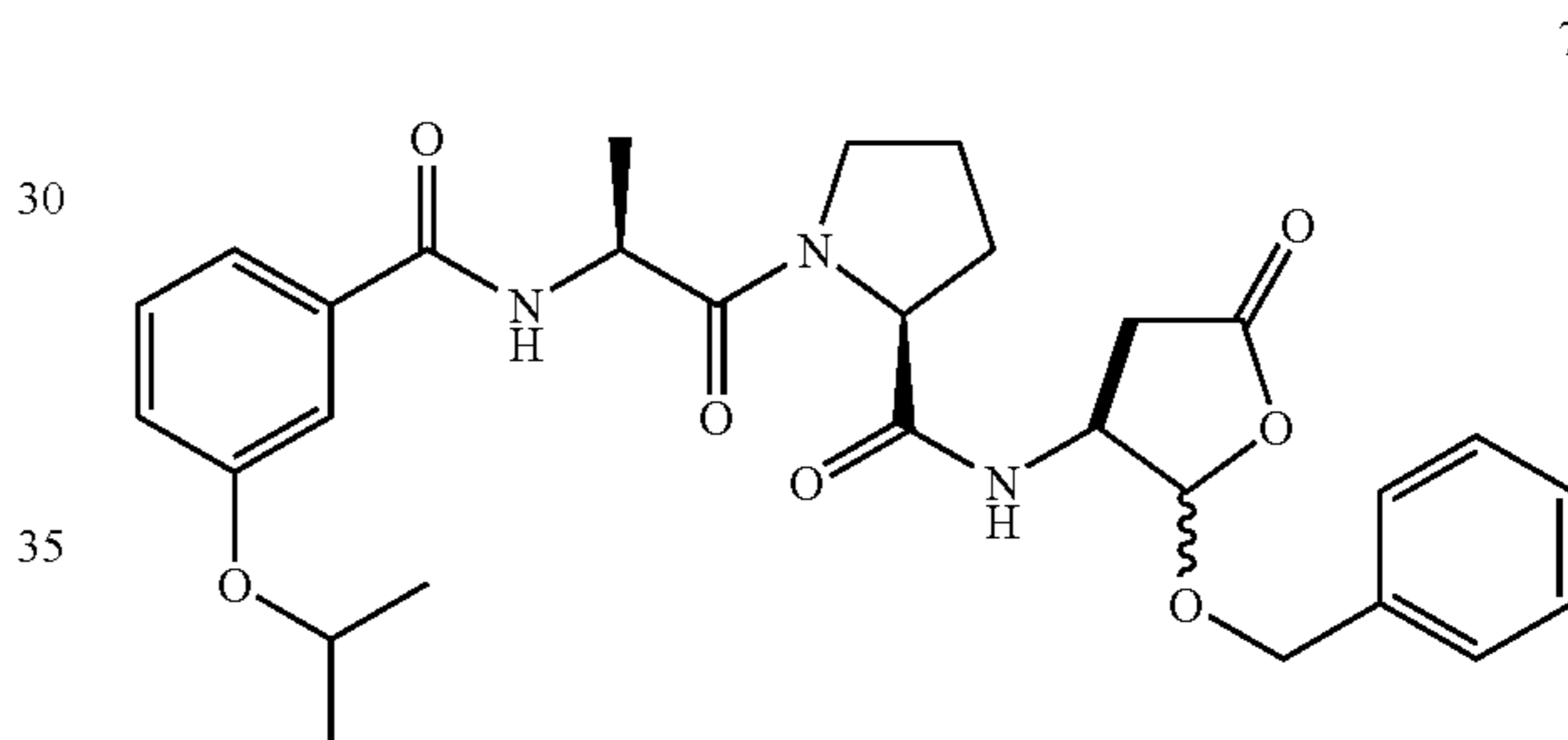
1-[2-(3-Isopropoxy-benzoylamino)-propionyl]-pyrrolidine-2-carboxylic acid (2-benzyloxy-5-oxo-tetrahydro-furan-3-yl)-amide (79)
