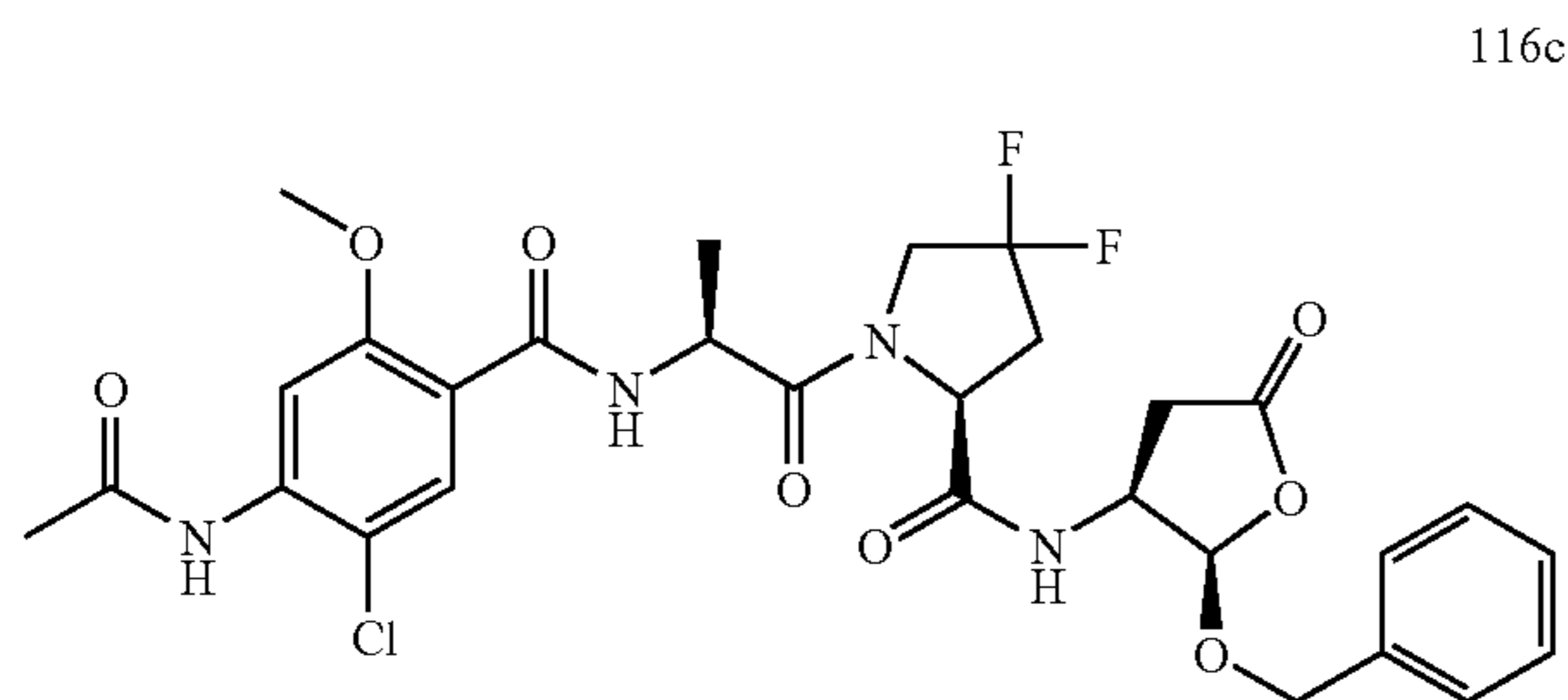
1-[2-(4-Acetylamino-5-chloro-2-methoxy-benzoylamino)-propionyl]-4,4-difluoro-pyrrolidine-2-carboxylic acid (2-benzyloxy-5-oxo-tetrahydro-furan-3-yl)-amide (116c)
