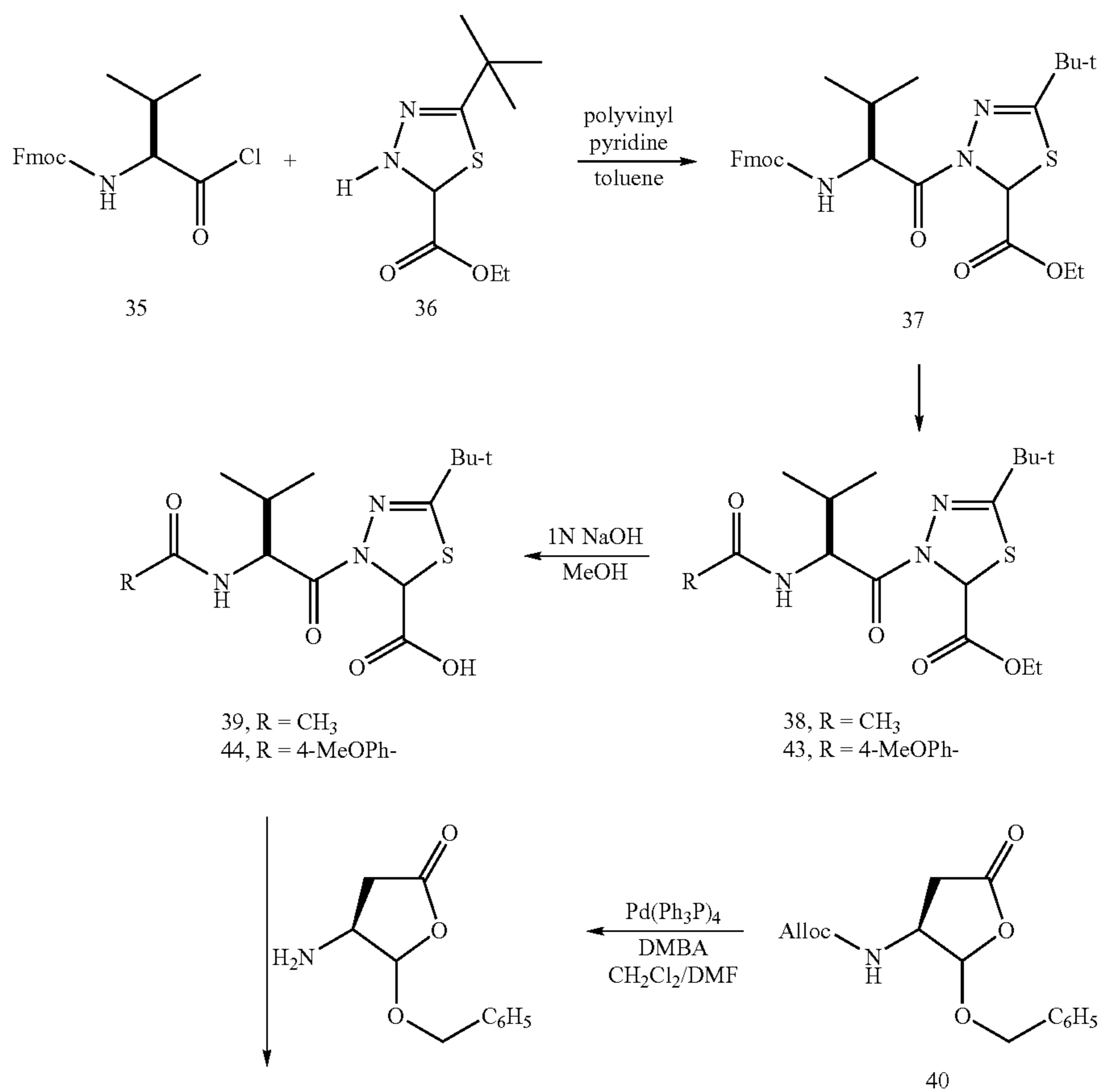
Scheme X
