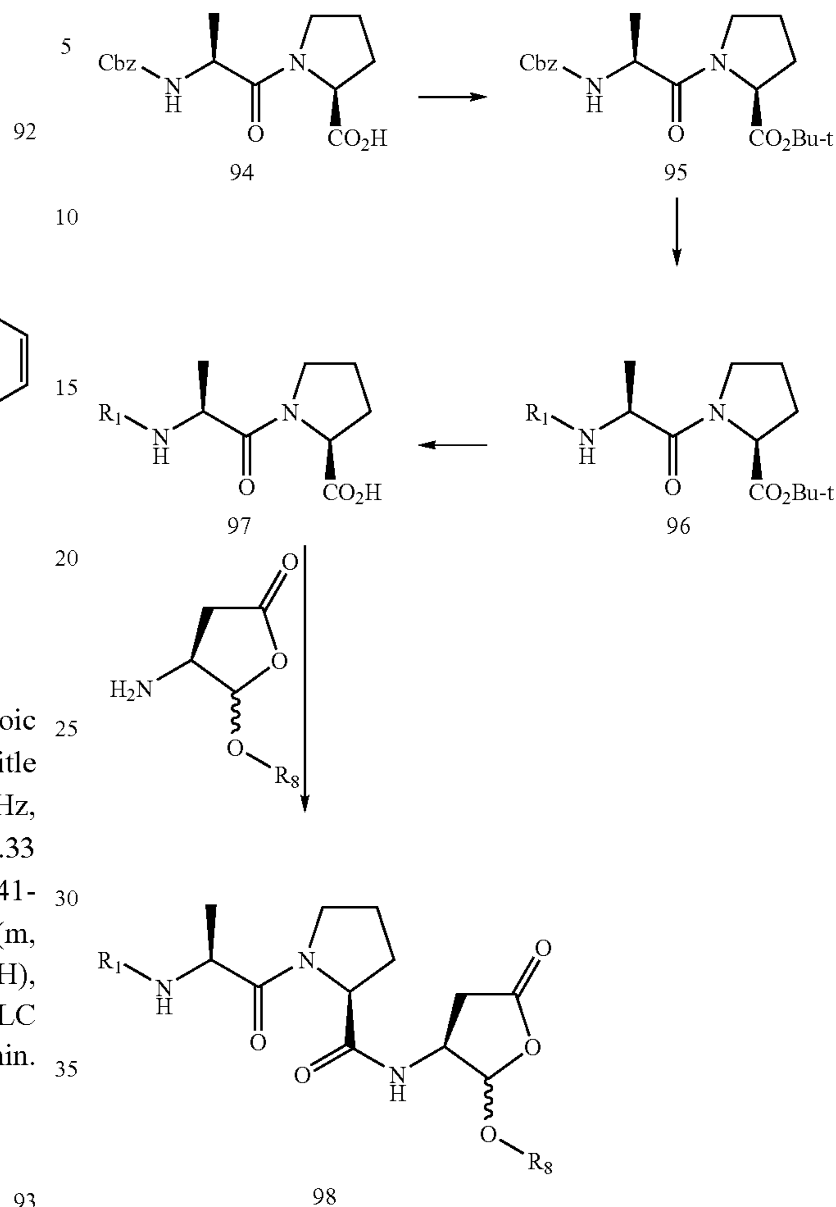
Scheme XVII
