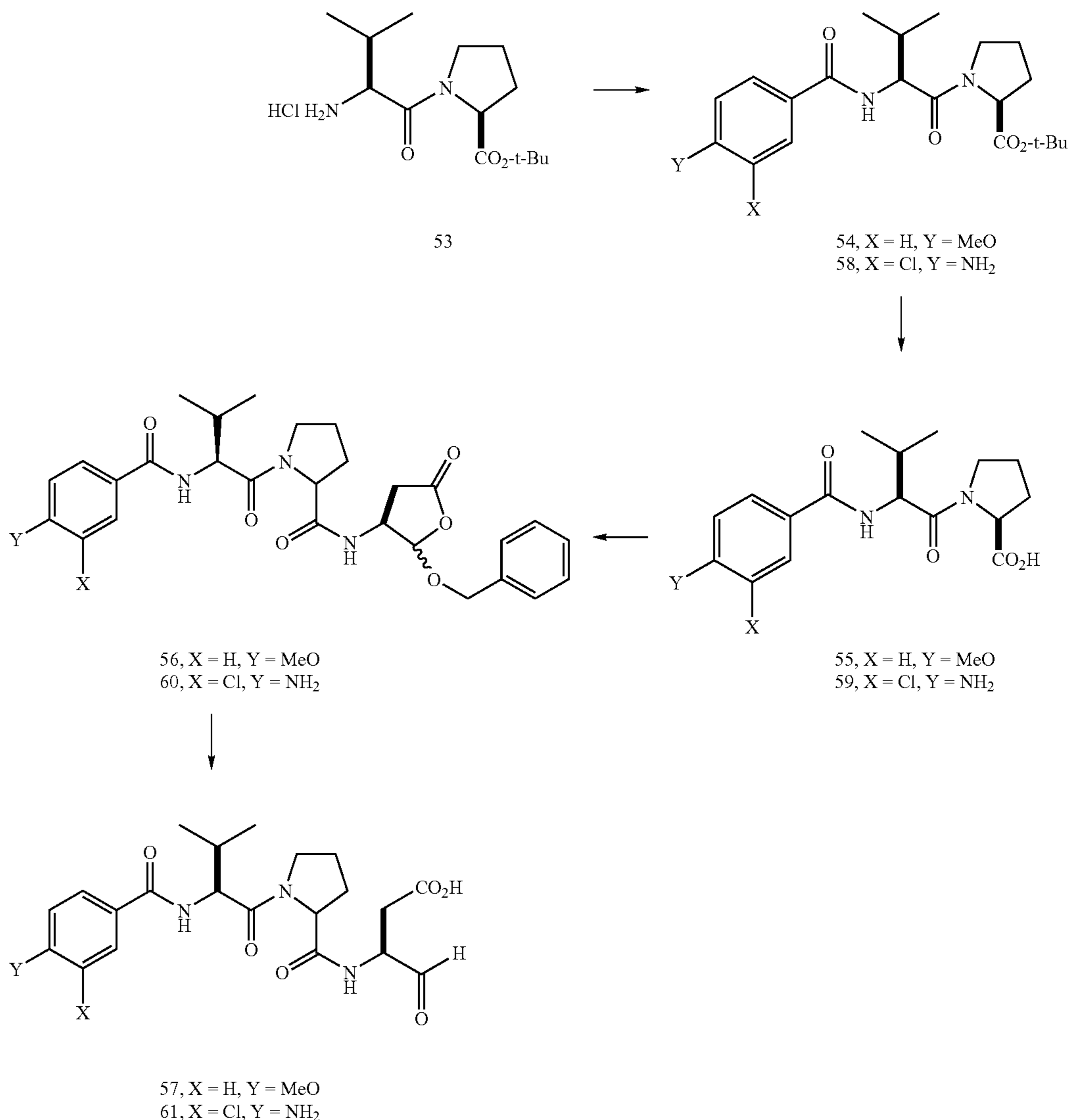
Scheme XII
