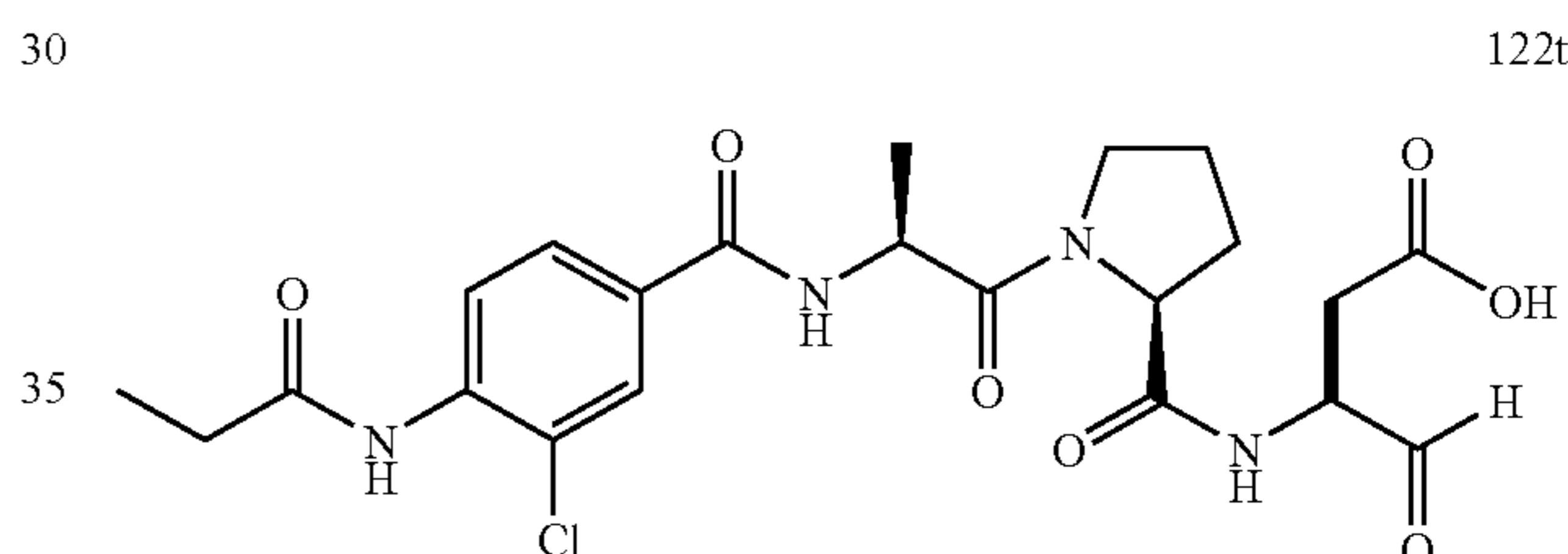
3-({1-[2-(3-Chloro-4-propionylamino-benzoylamino)-propionyl]-pyrrolidine-2-carbonyl}-amino)-4-oxo-butyric acid (122t)
