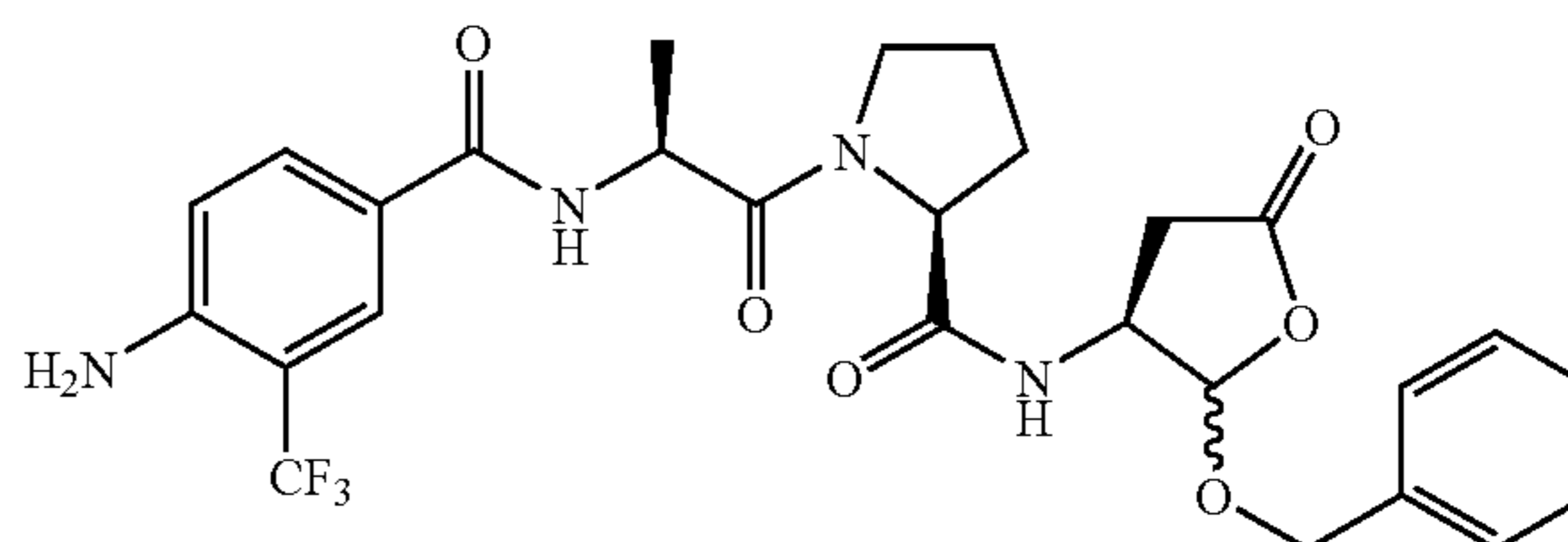
1-[2-(4-amino-3-trifluoromethyl-benzoylamino)-propionyl]-pyrrolidine-2-carboxylic acid (2-benzyloxy-5-oxo-tetrahydro-furan-3-yl)-amide (98w)
