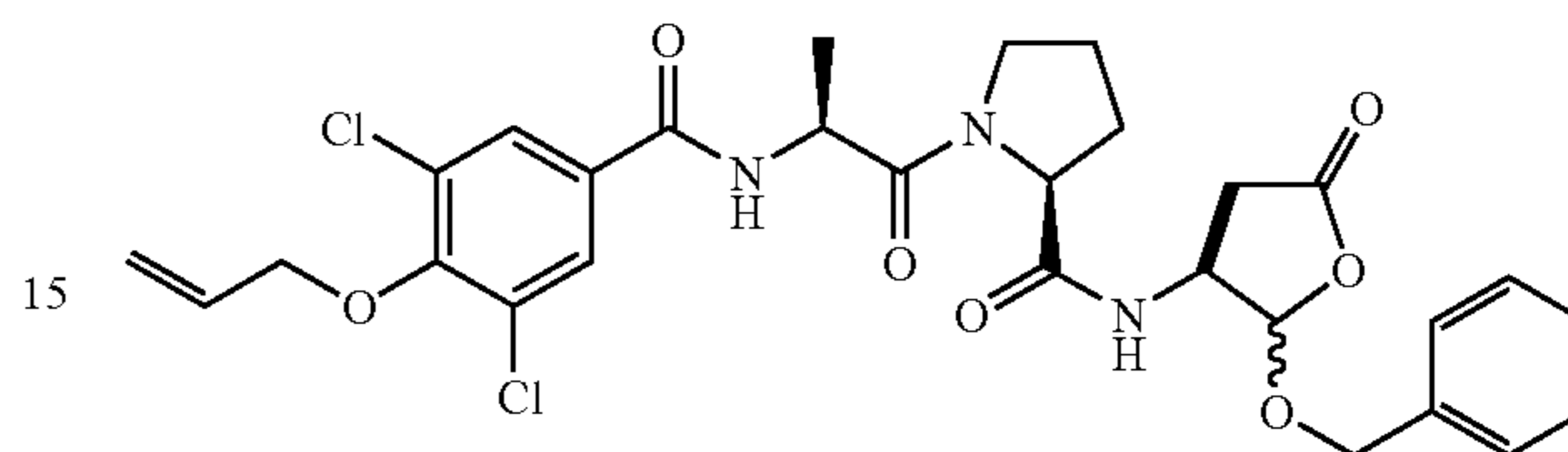
1-[2-(4-Allyloxy-3,5-dichloro-benzoylamino)-propionyl]-pyrrolidine-2-carboxylic acid (2-benzyloxy-5-oxo-tetrahydro-furan-3-yl)-amide (82)
