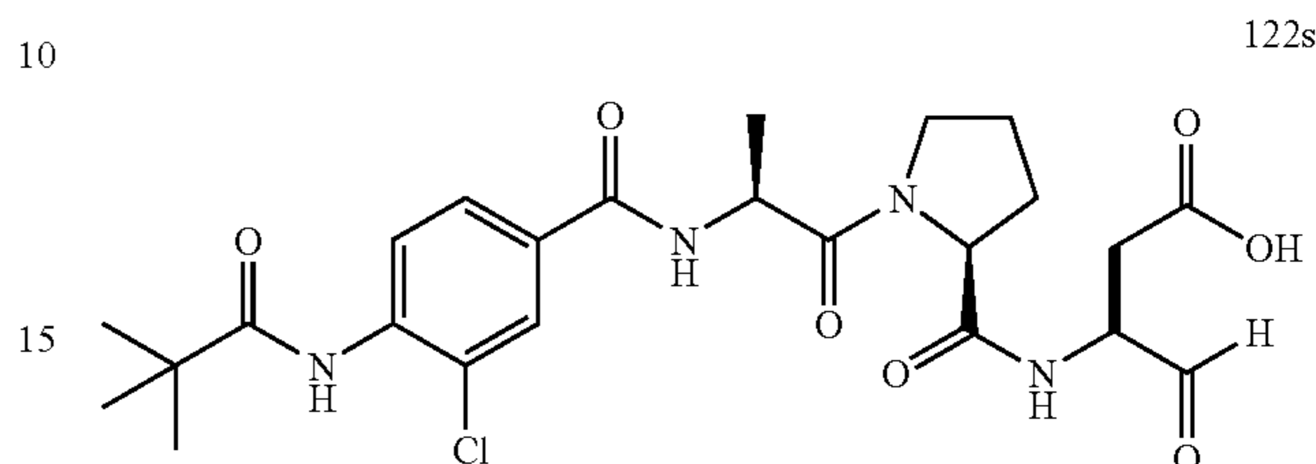
3-[(1-{2-[3-Chloro-4-(2,2-dimethyl-propionylamino)-benzoylamino]-propionyl}-pyrrolidine-2-carbonyl)-amino]-4-oxo-butyric acid (122s)
