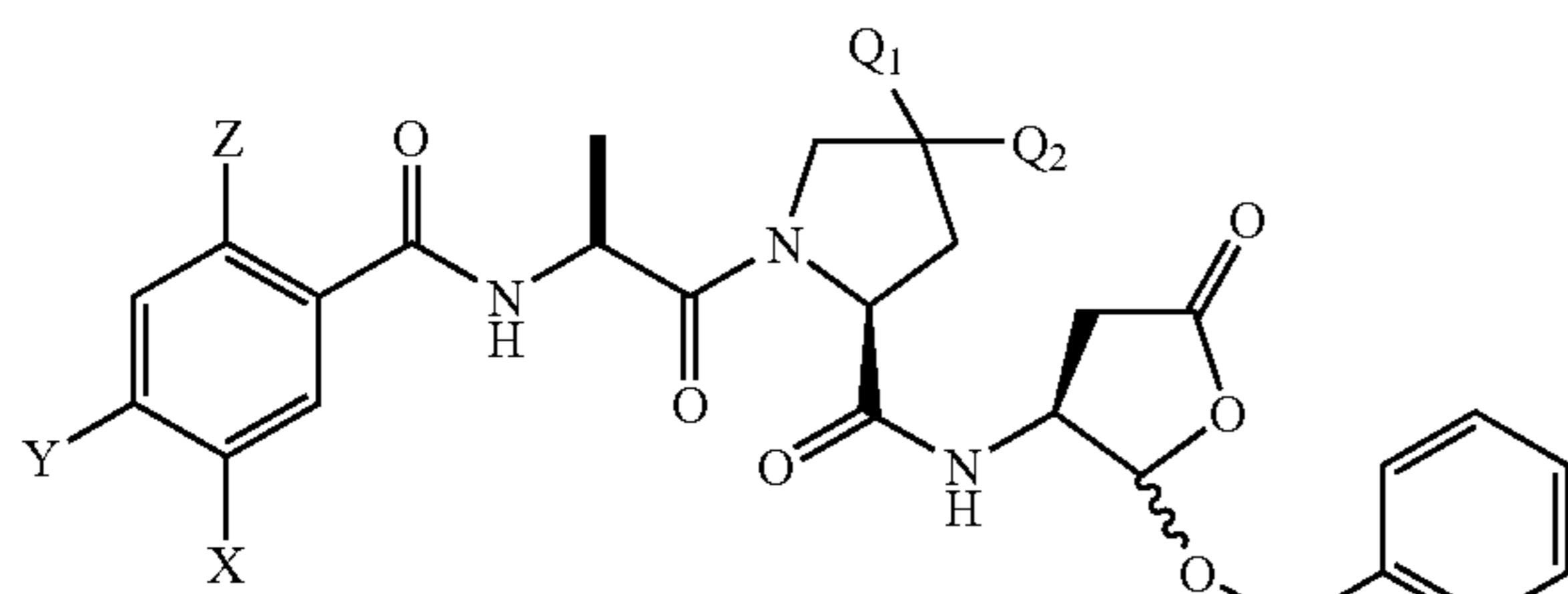
Scheme XXV
