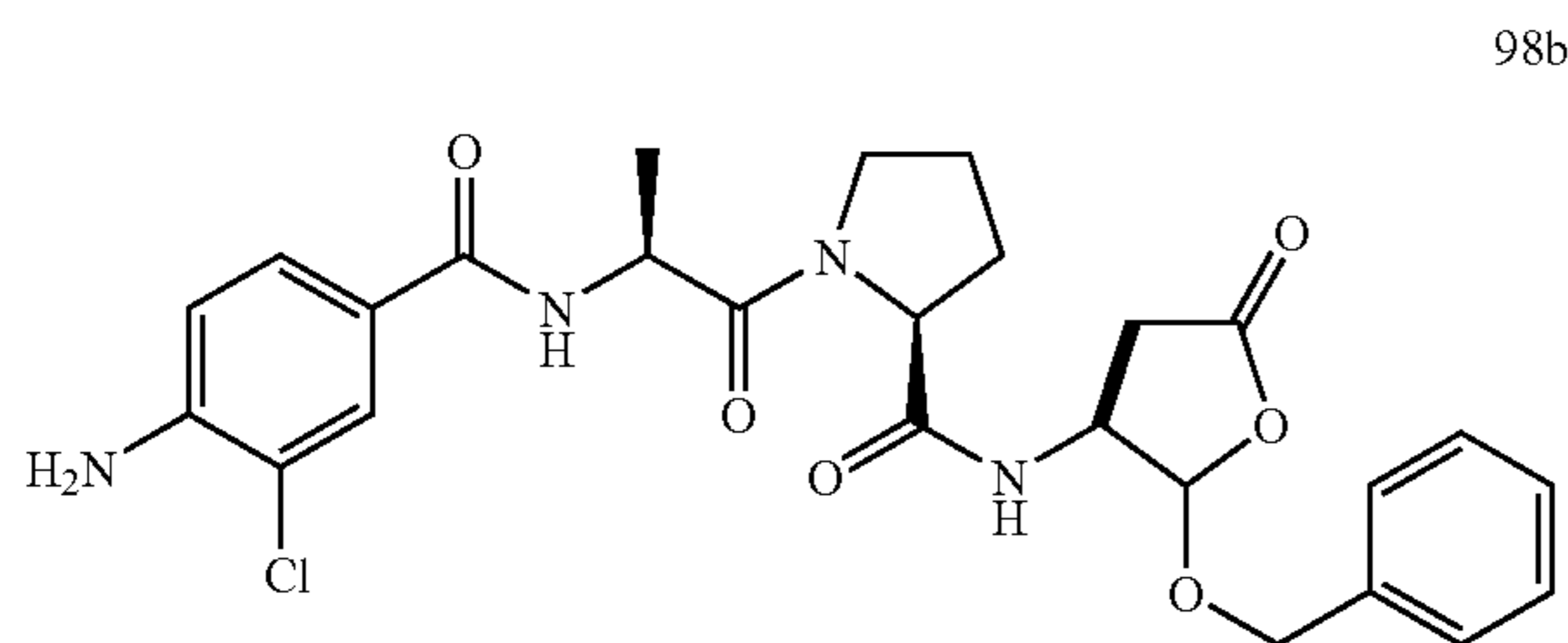
1-[2-(4-Amino-3-chloro-benzoylamino)-propionyl]-pyrrolidine-2-carboxylic acid (2-benzyloxy-5-oxo-tetrahydro-furan-3-yl)-amide (98b)
