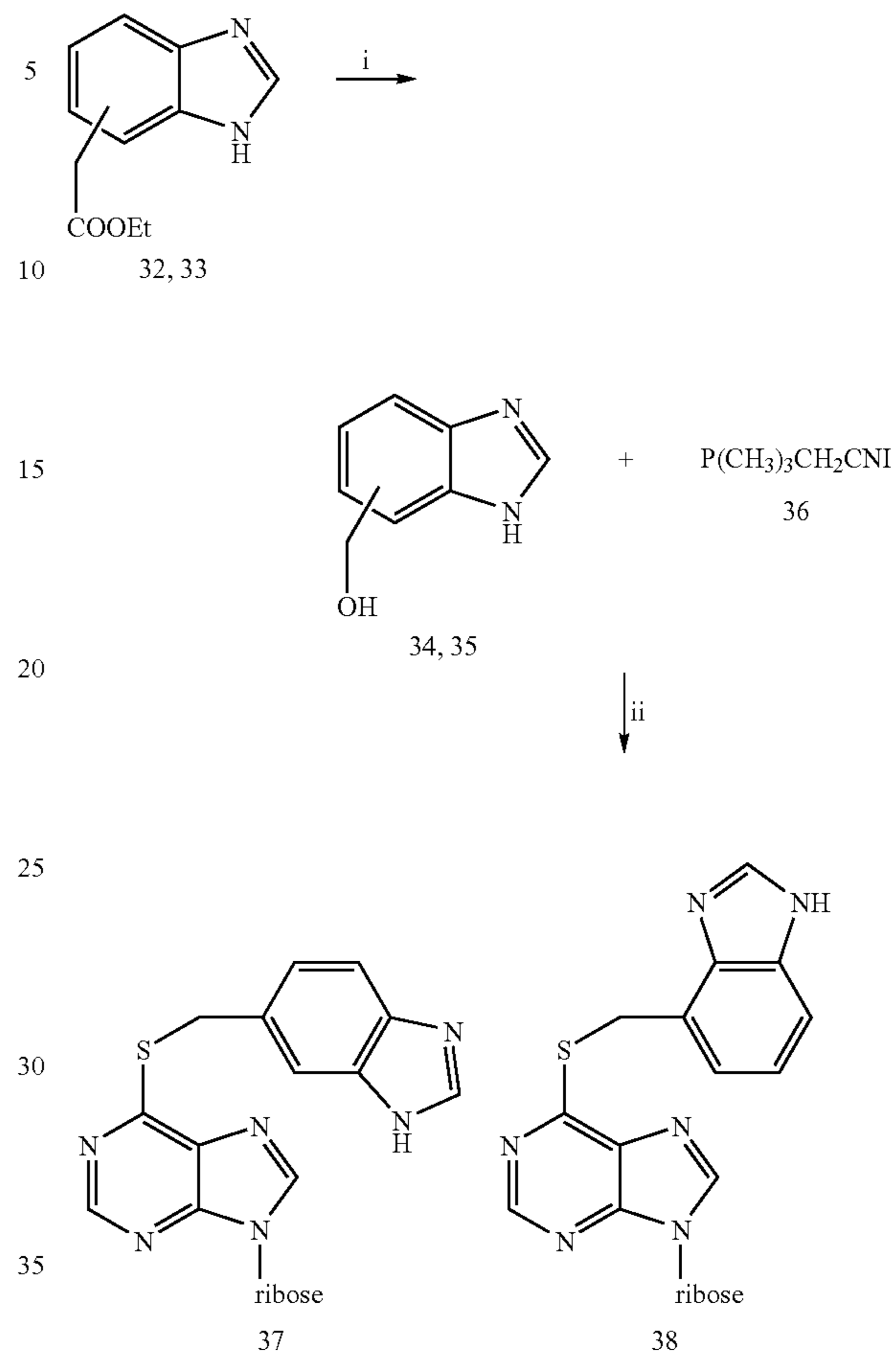
Scheme 4. Preparation of Benzimidazole Analogs.
