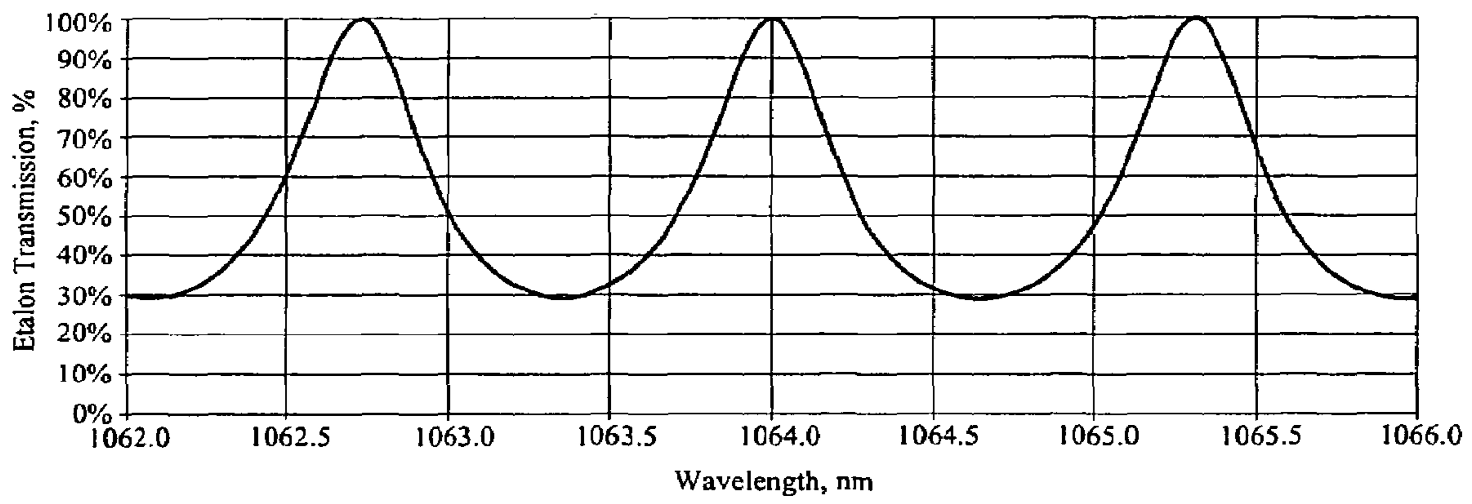
FIG. 15 (Prior Art)
