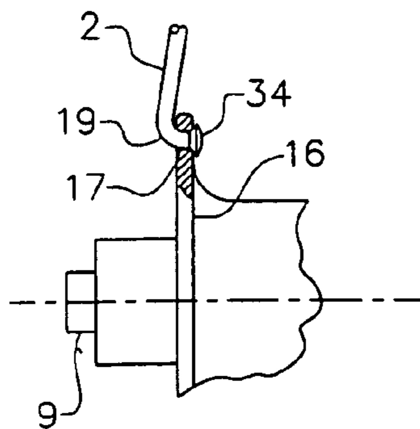
Fig. 2c Prior Art
