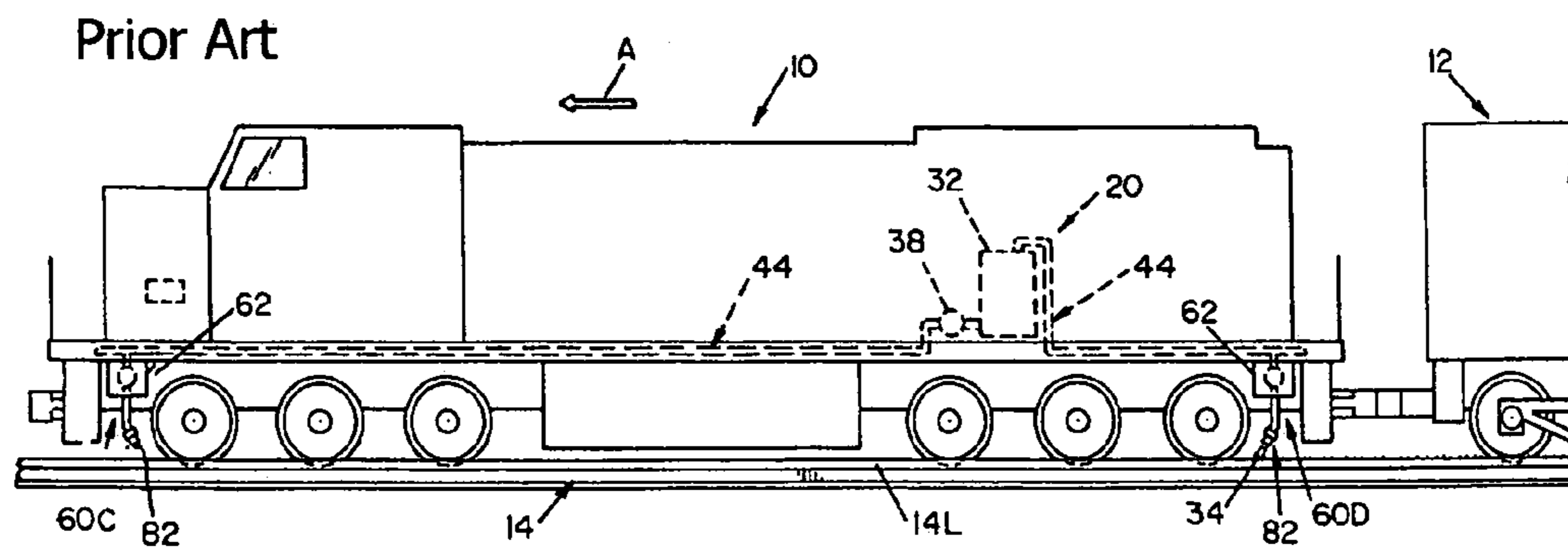
Figure 1, Prior Art
