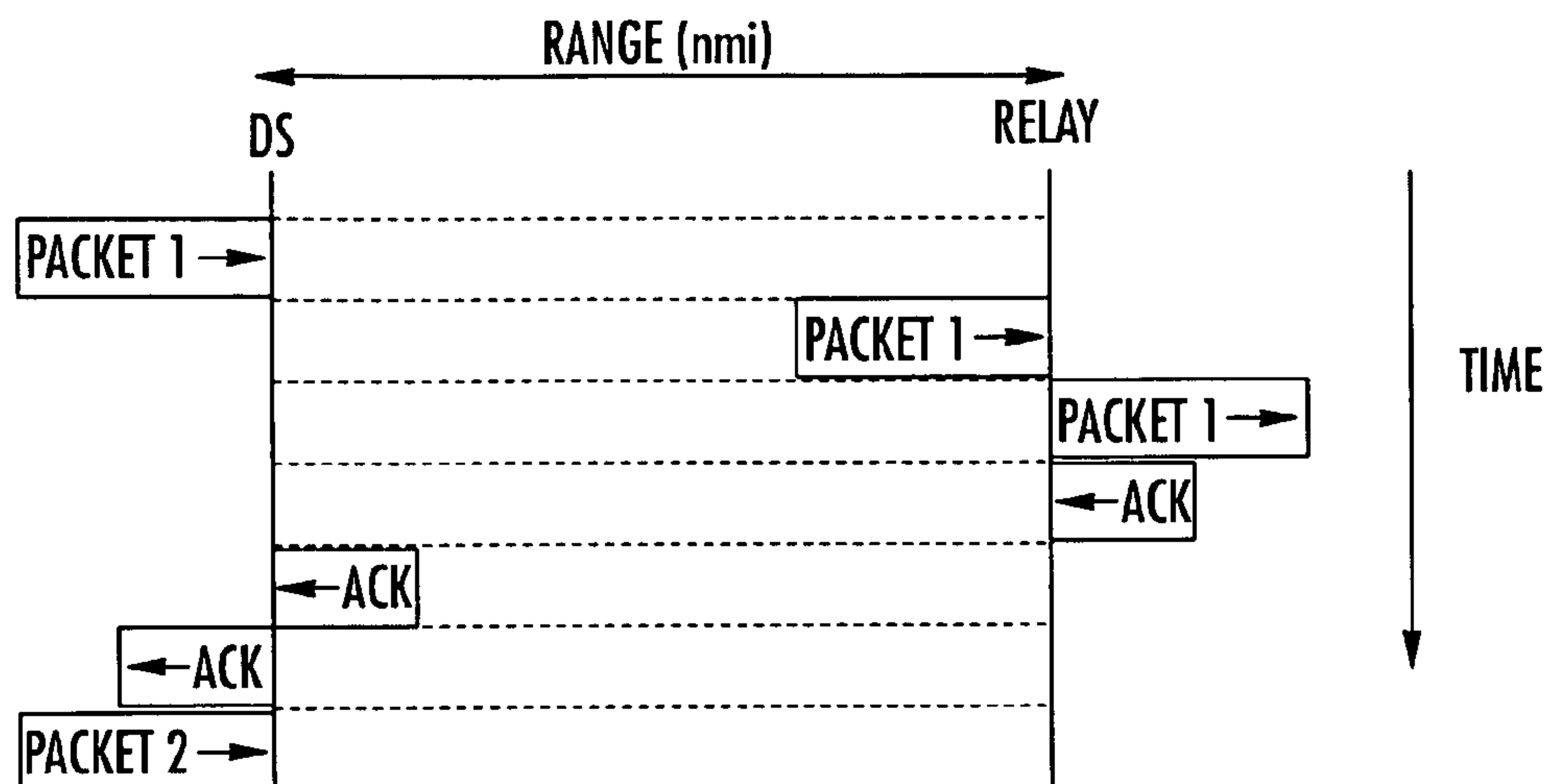
FIG. 1 (PRIOR ART)
