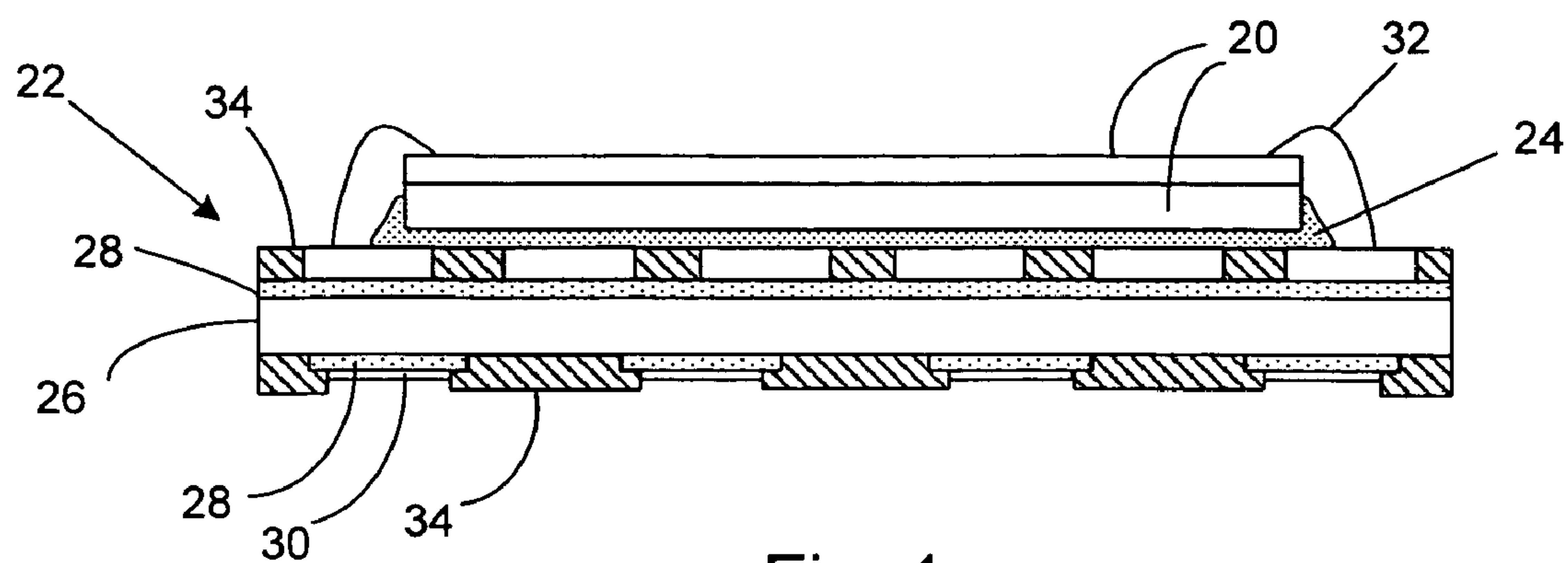
Fig. 1 (Prior Art)
