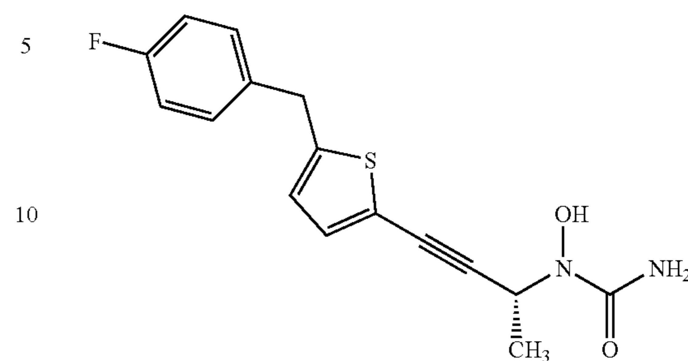
ABT-761
