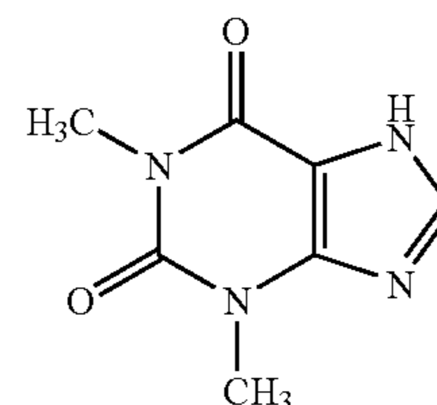
Theophylline
