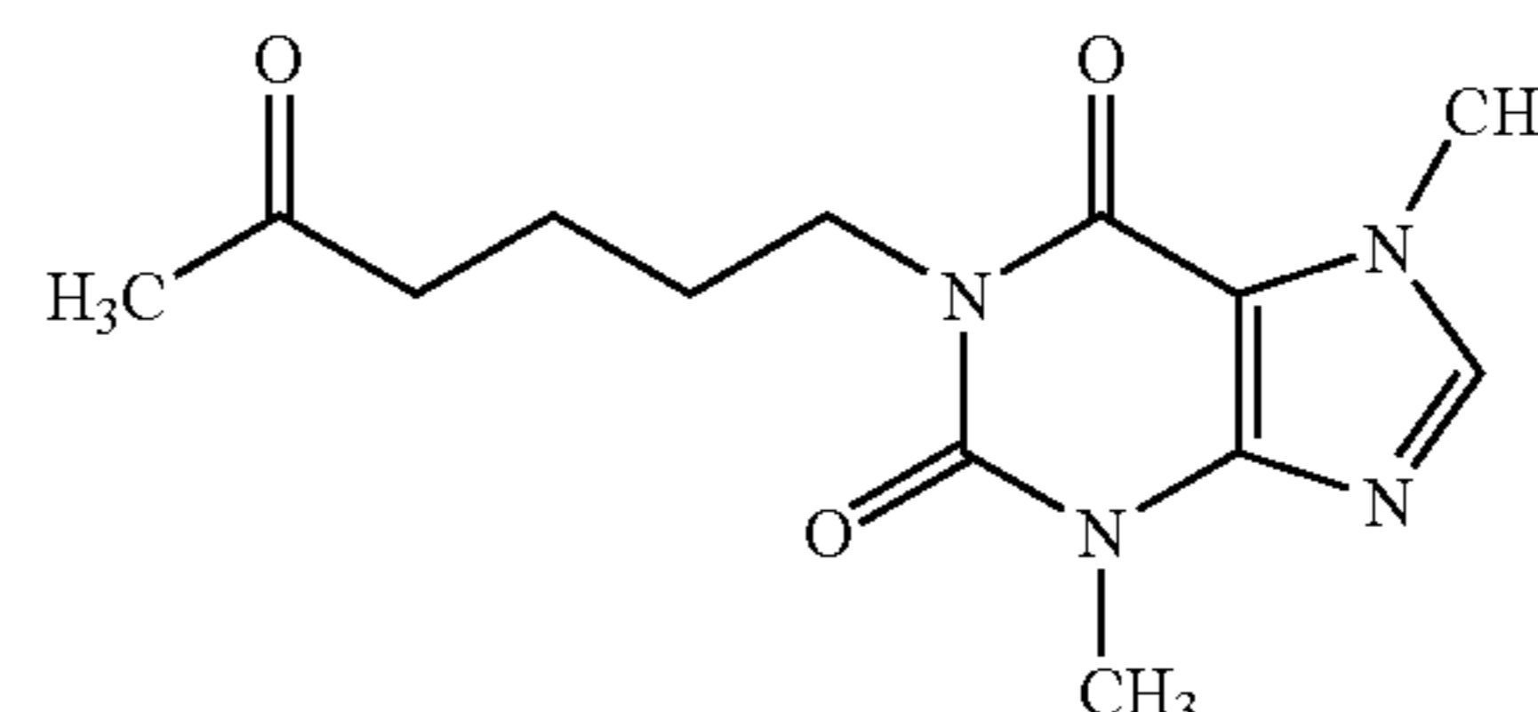
Pentoxifylline
