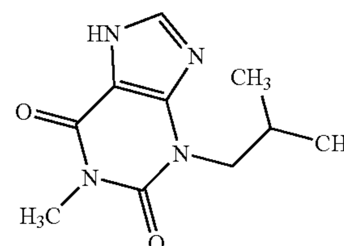
IBMX
