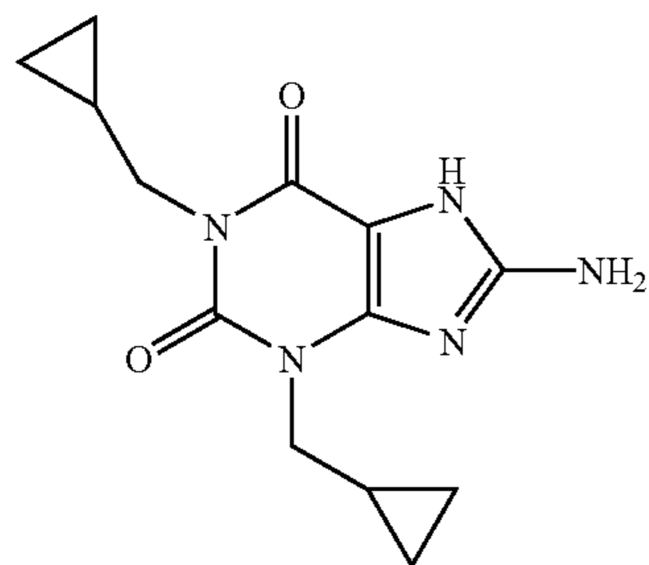
Cipamfylline (BRL-61,063)
