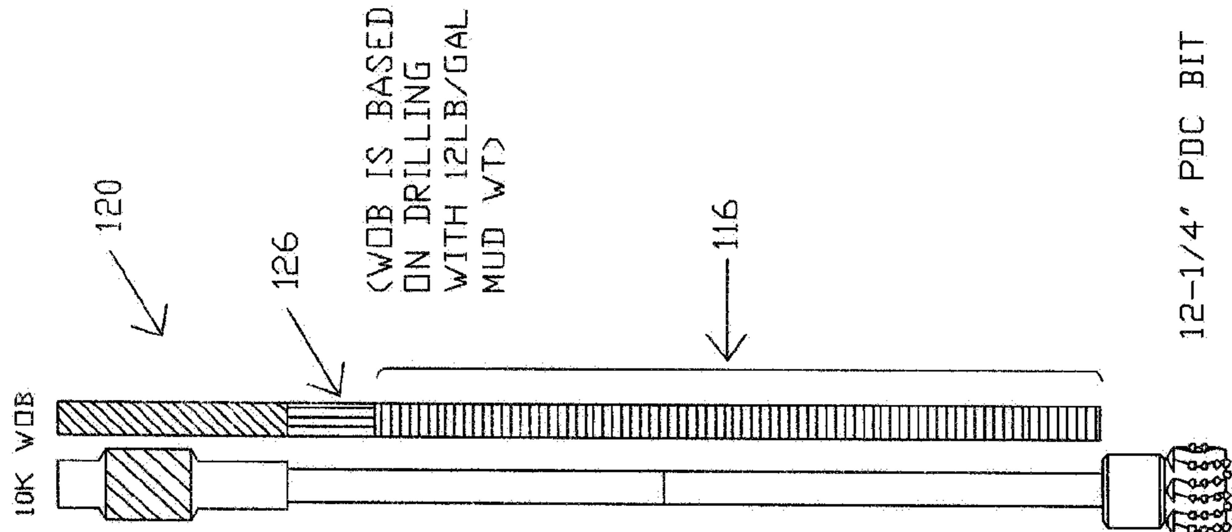
FIG. 5C (PRIOR ART)
