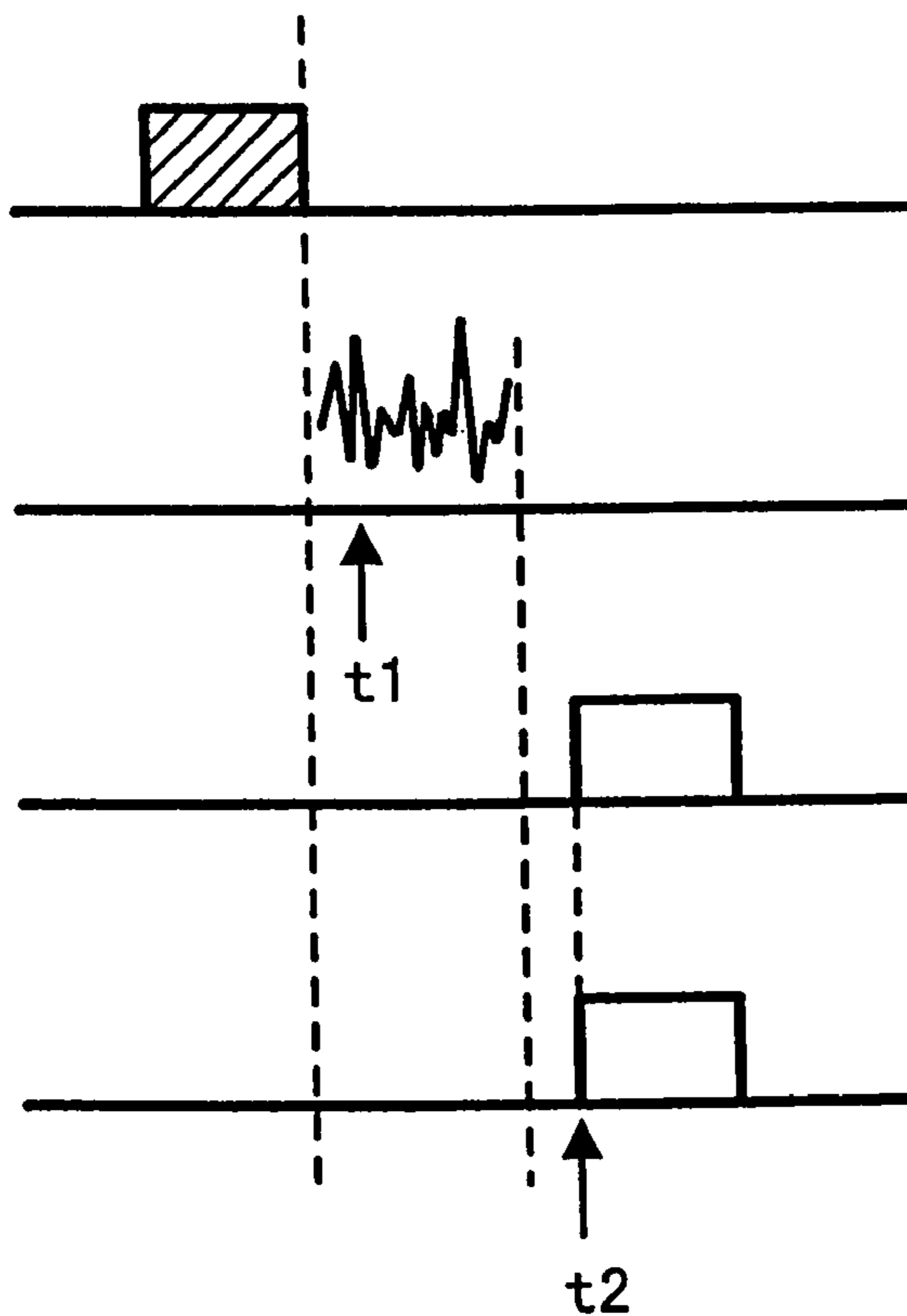
FIG. 10B DISTURBING SIGNAL SUCH AS EXTERNAL NOISE
