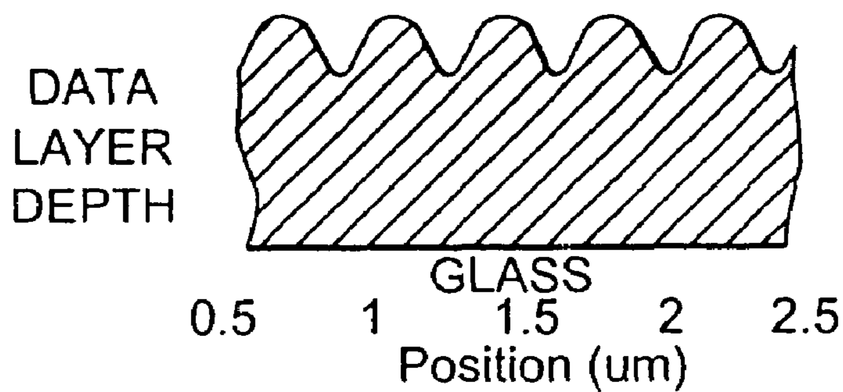
FIG. 1 PRIOR ART
