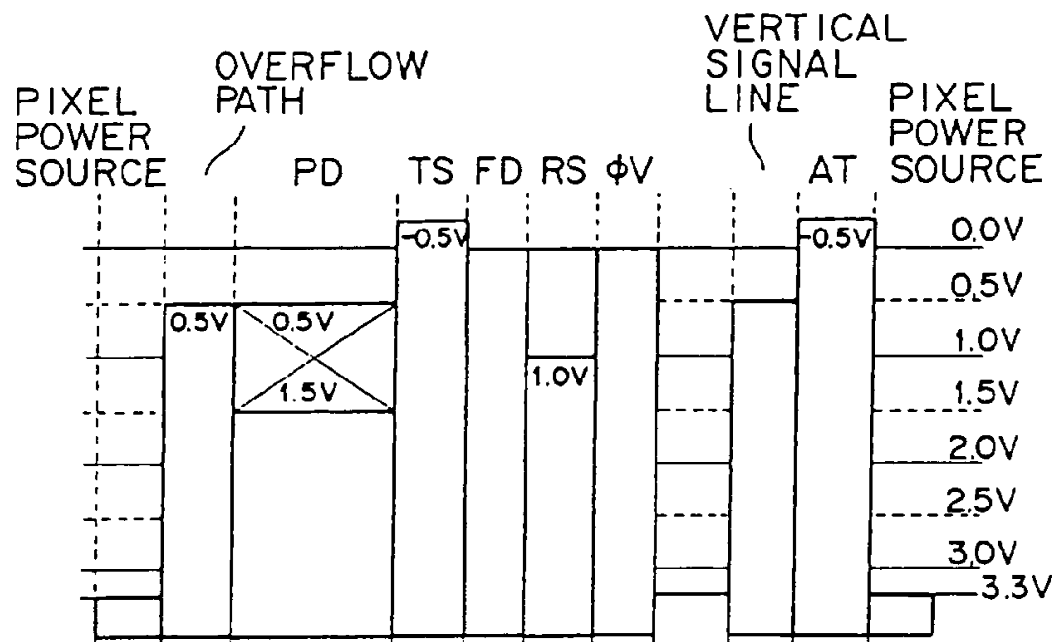
FIG. 4A t < t_1 NON-SELECTION STATE
