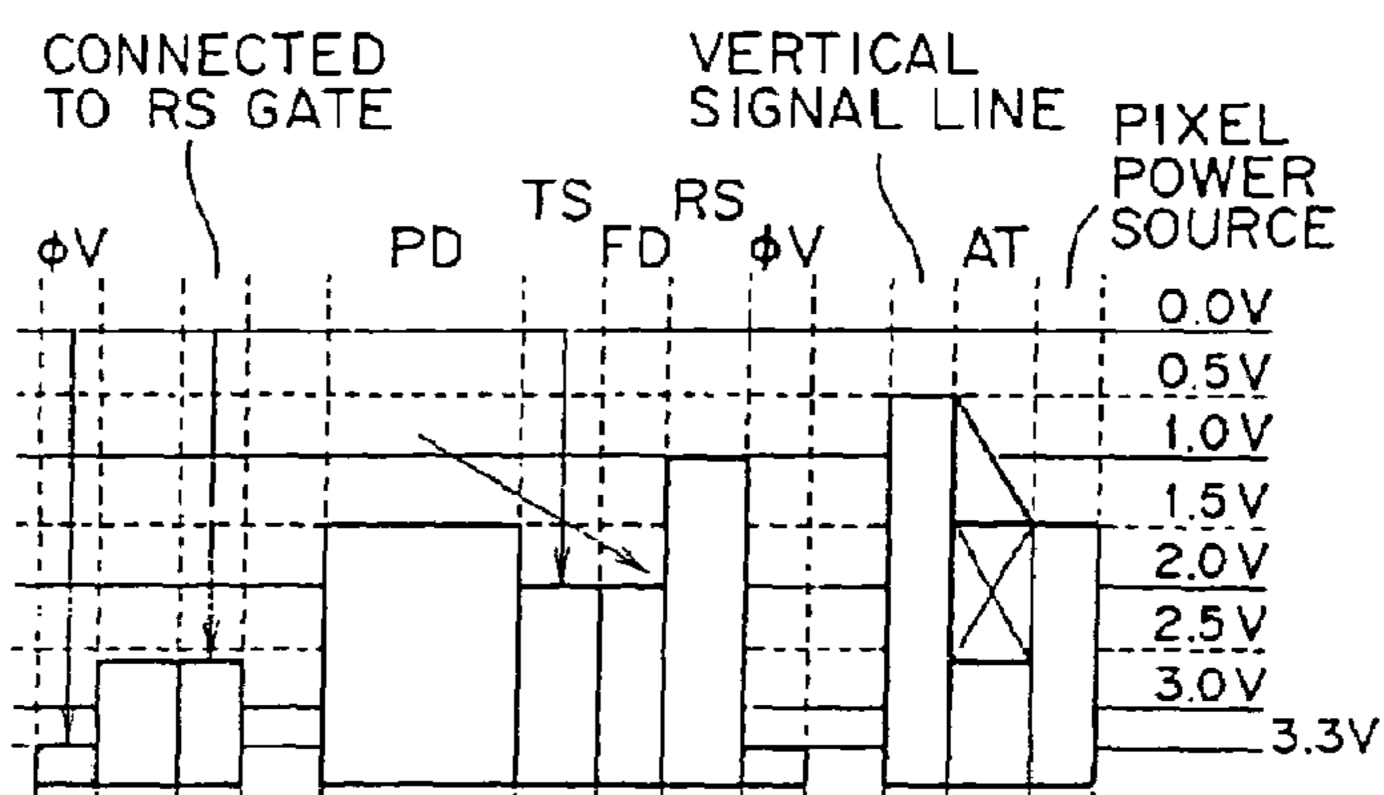
FIG. 14A t_{14} < t < t_{15} TRANSFER OF STORED CHARGES FROM PD TO FD
