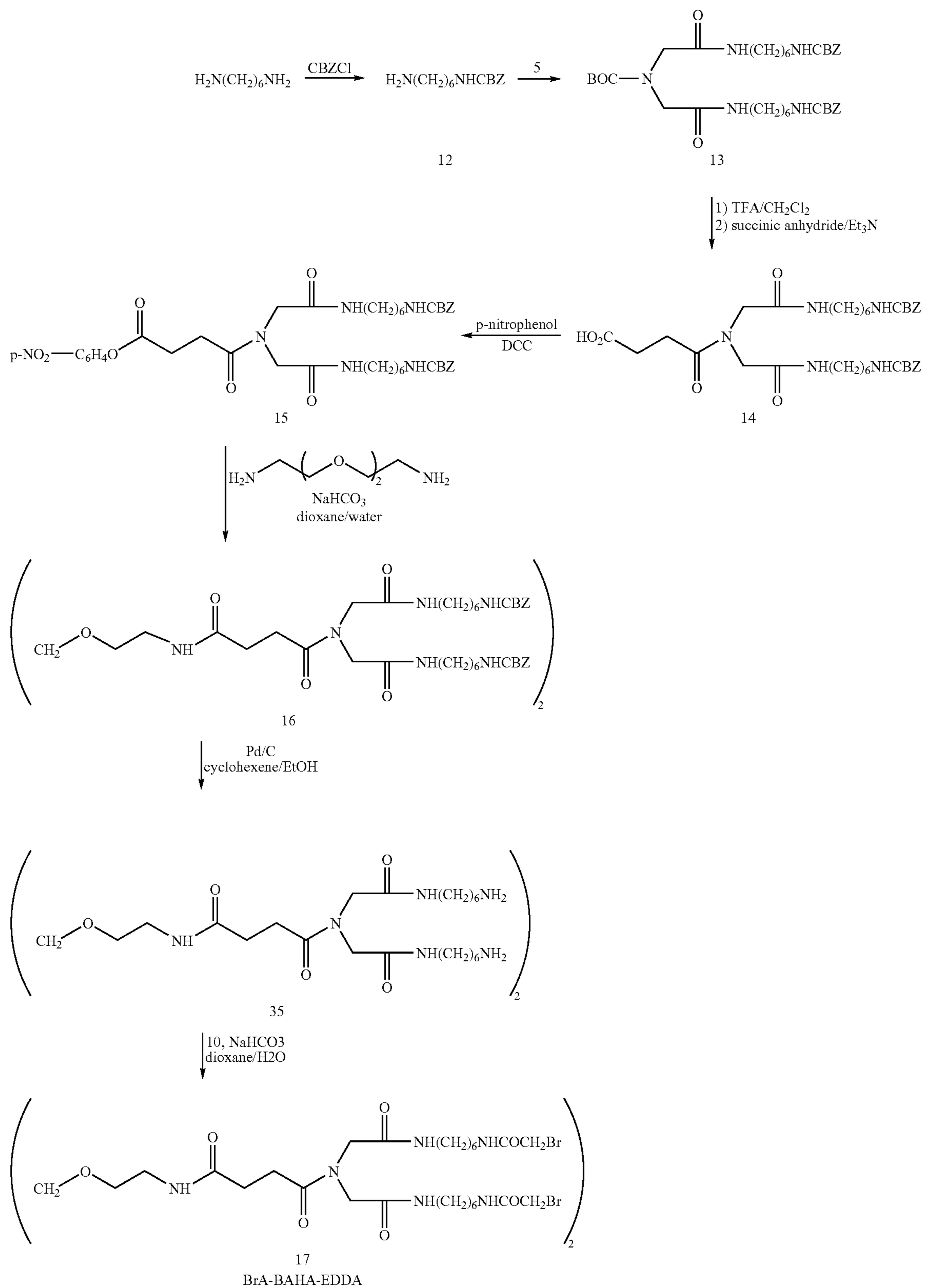
Reaction Scheme 3
