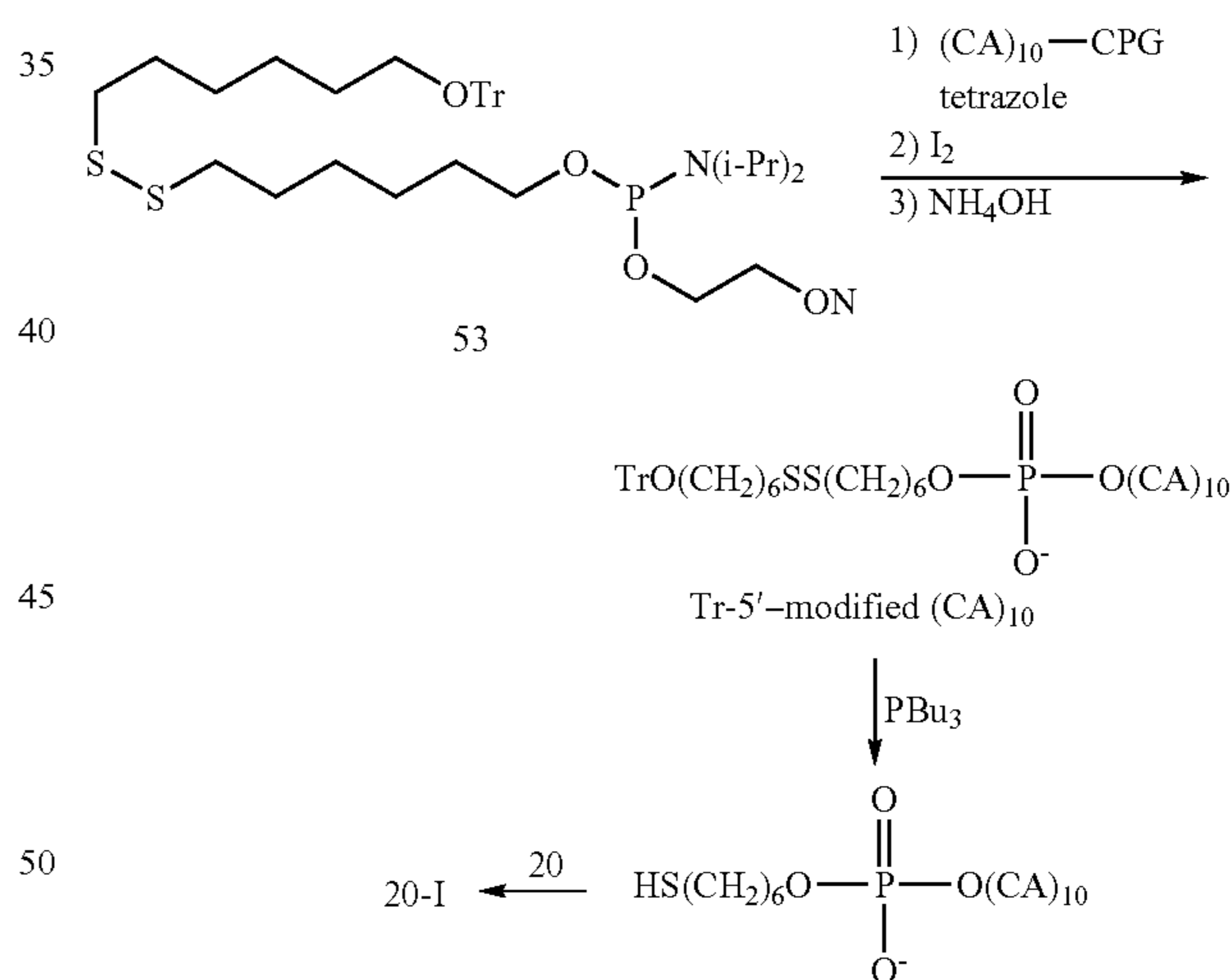
Reaction Scheme 22
