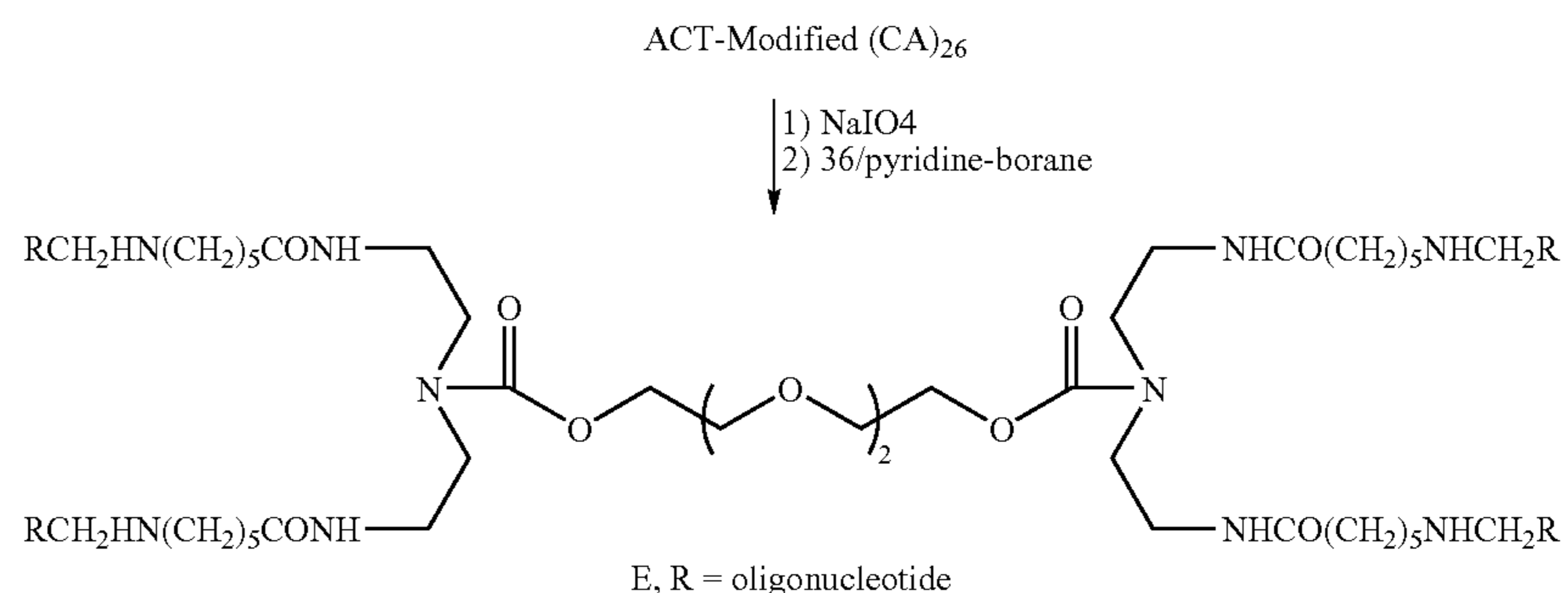
Reaction Scheme 16
