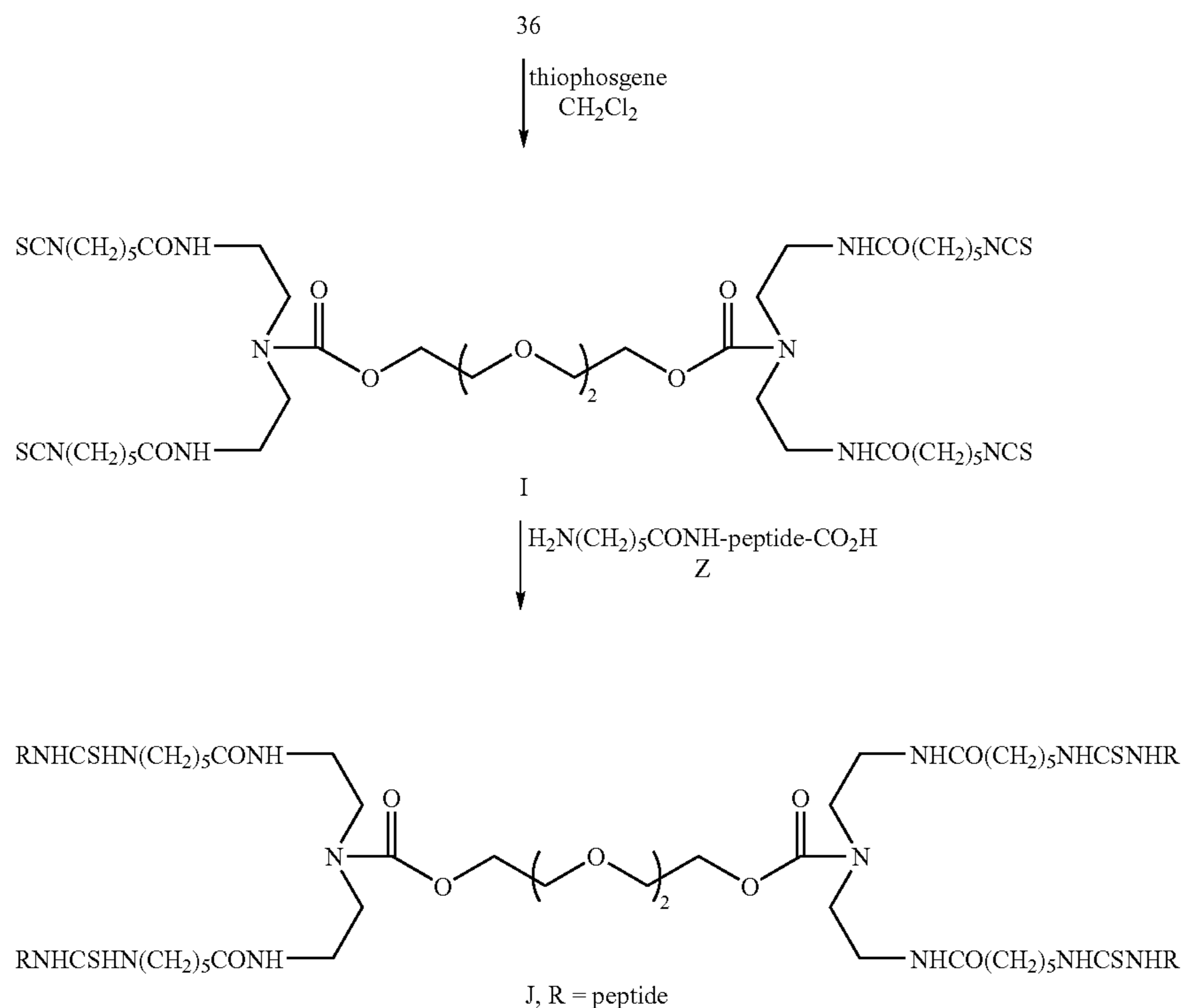
Reaction Scheme 18
