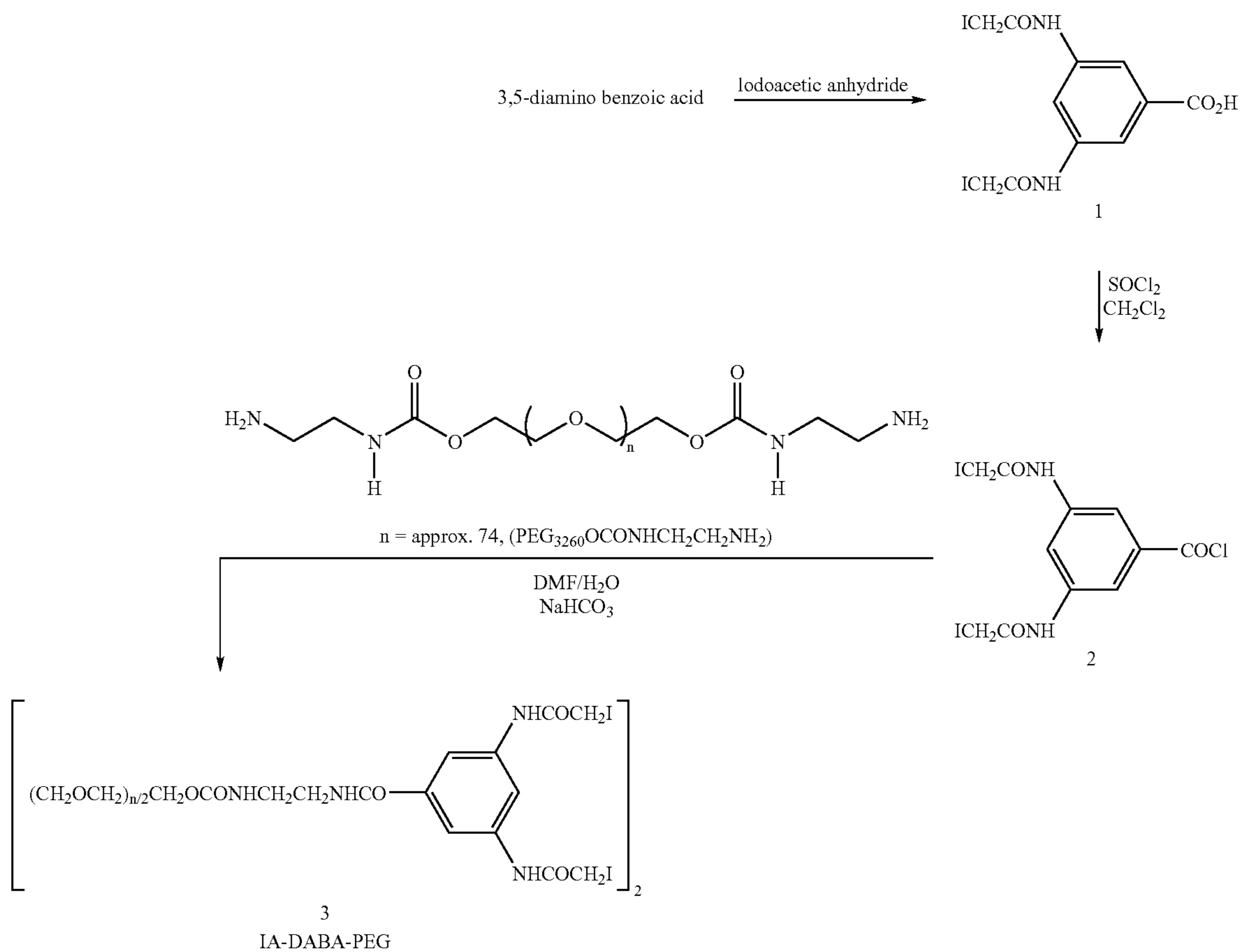
Reaction Scheme 1
