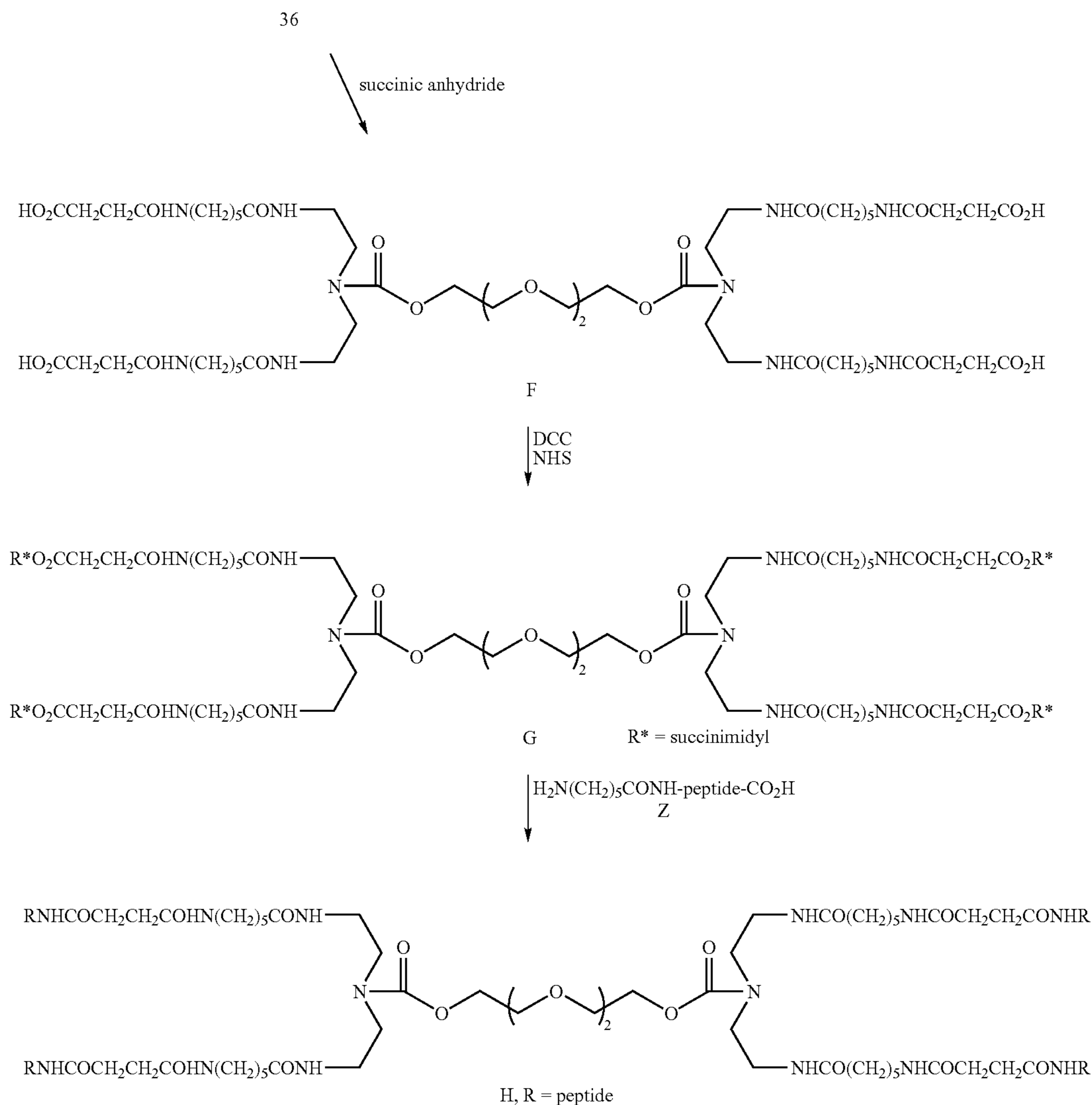
Reaction Scheme 17
