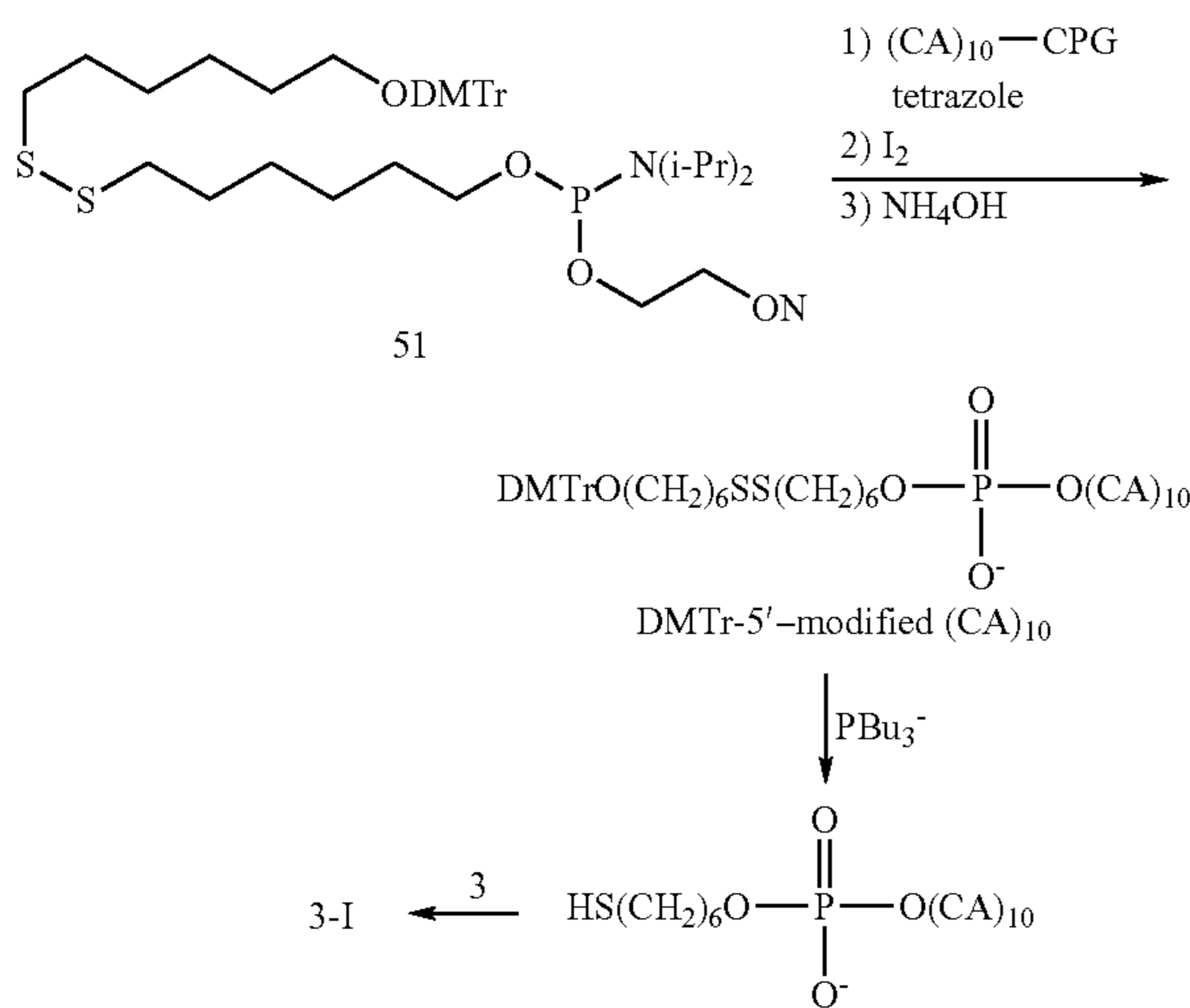
Reaction Scheme 21
