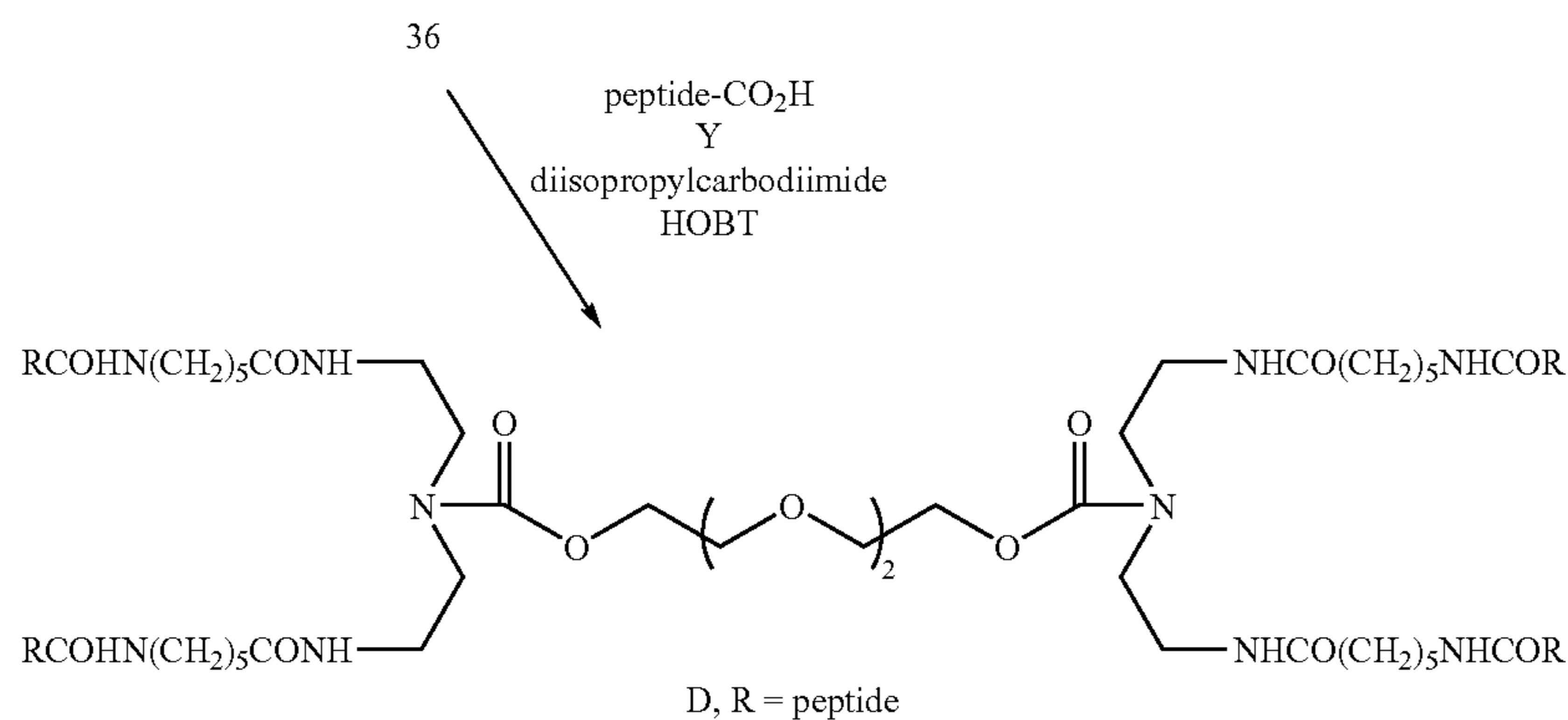
Reaction Scheme 15
