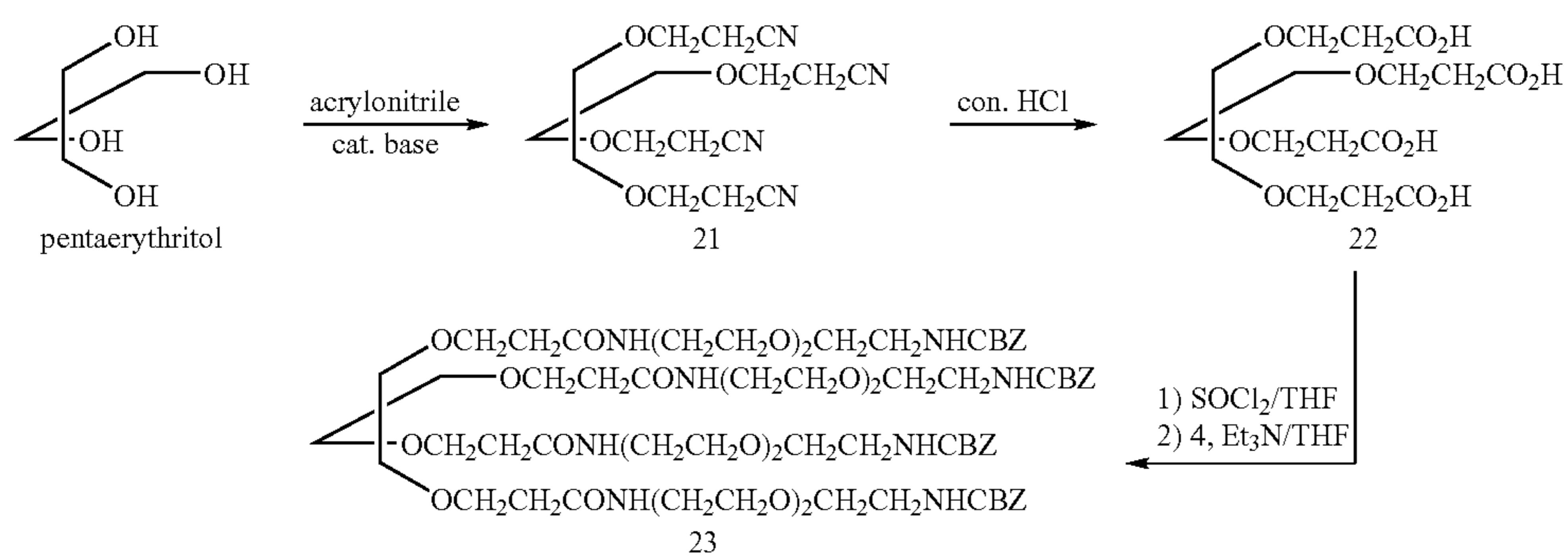
Reaction Scheme 5
