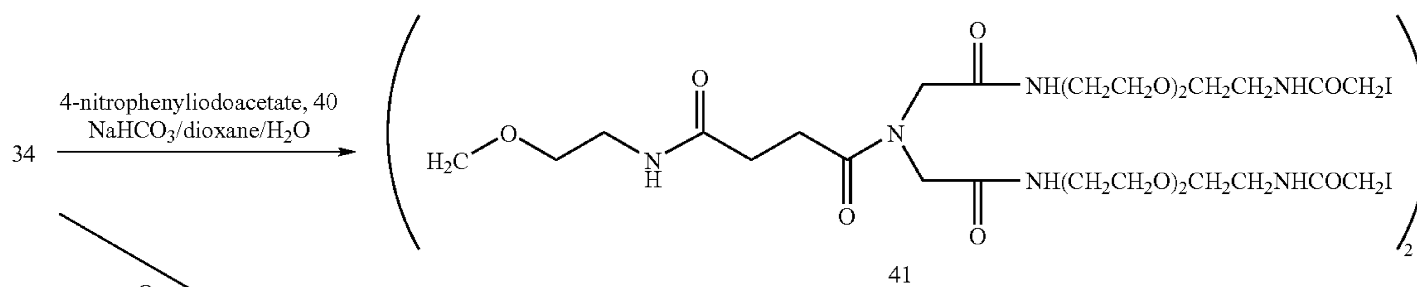
Reaction Scheme 9
