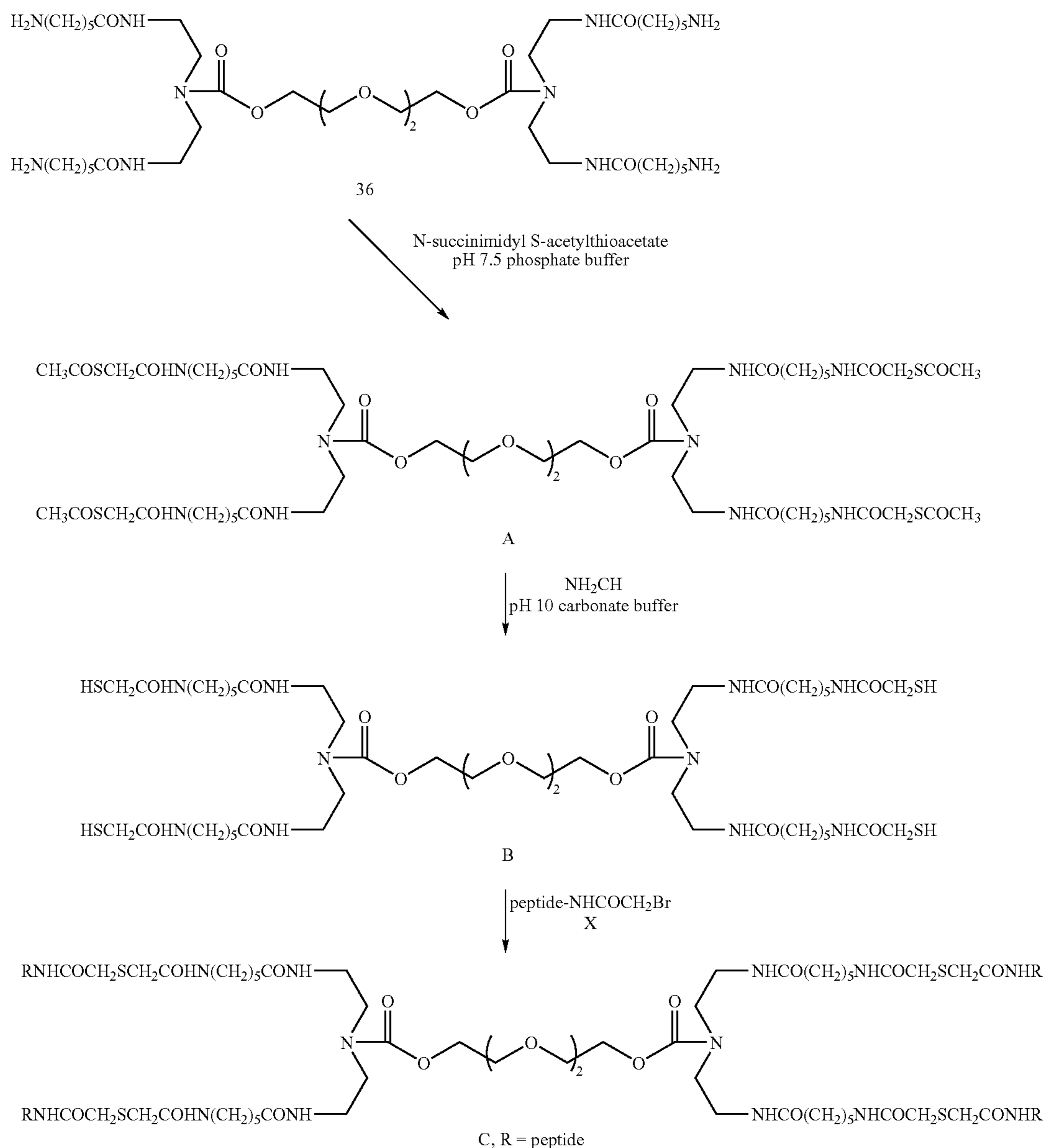
Reaction Scheme 14
