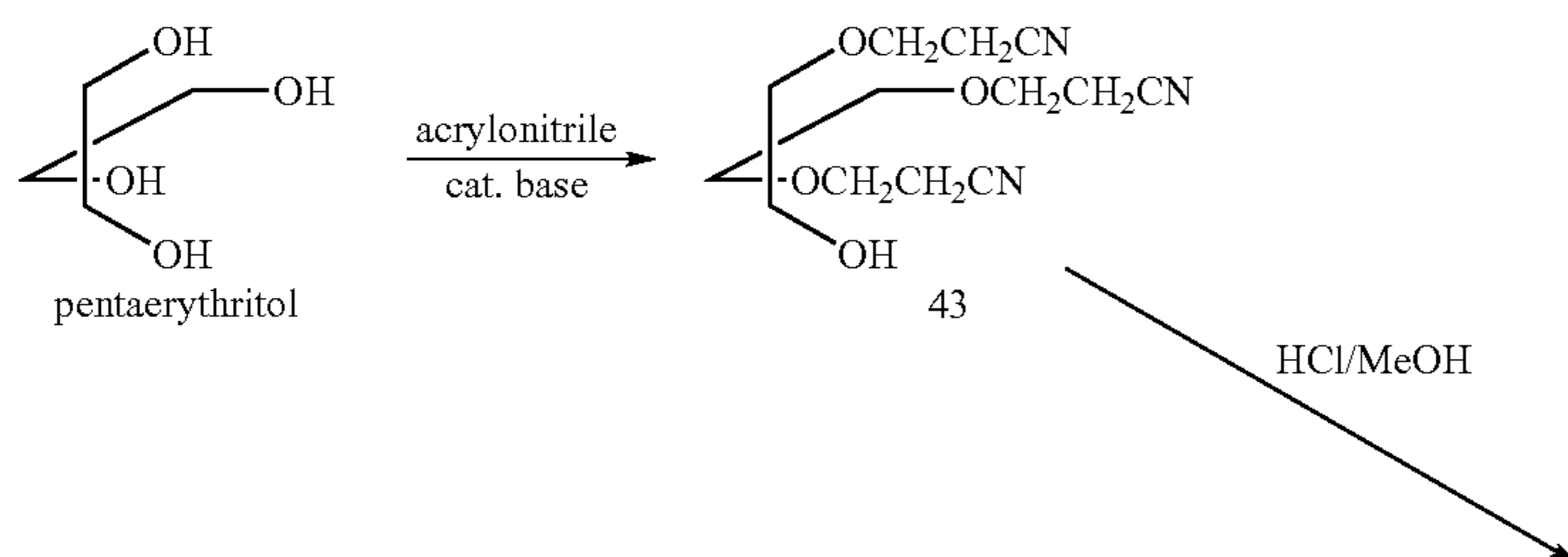
Reaction Scheme 10
