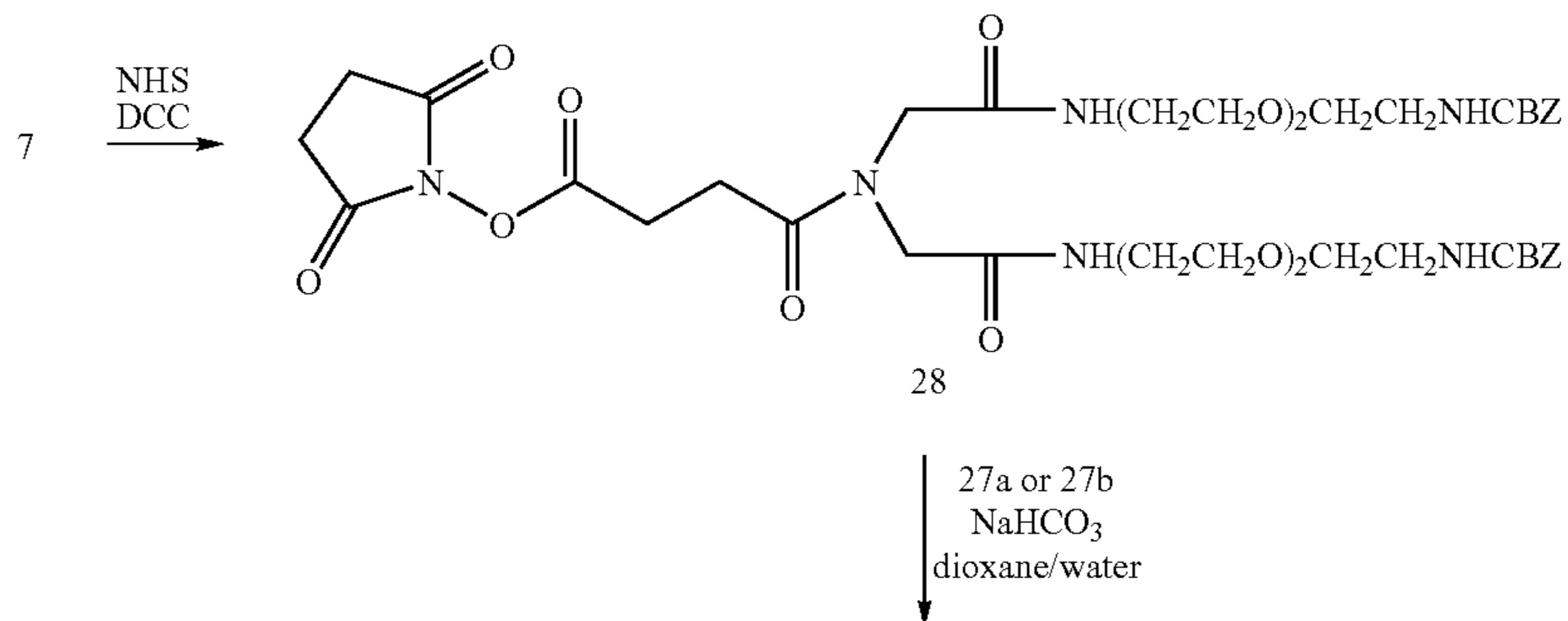
Reaction Scheme 7
