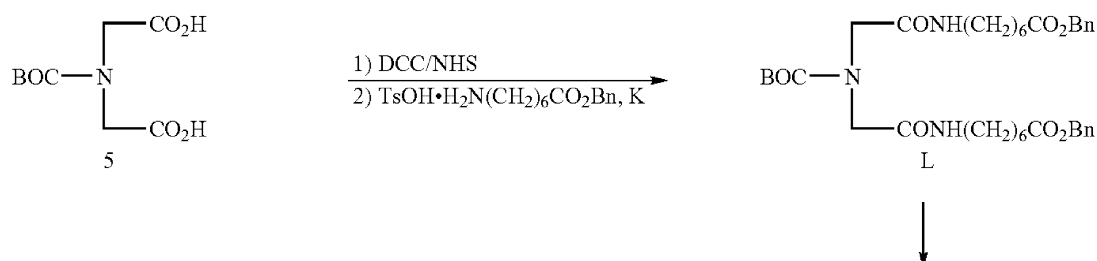
Reaction Scheme 20
