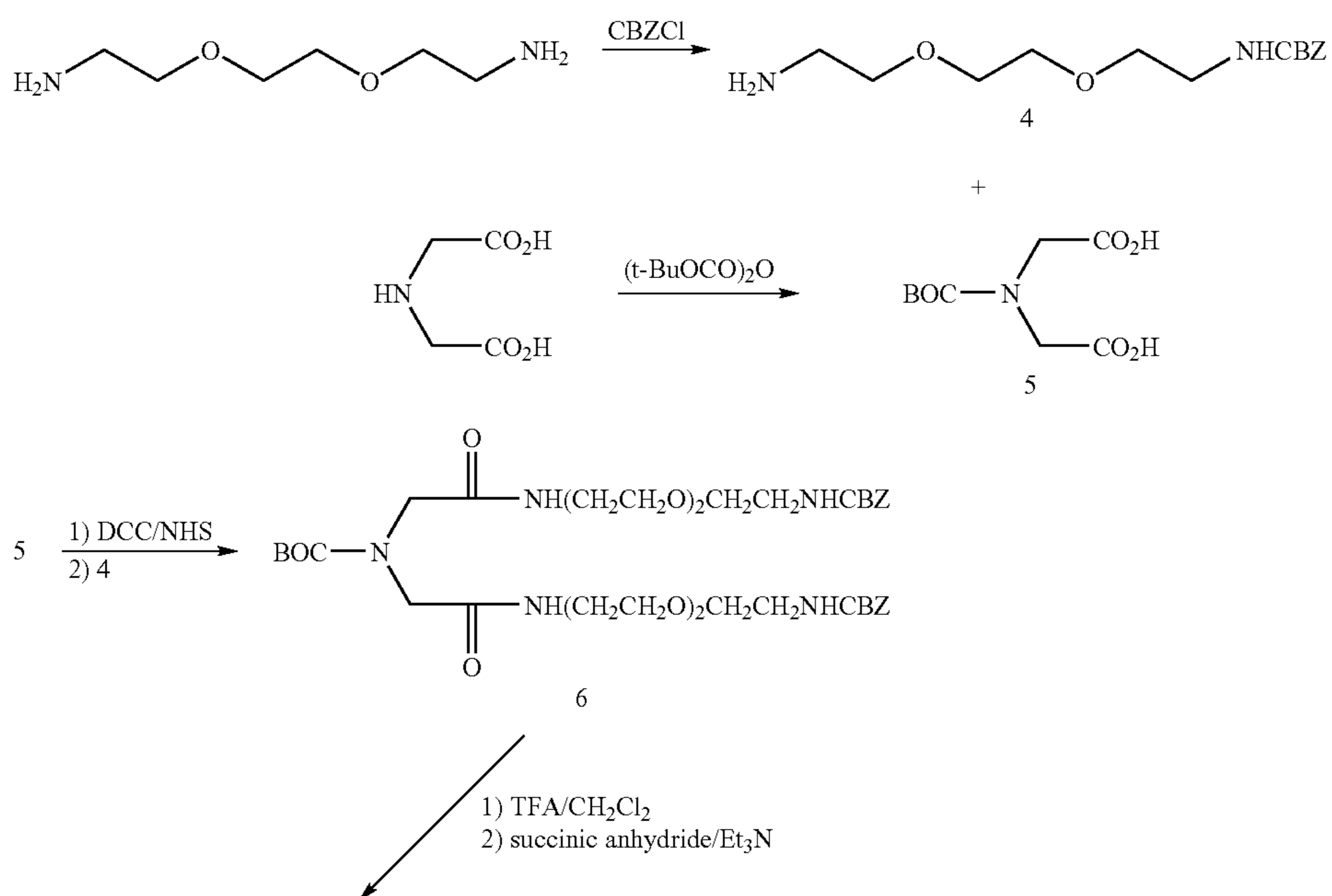
Reaction Scheme 2
