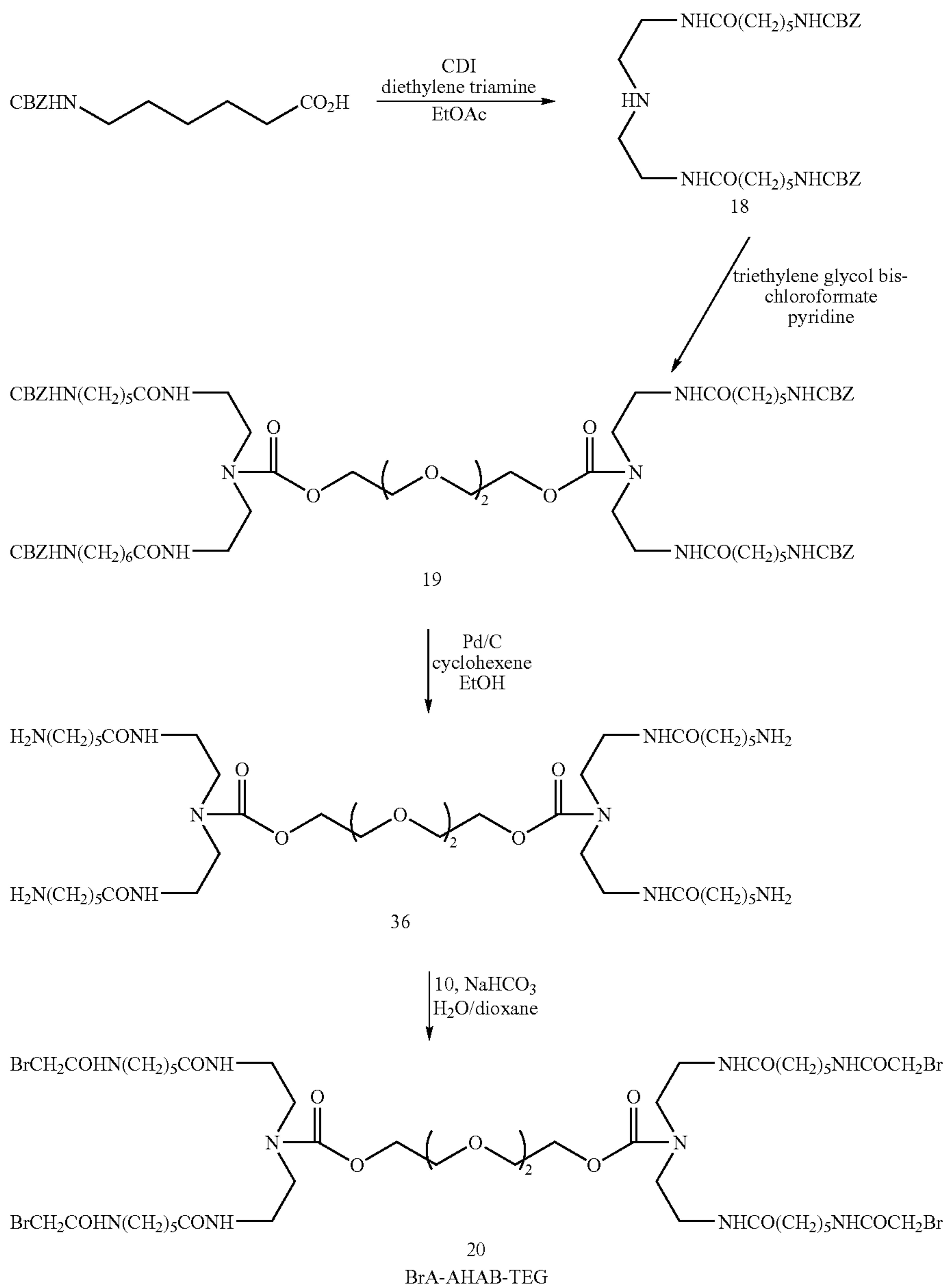
Reaction Scheme 4
