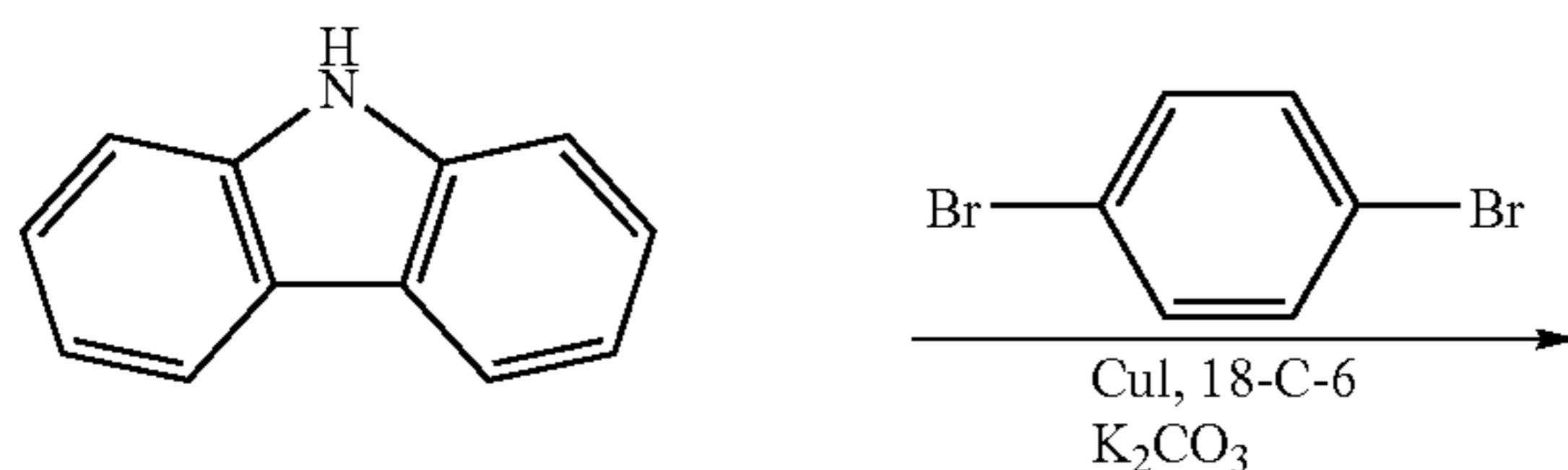
Reaction Scheme 3
