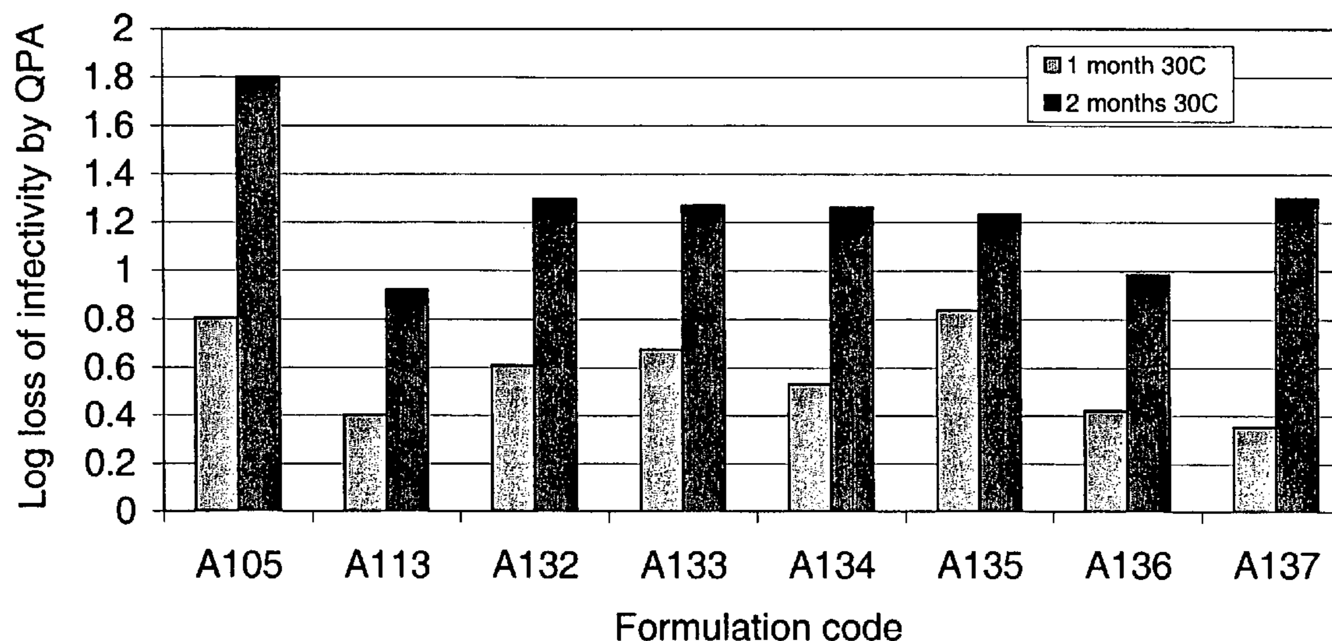
Effect of oxidation inhibitors on the stability of Ad5gag in A105
