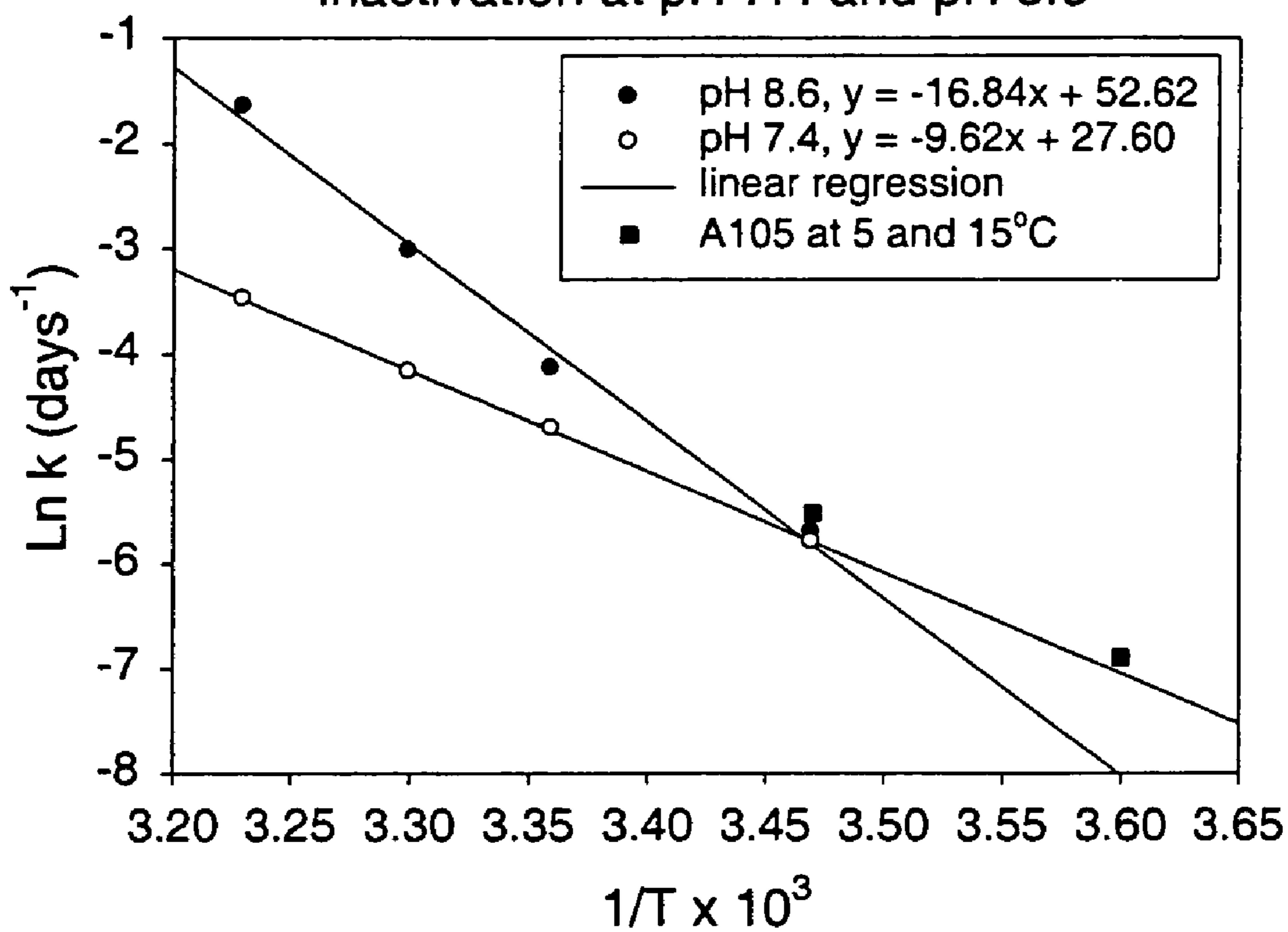
Figure 11. Arrhenius plot of Ad5gag inactivation at pH 7.4 and pH 8.6
