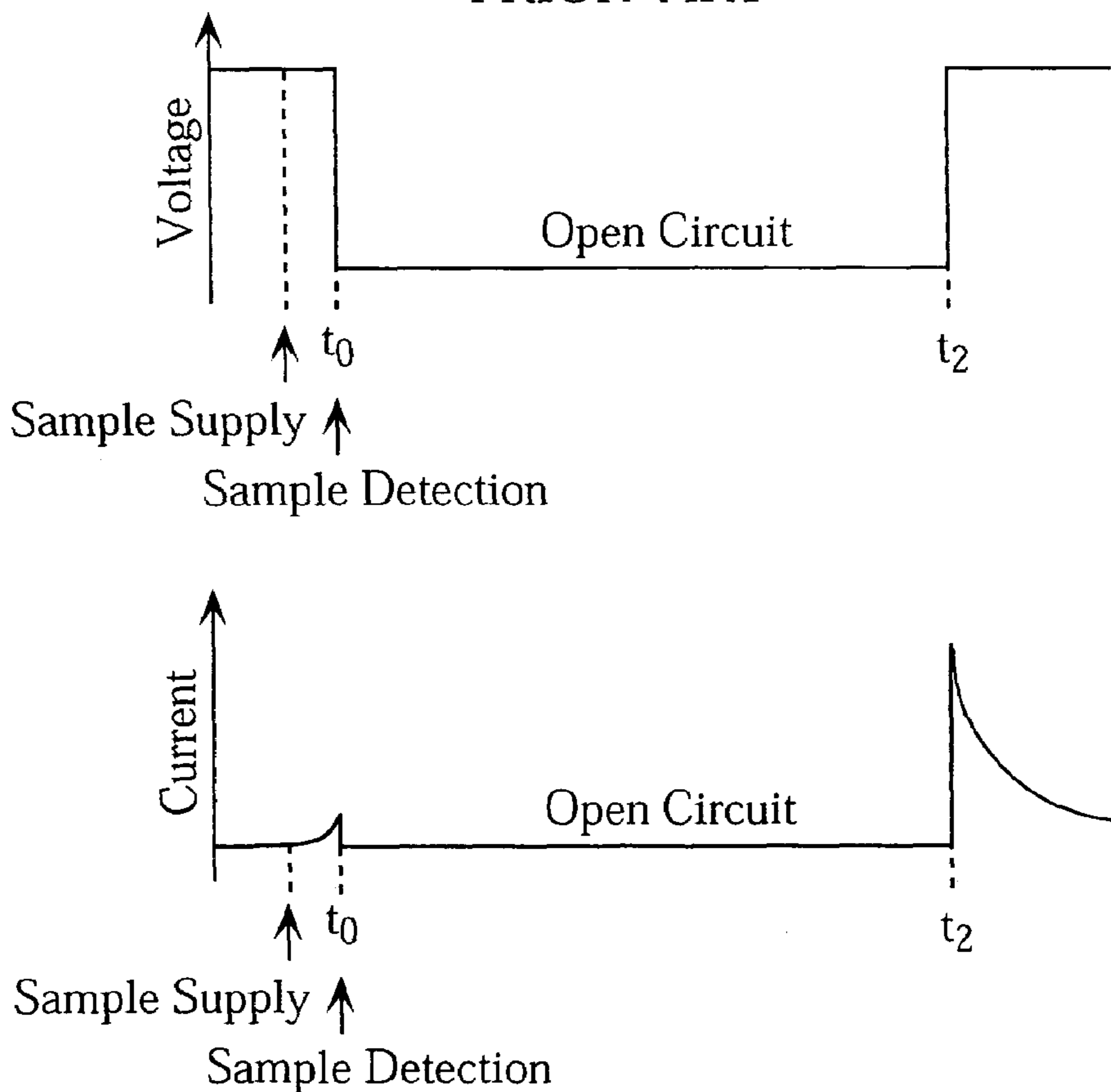
FIG.10 PRIOR ART
