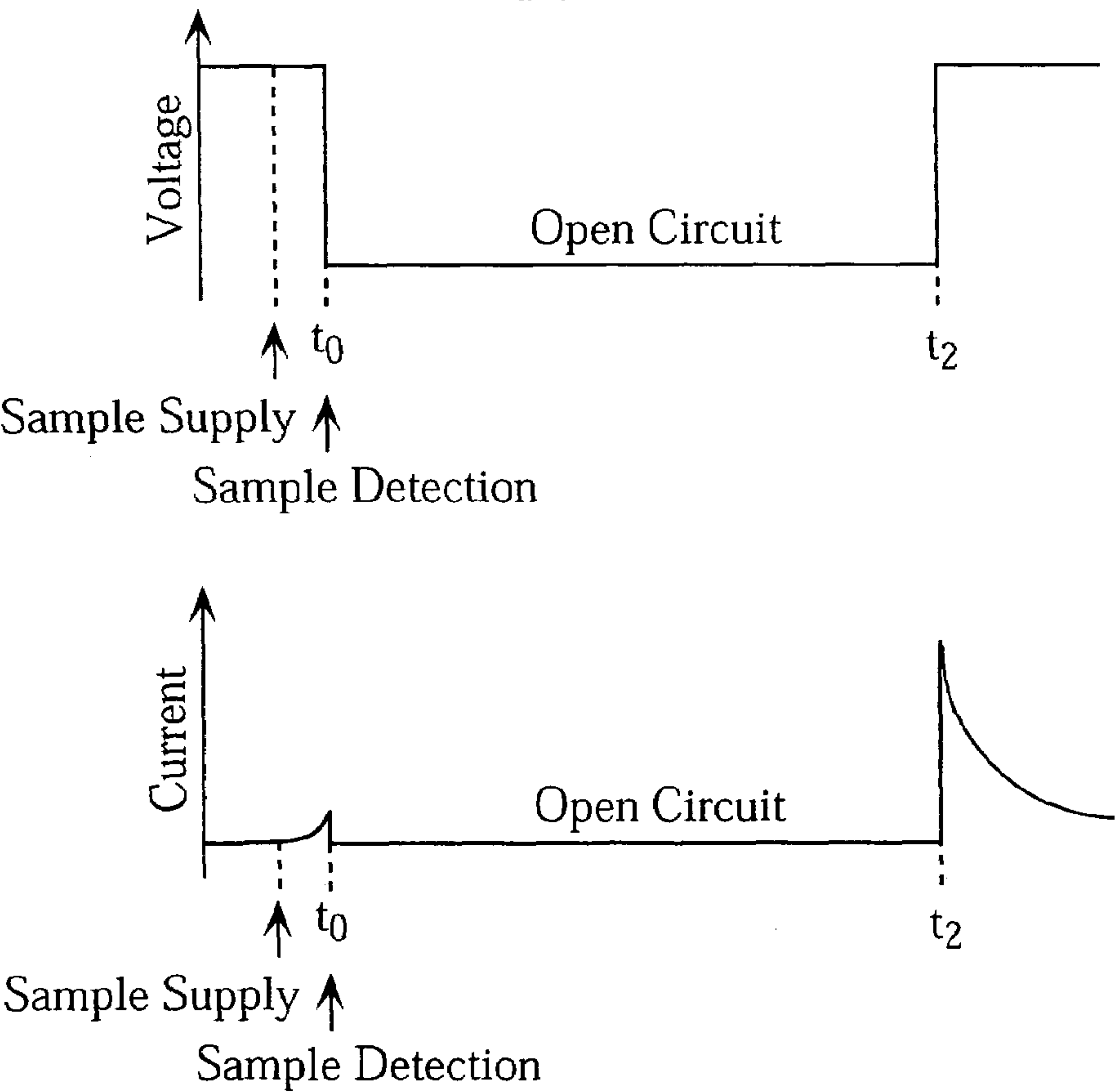
FIG.10 PRIOR ART
