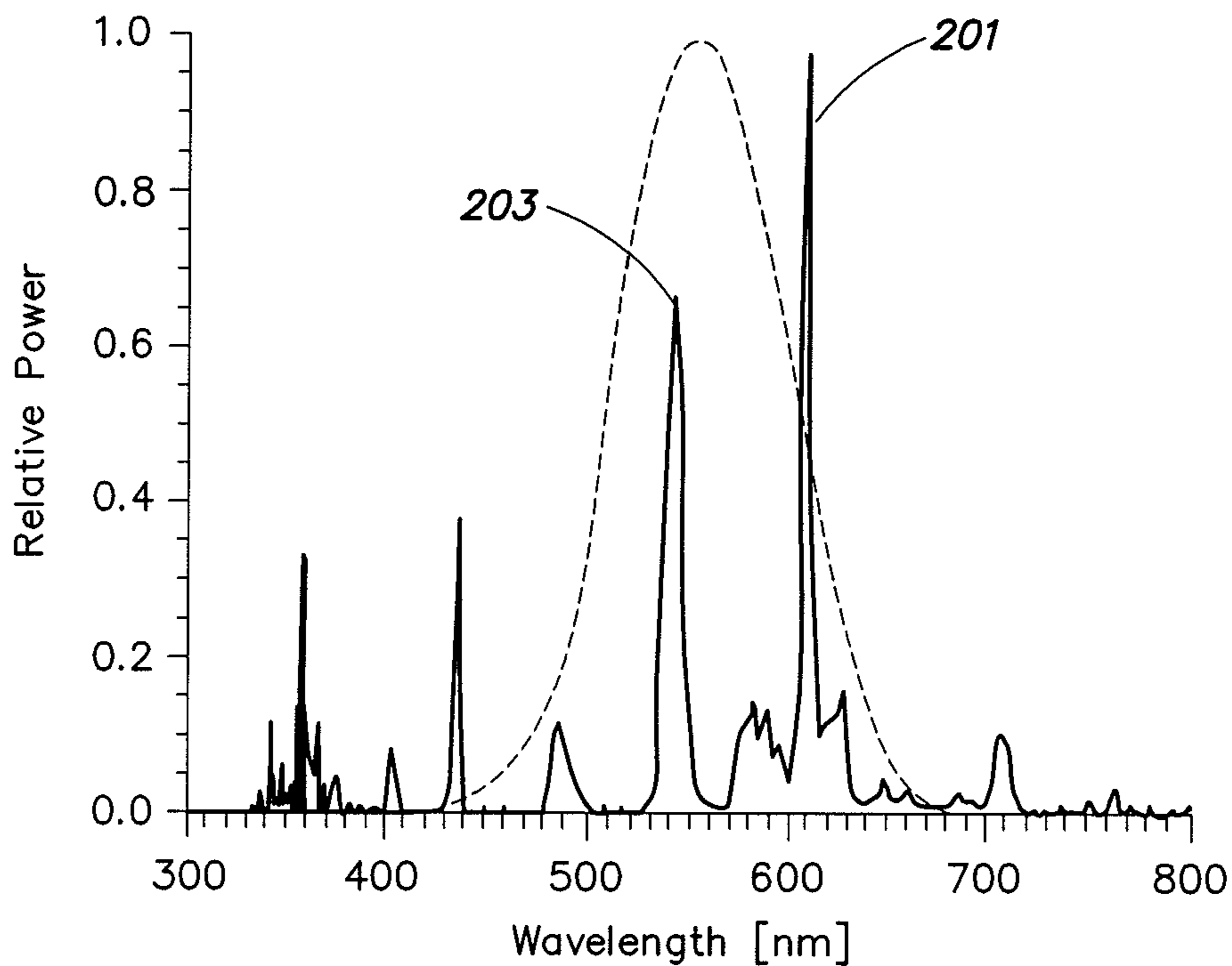
FIG. 27 (Prior Art)
