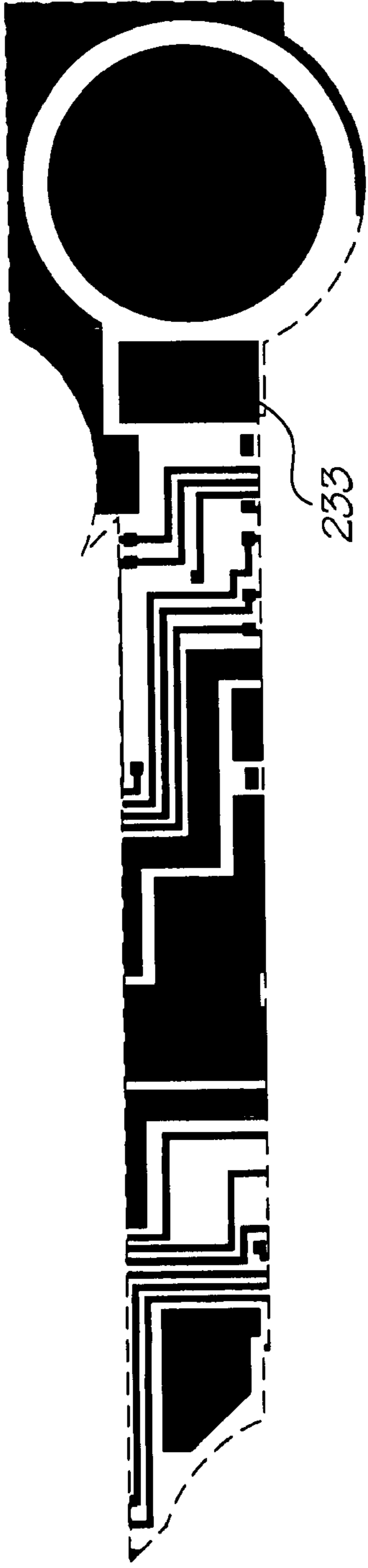
Metal 2 mask
