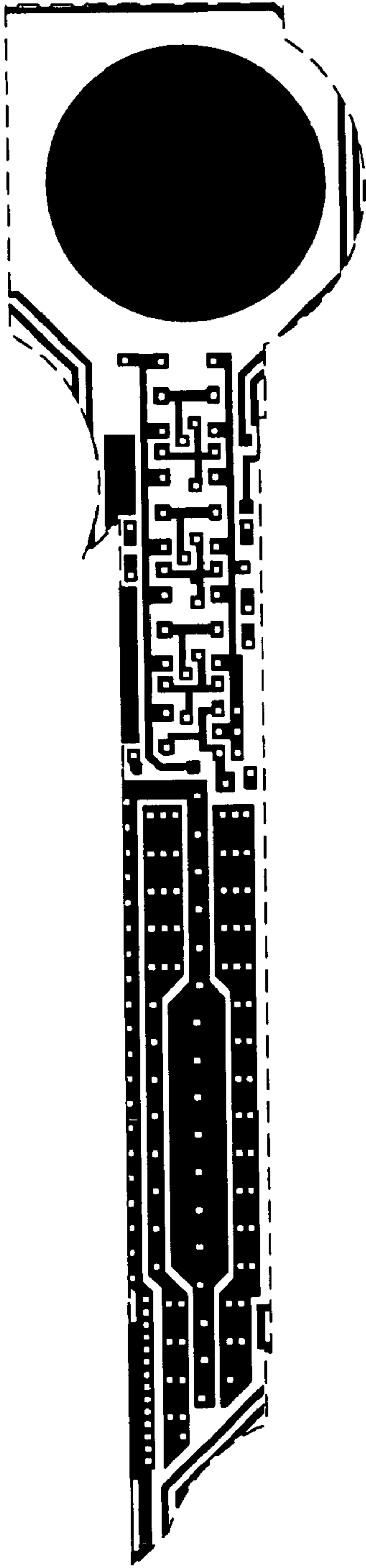
Metal 1 mask
