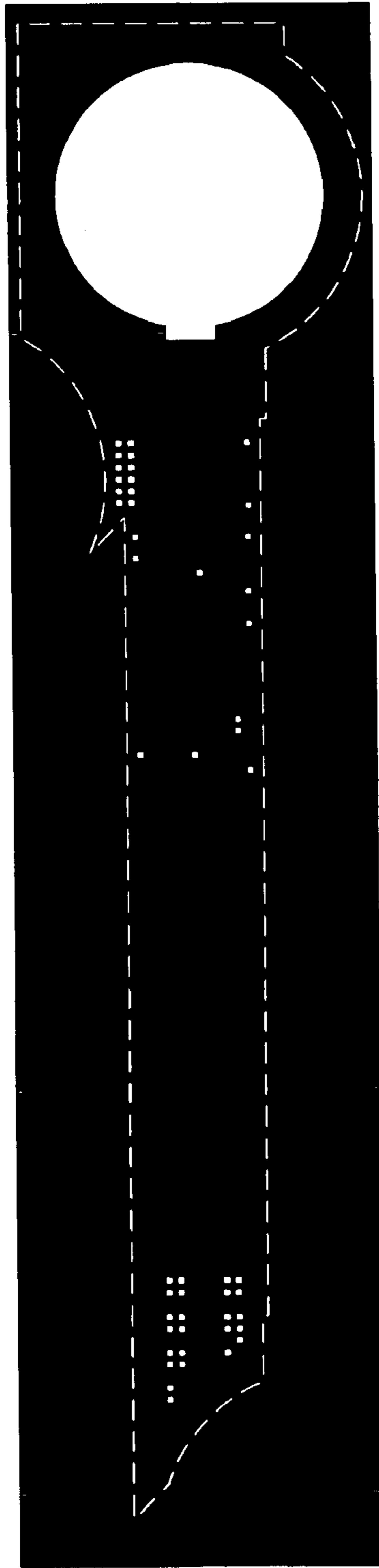
Via 1 mask
