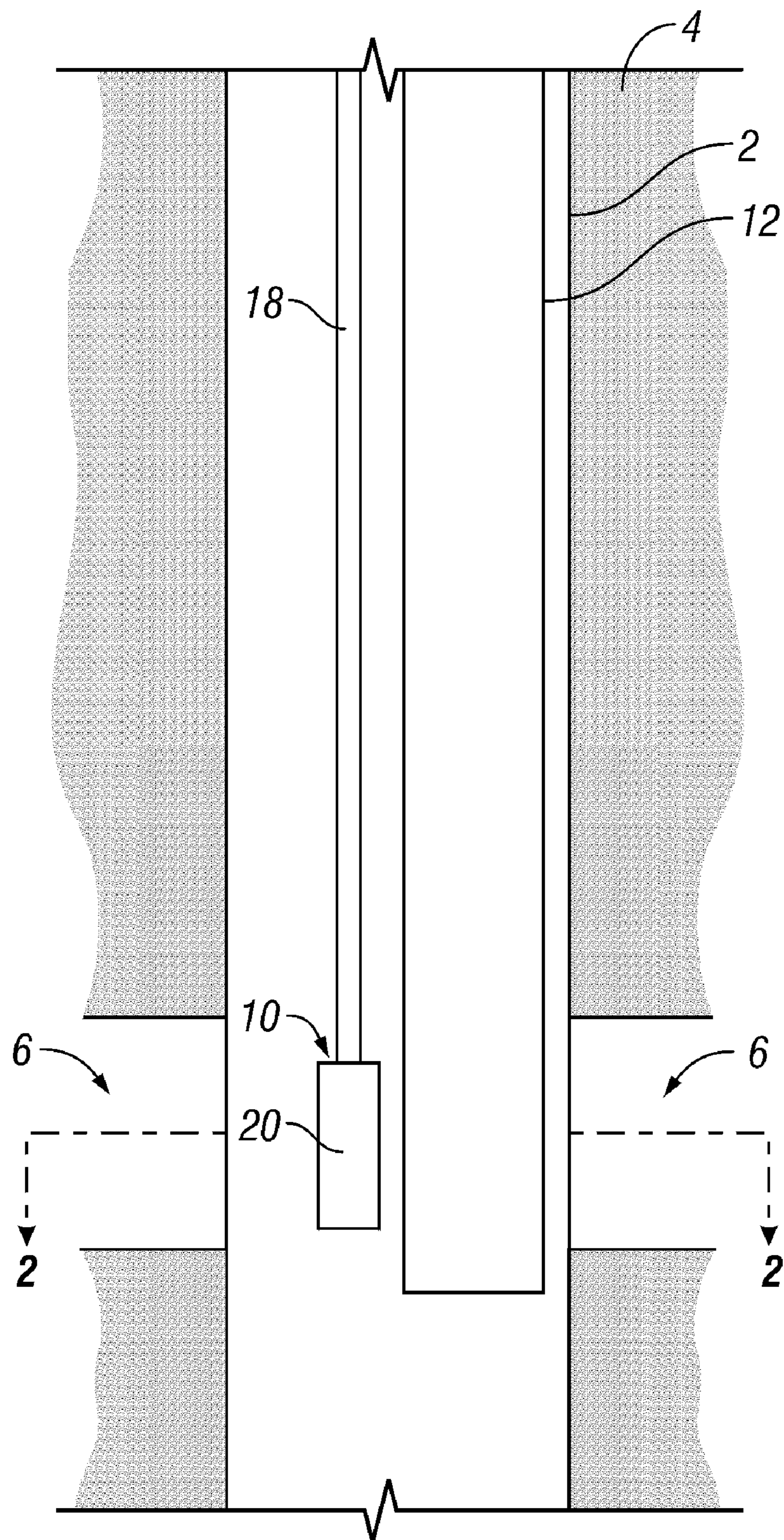
FIG. 1 (Prior Art)
