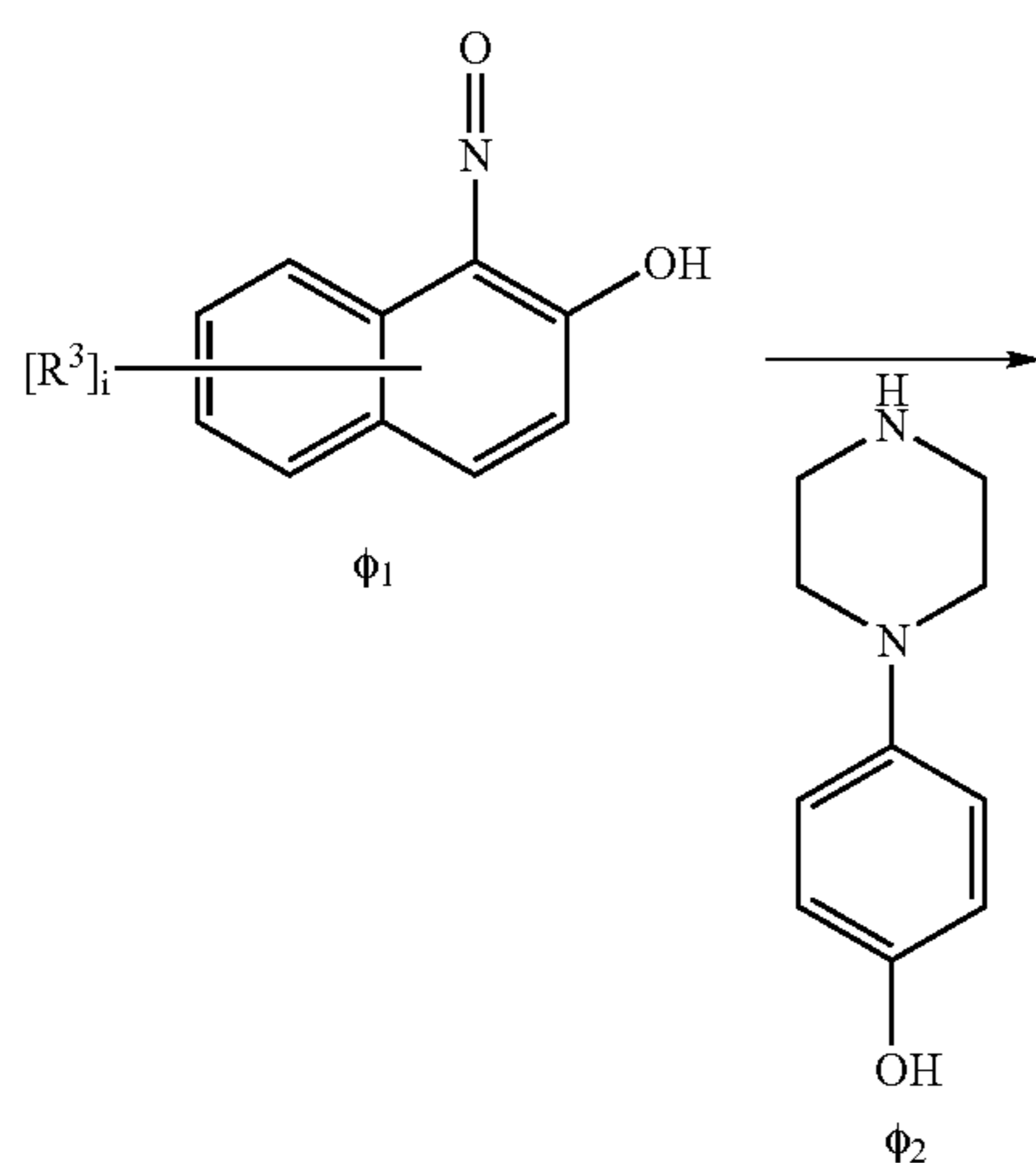
Reaction Sequence J
