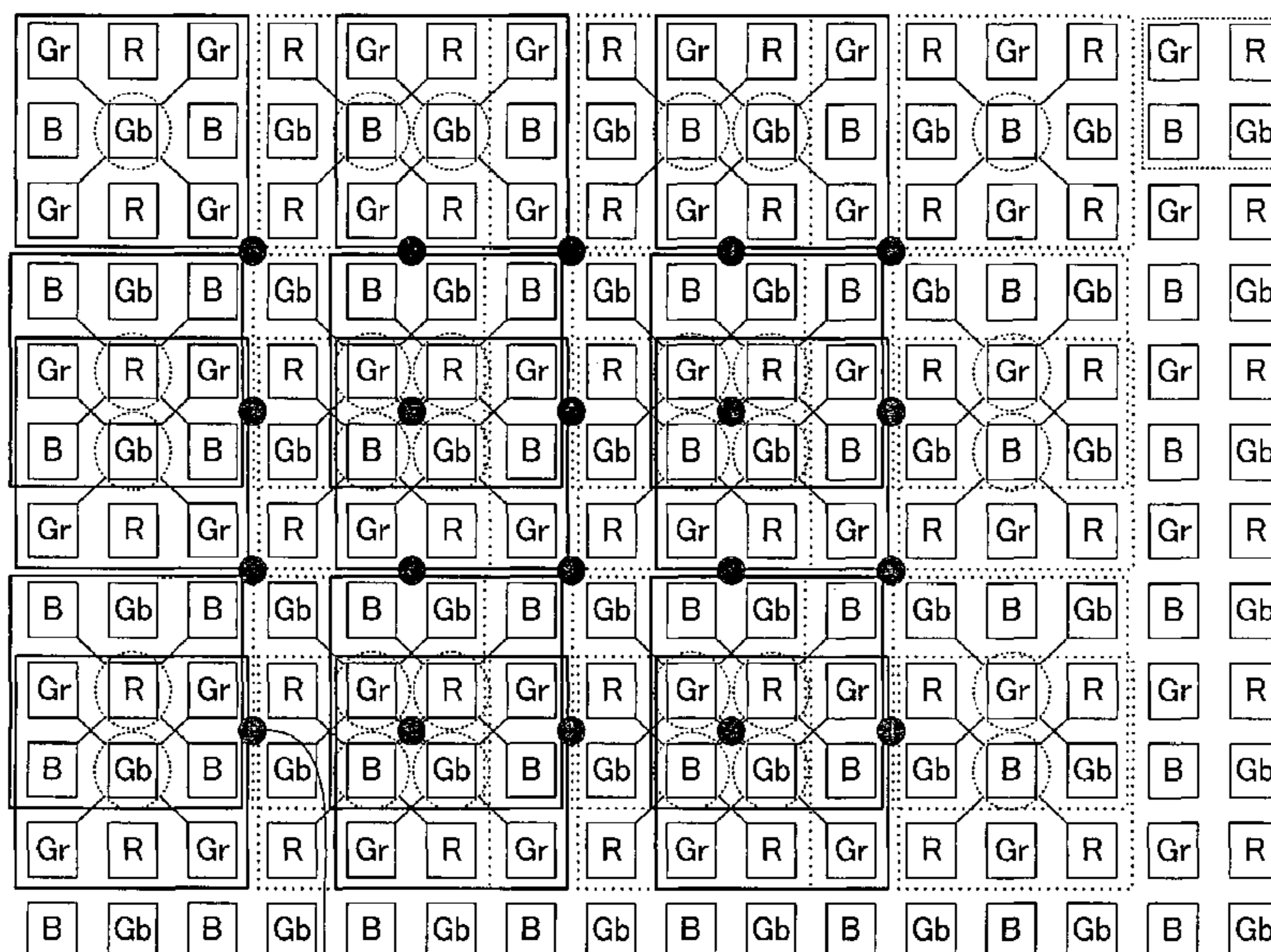
Y PIXEL WEIGHT CENTER ARRANGEMENT IN OUTPUT OF FILTER 92 FOR CORRECTING WEIGHT CENTER IRREGULARITY
