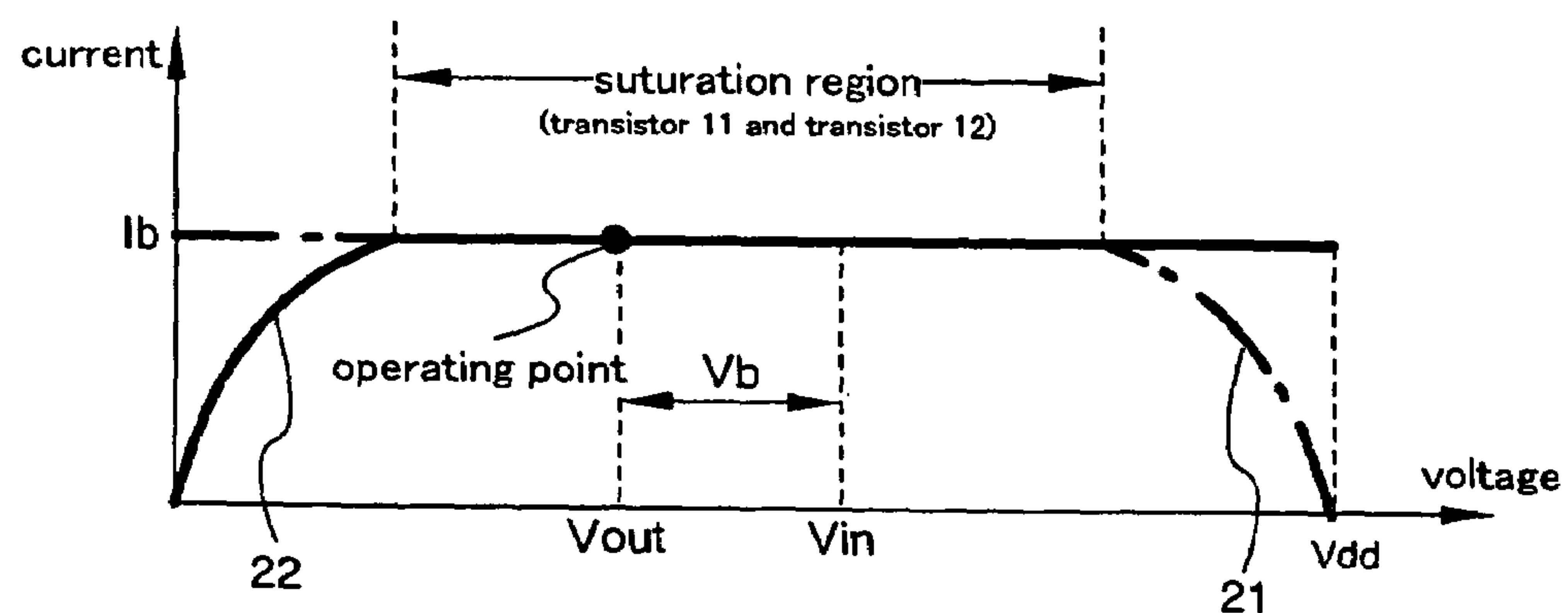
Fig. 5B V_{gs1} = V_{gs2} = V_b
