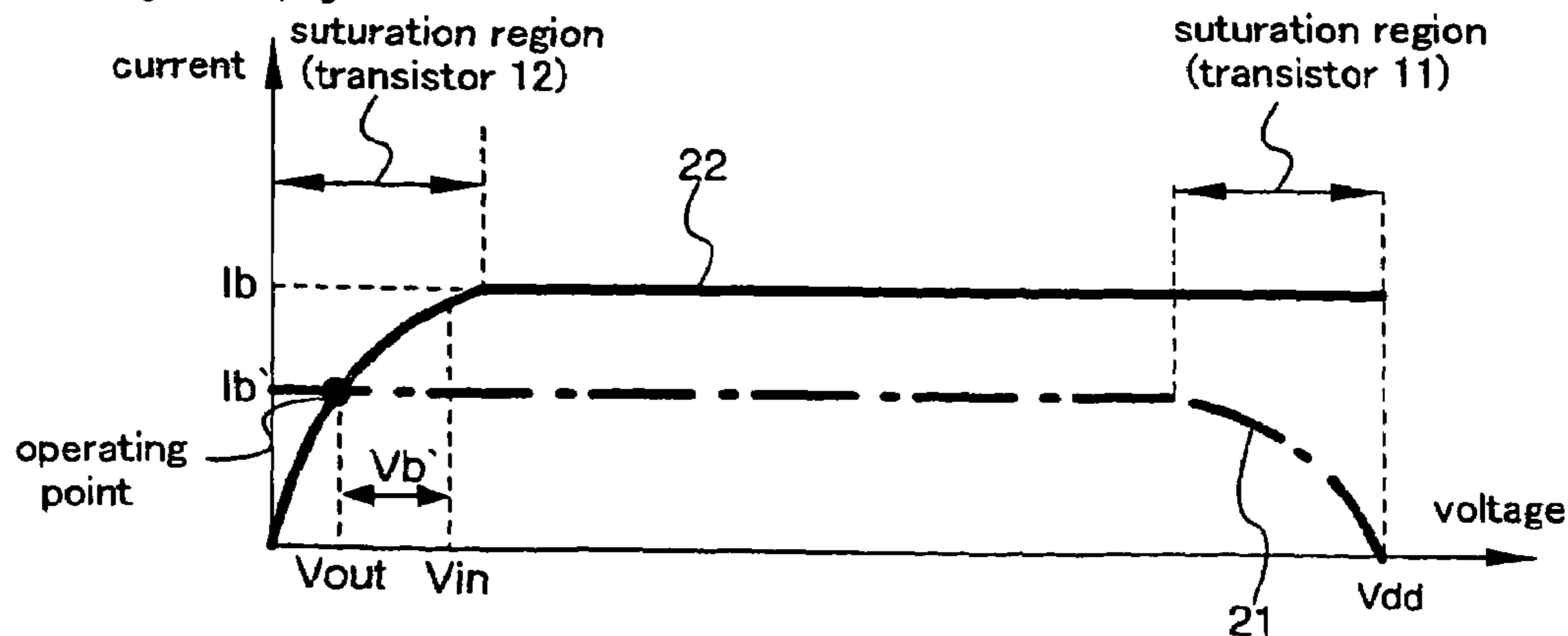
Fig. 5C V_{gs2} = V_b, V_{gs1} = V_b'
