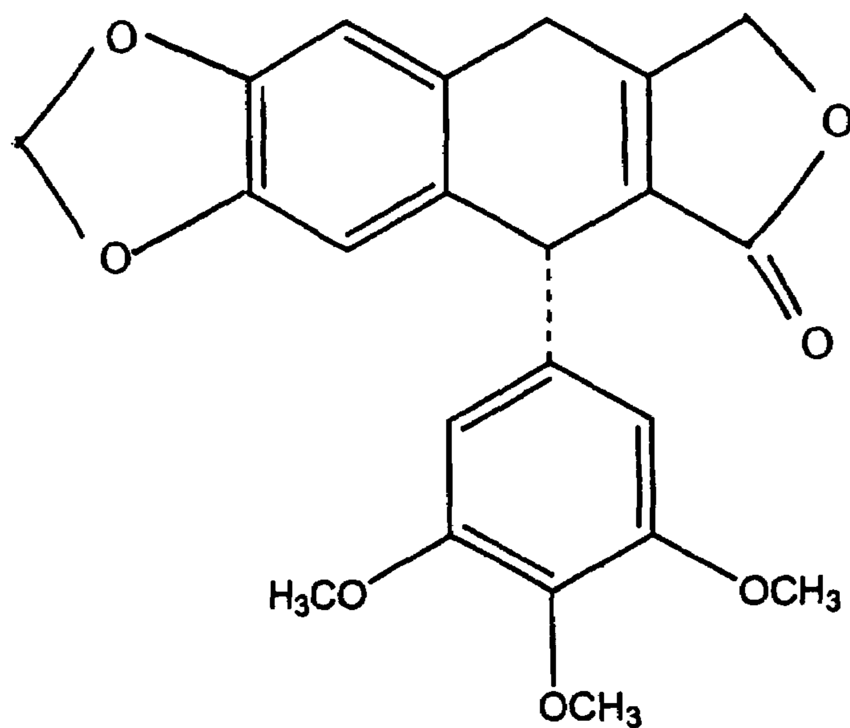
\beta -apopicropodophyllin
