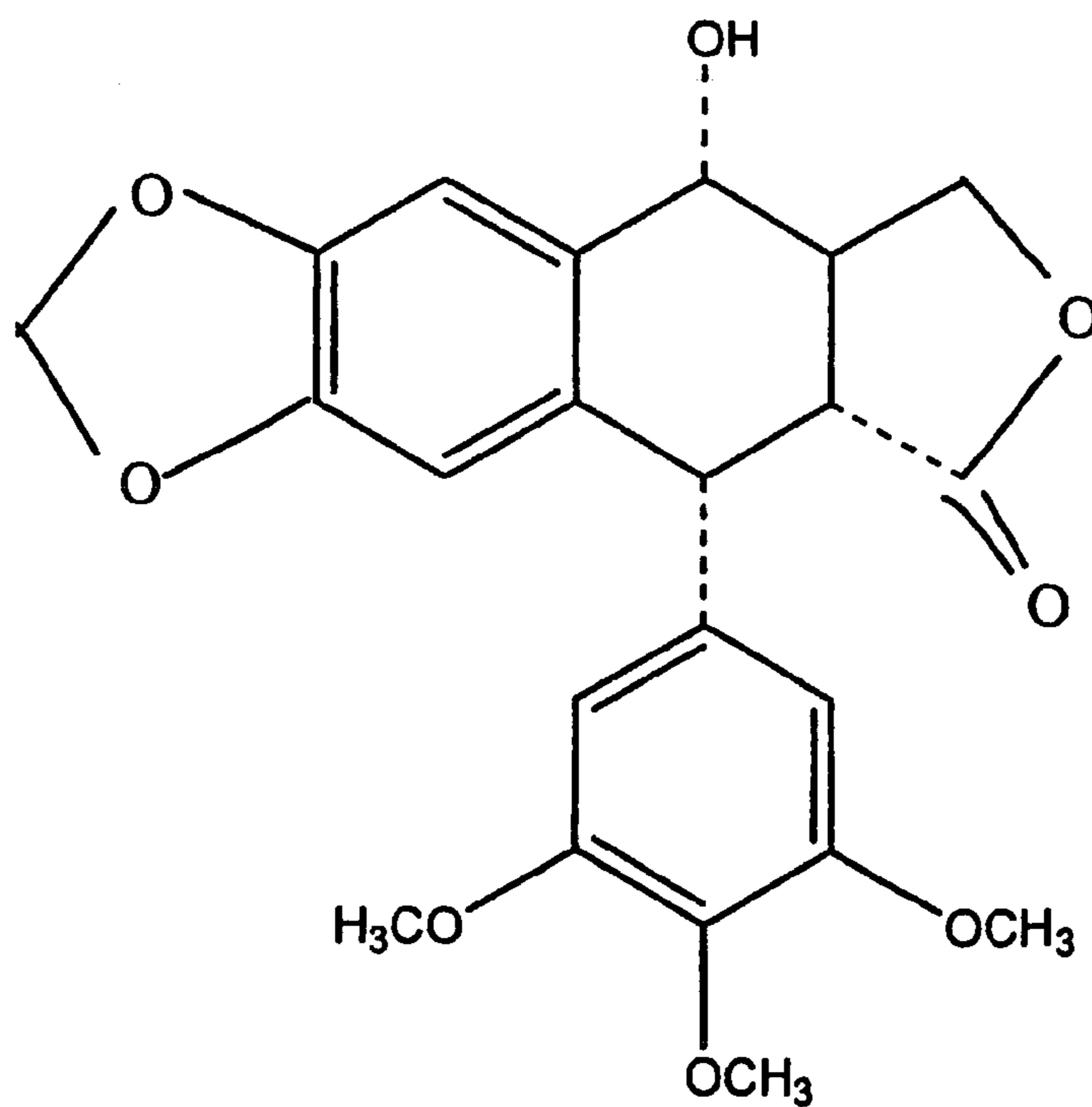
Podophyllotoxin
