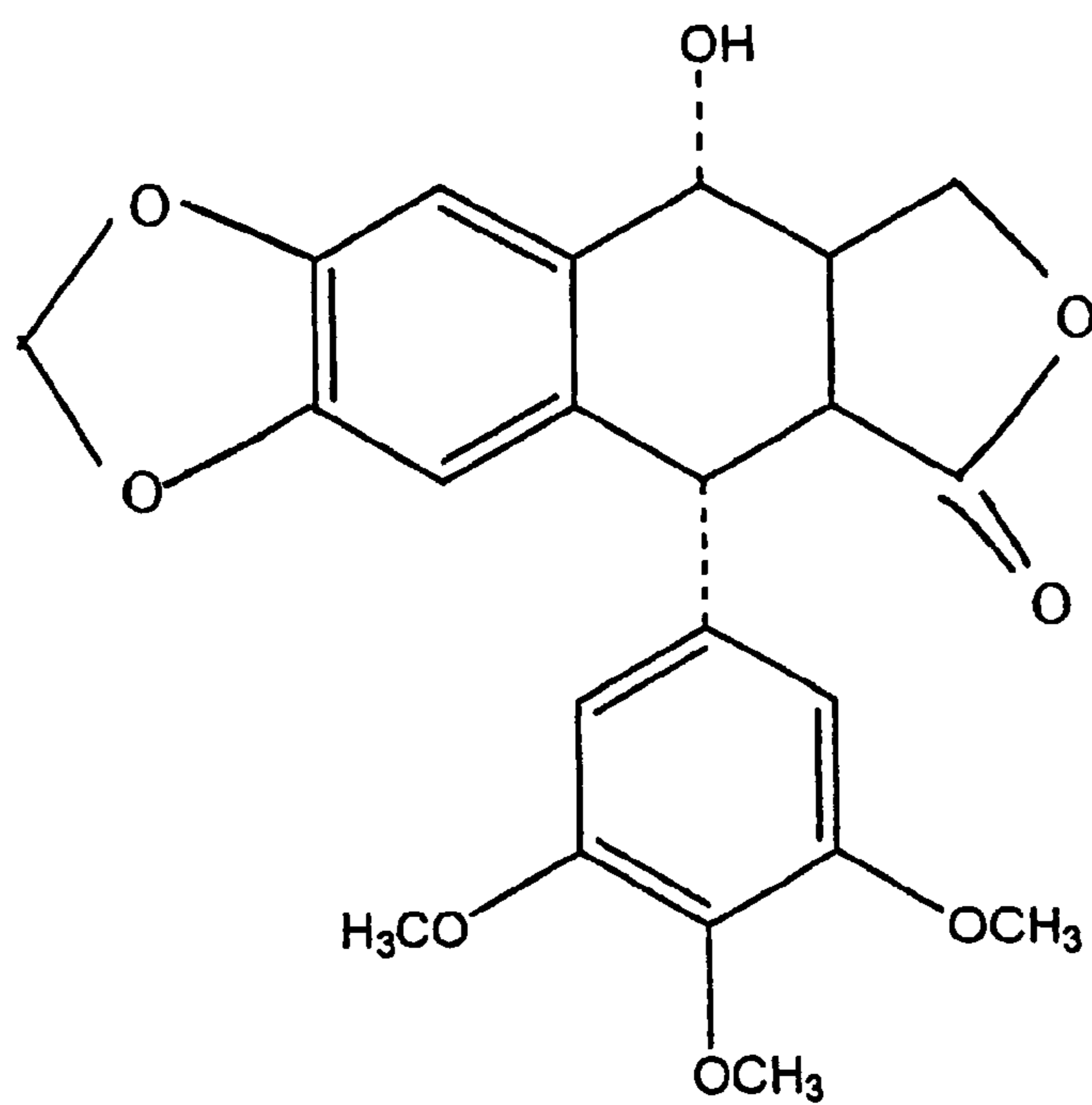
Picropodophyllin
