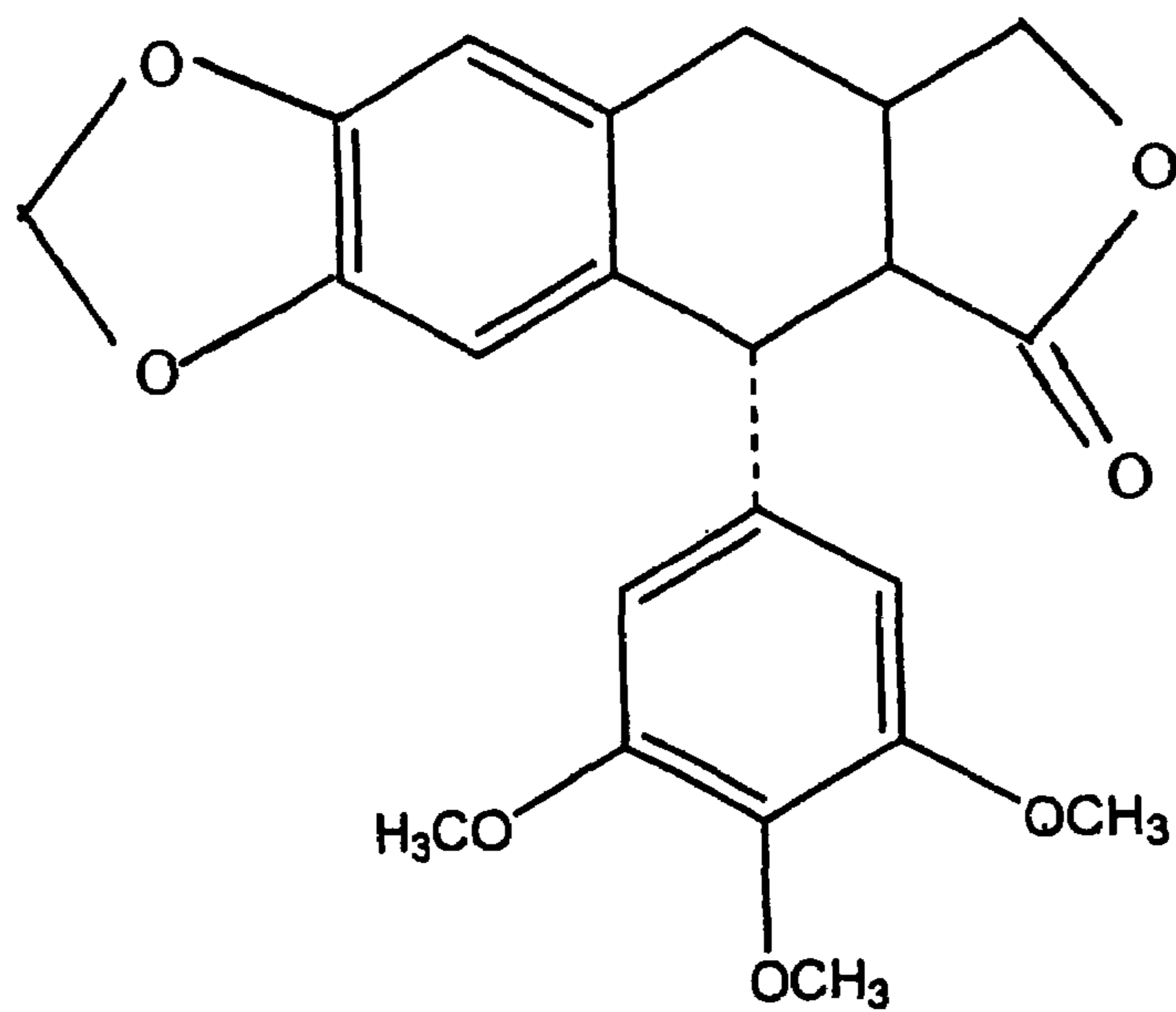
Deoxypicropodophyllin
