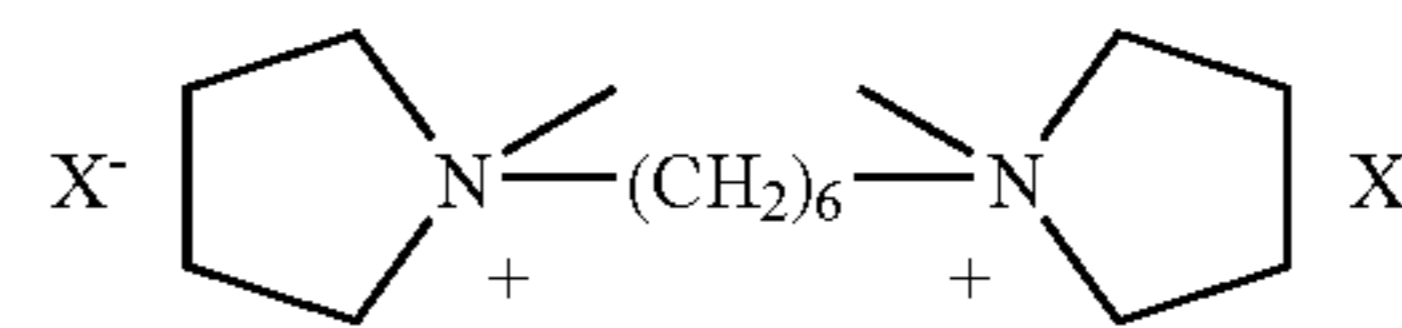
Hexamethylene-1,6-bis-(N-methyl-N-pyrrolidinium) dication
