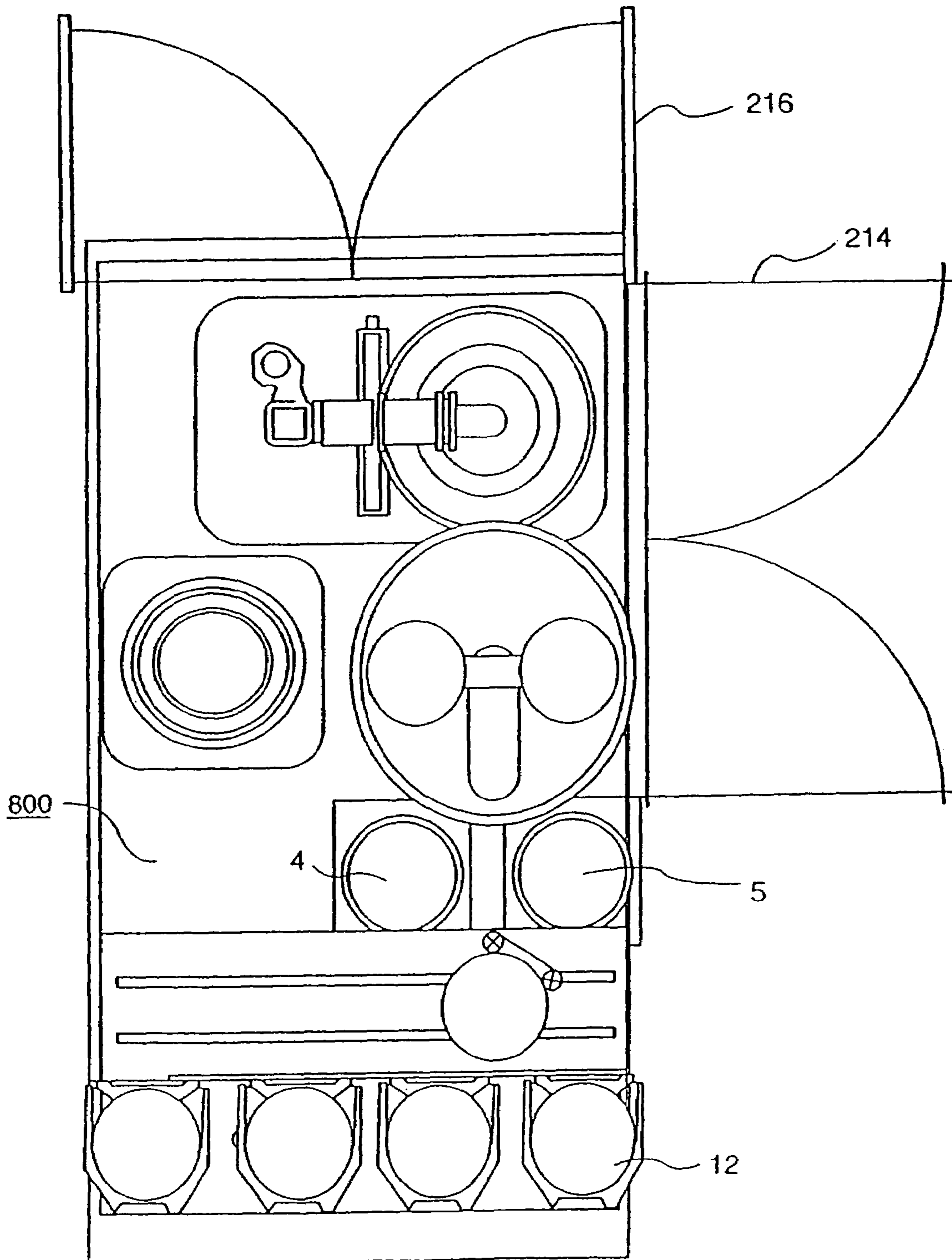
FIG. 9 PRIOR ART
