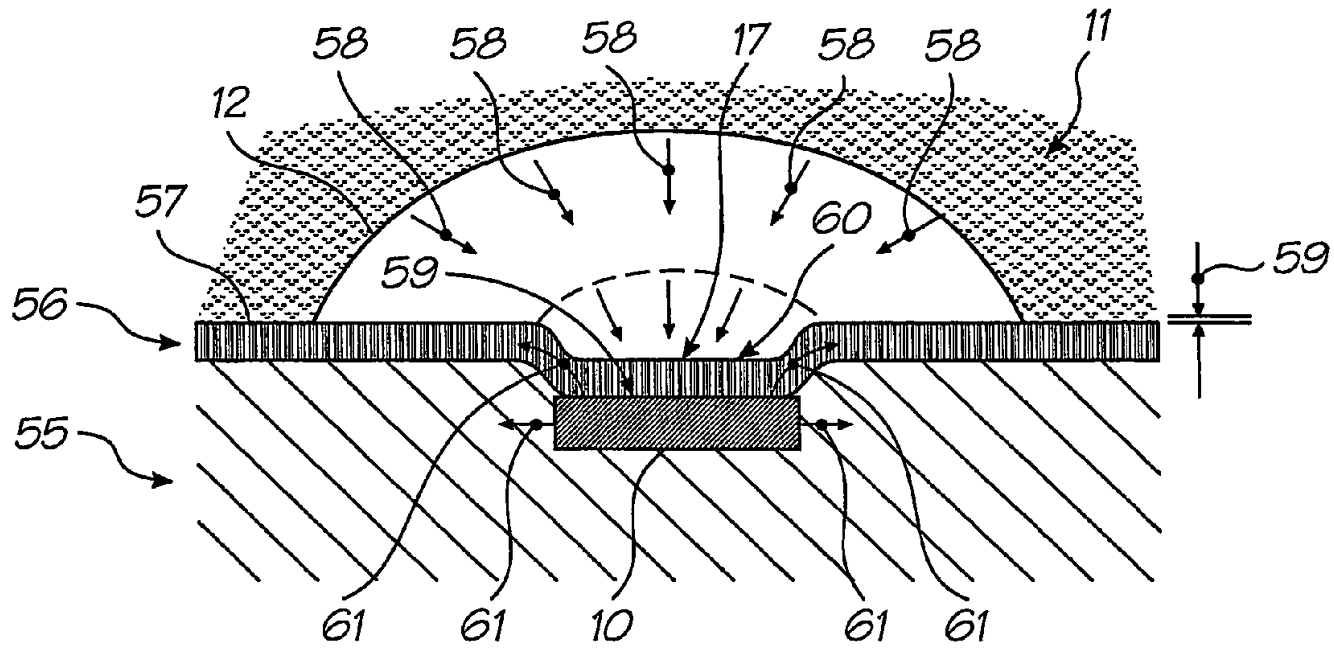
FIG. 47 (PRIOR ART)
