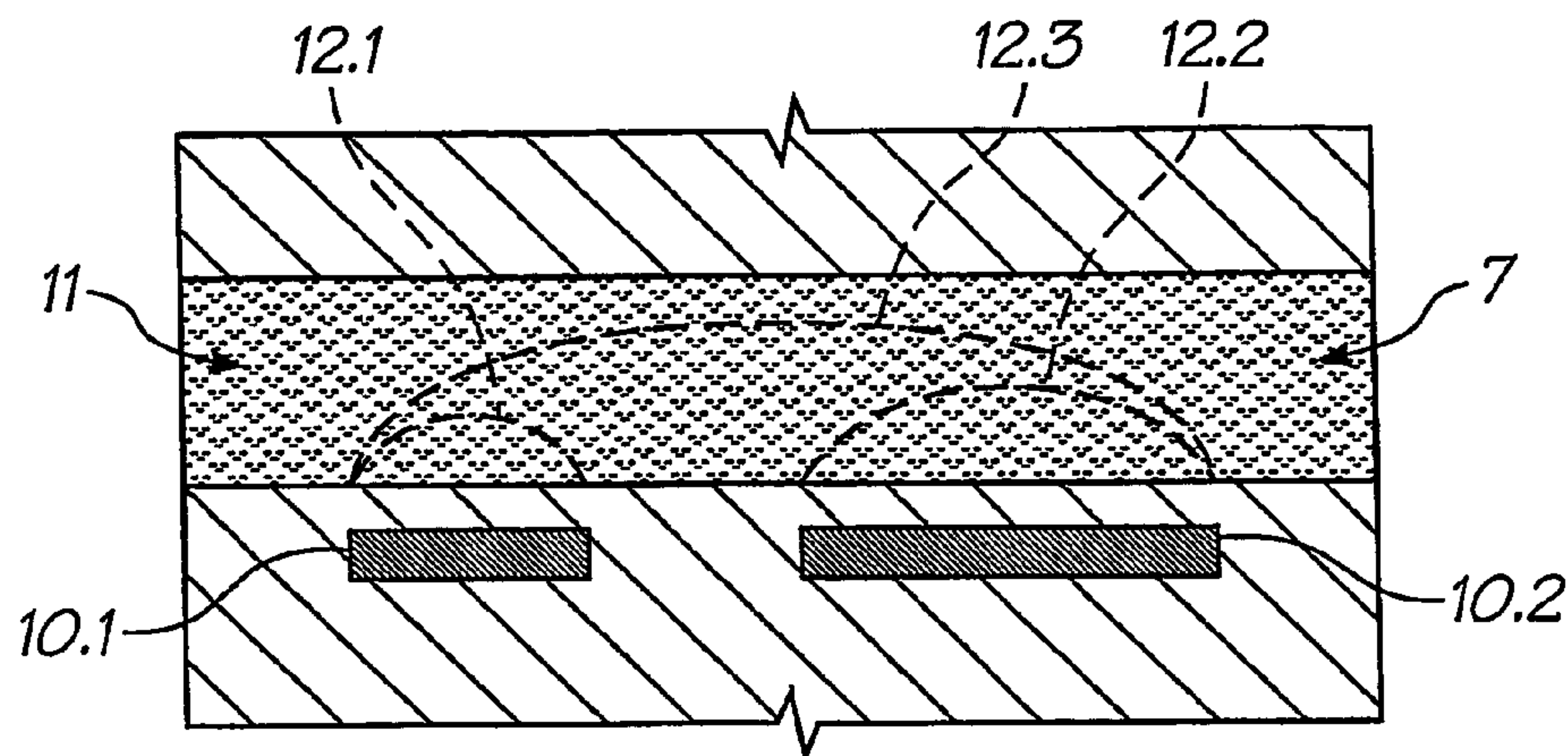
FIG. 52 (PRIOR ART)
