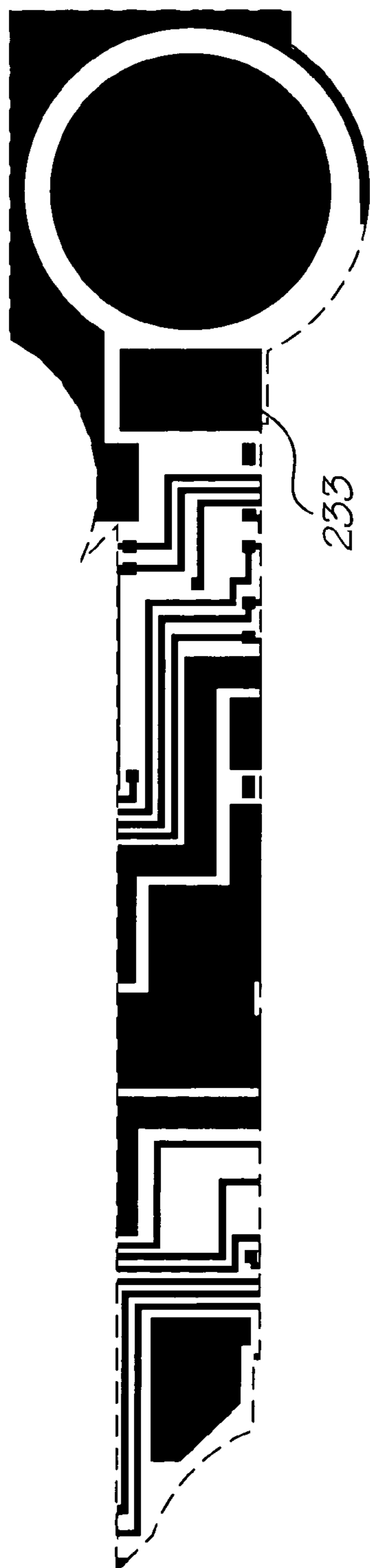
Metal 2 mask
