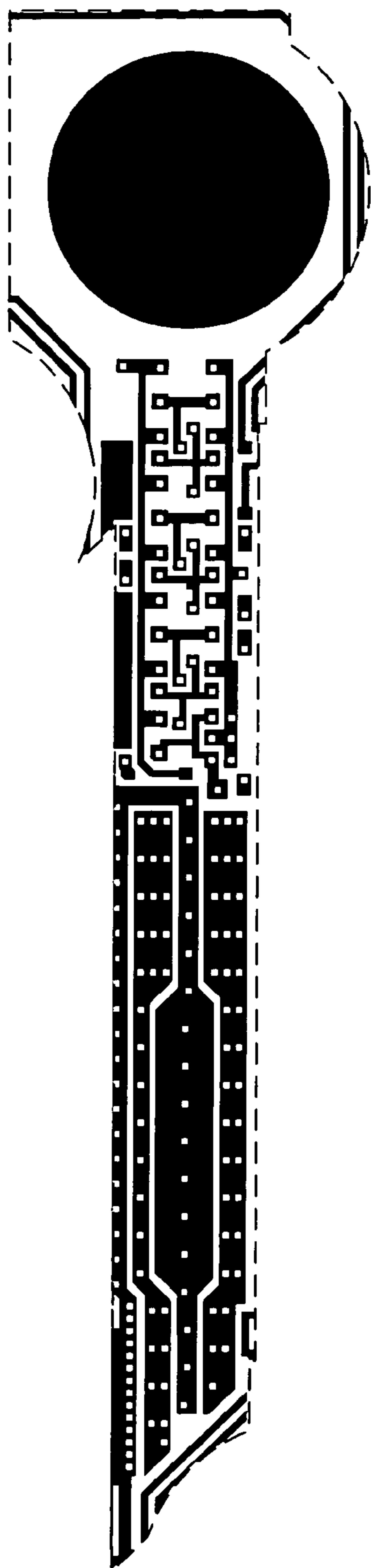
Metal 1 mask
