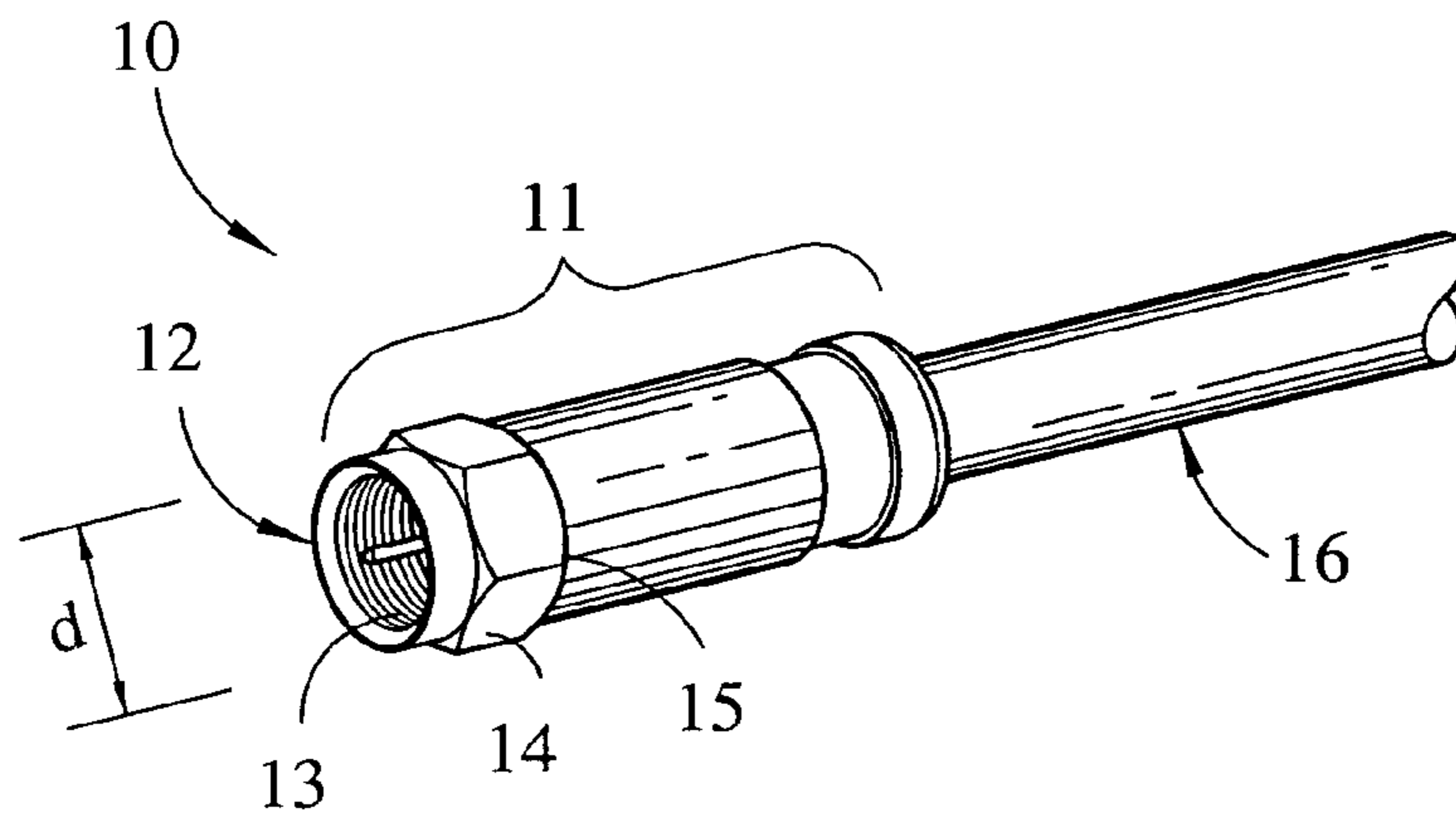
FIG. 1 PRIOR ART
