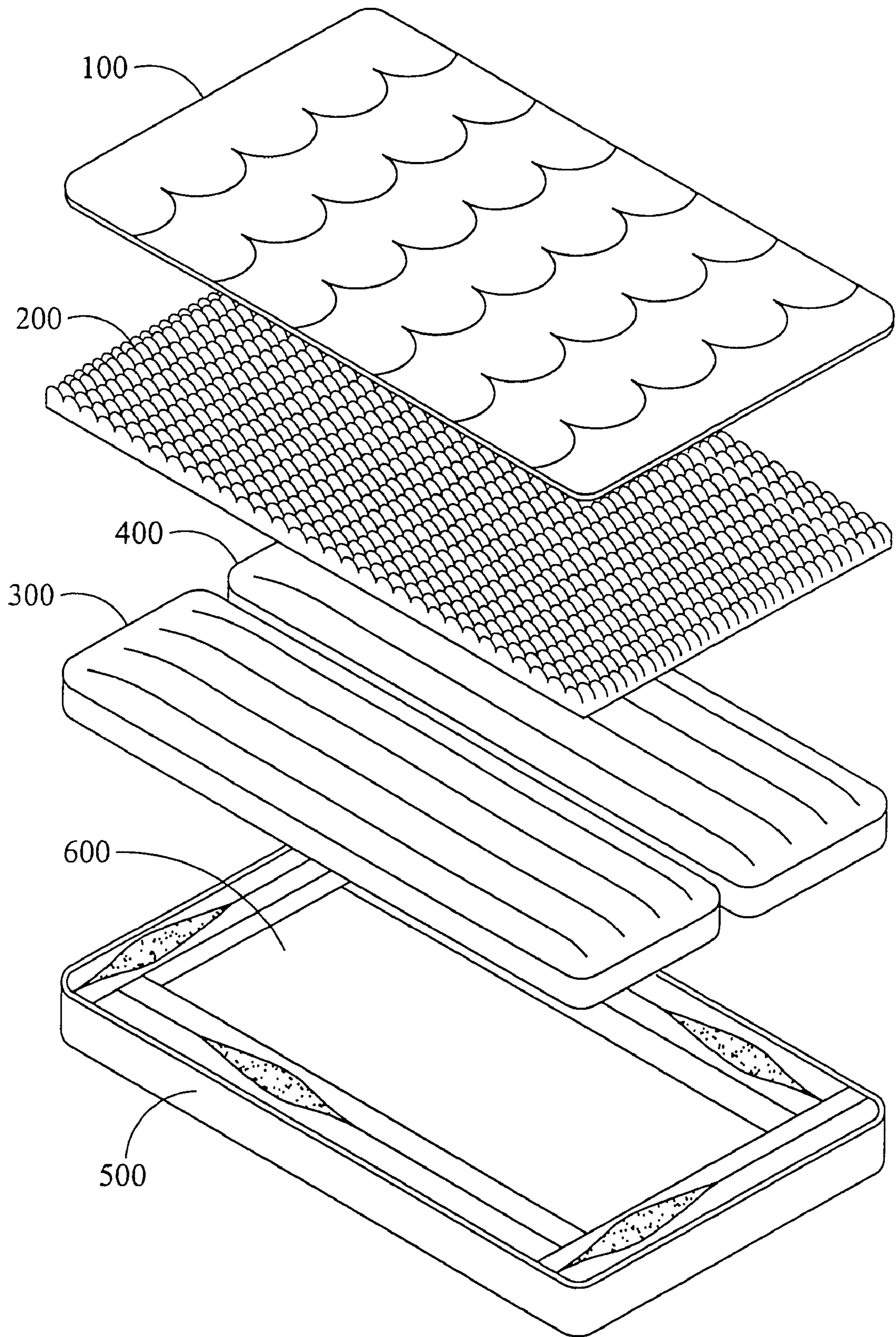
FIG. 11 ( PRIOR ART )
