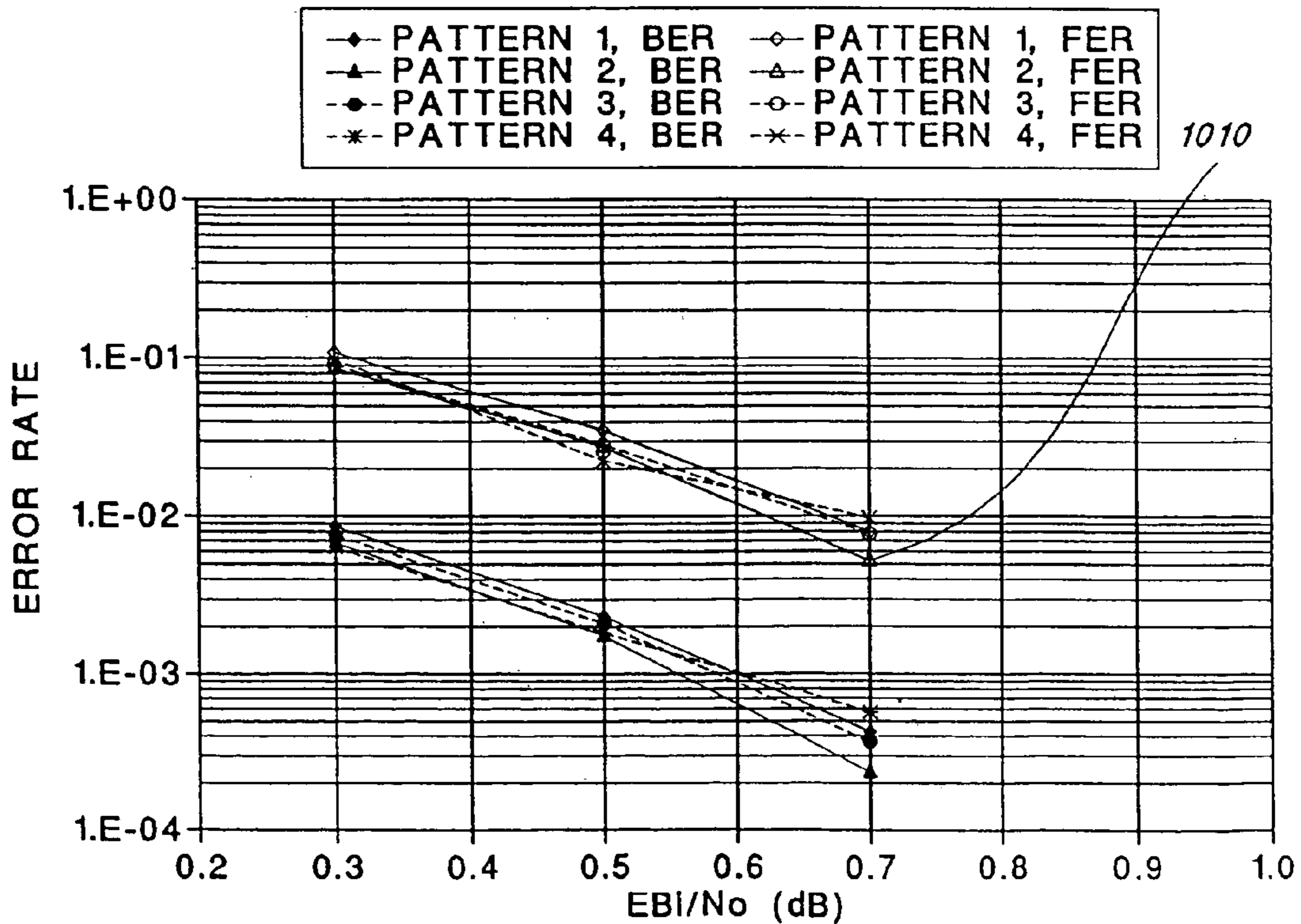
FIG. 10 PERFORMANCE OF CODE #1, FRAME SIZE=512
