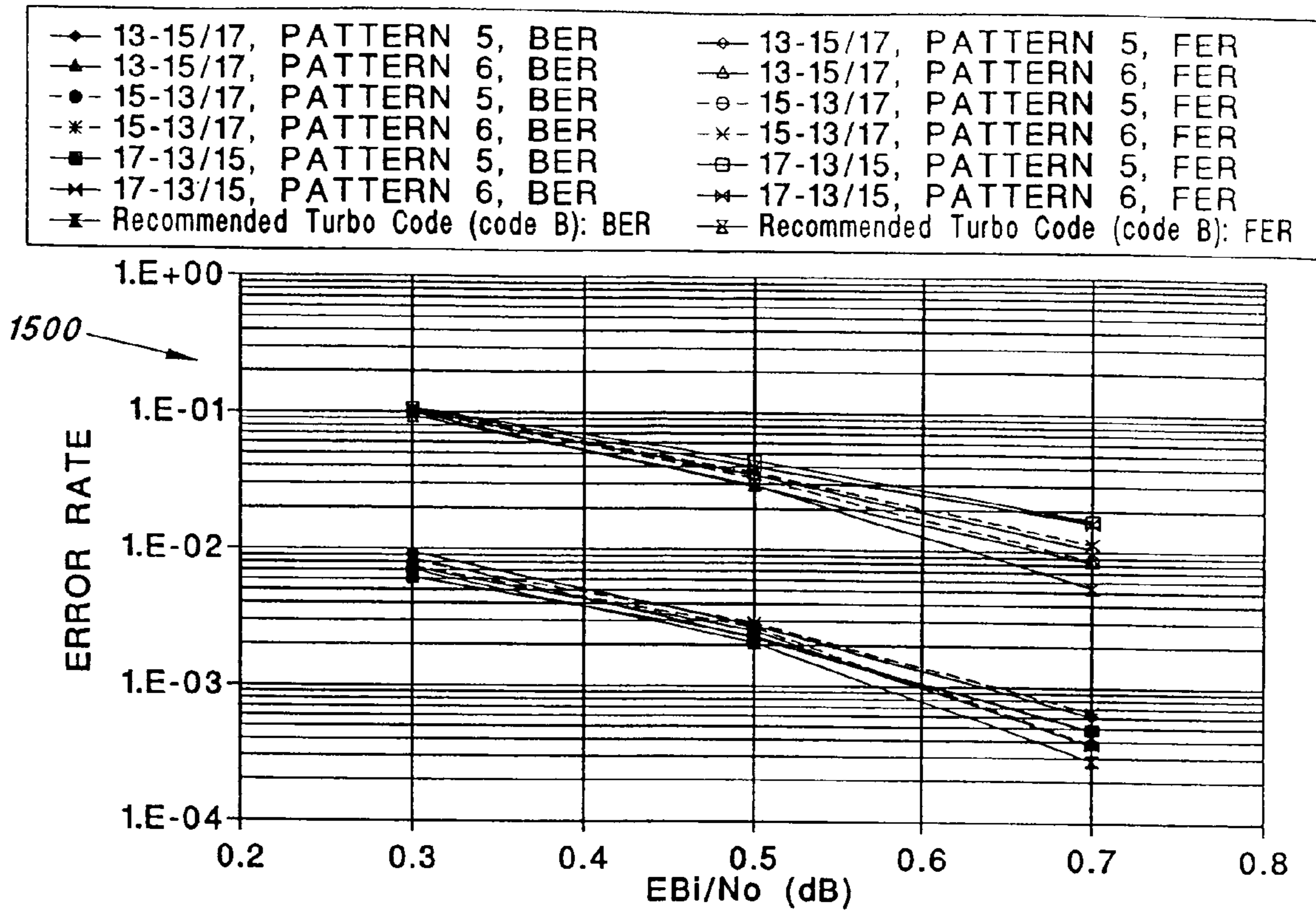
FIG. 15 COMPARISON AGAINST OTHER PUNCTURING SCHEMES, FRAME=512
