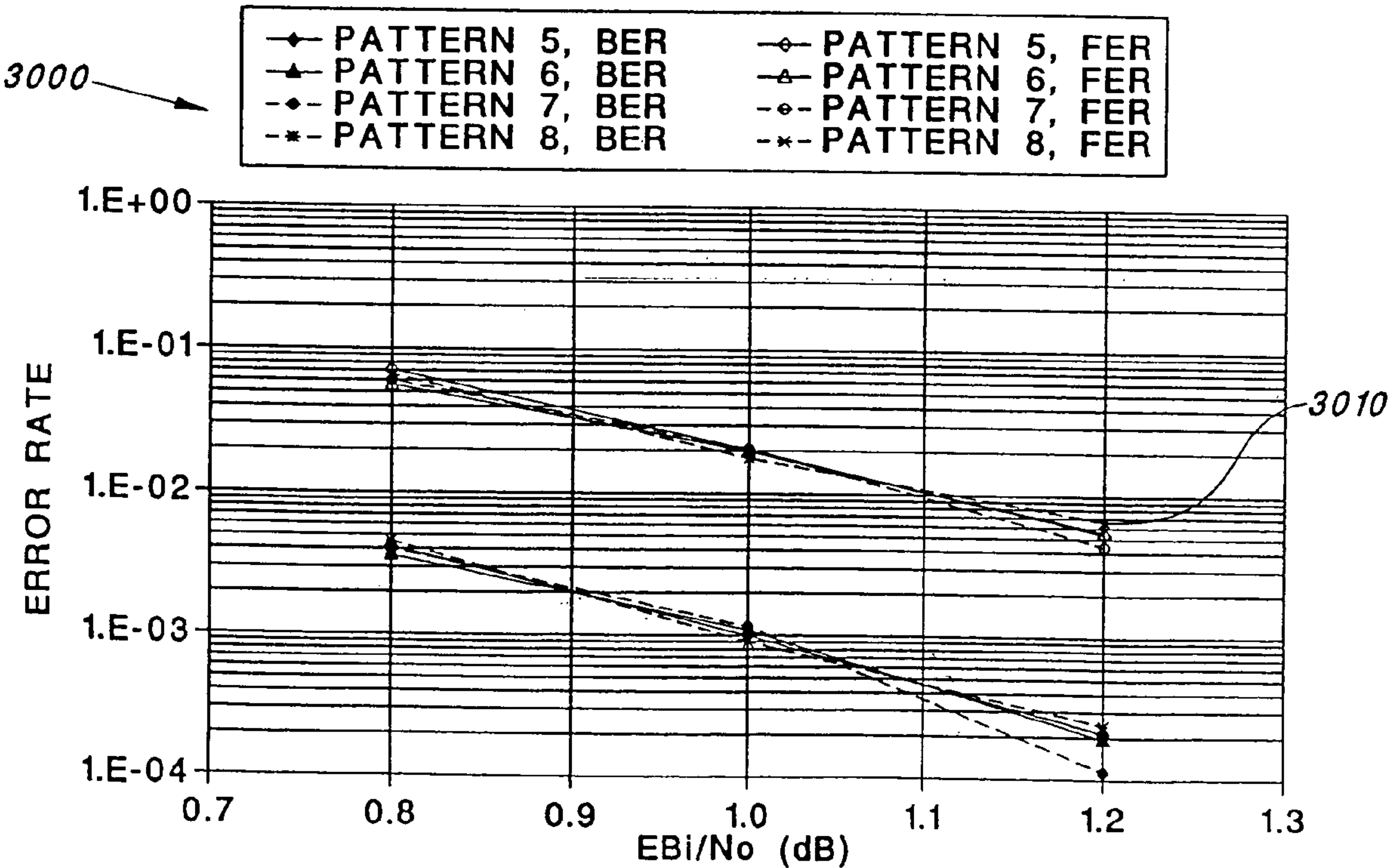
RATE 3/8 REVERSE LINK TURBO CODES, FRAME=512, AWGN CHANNEL
