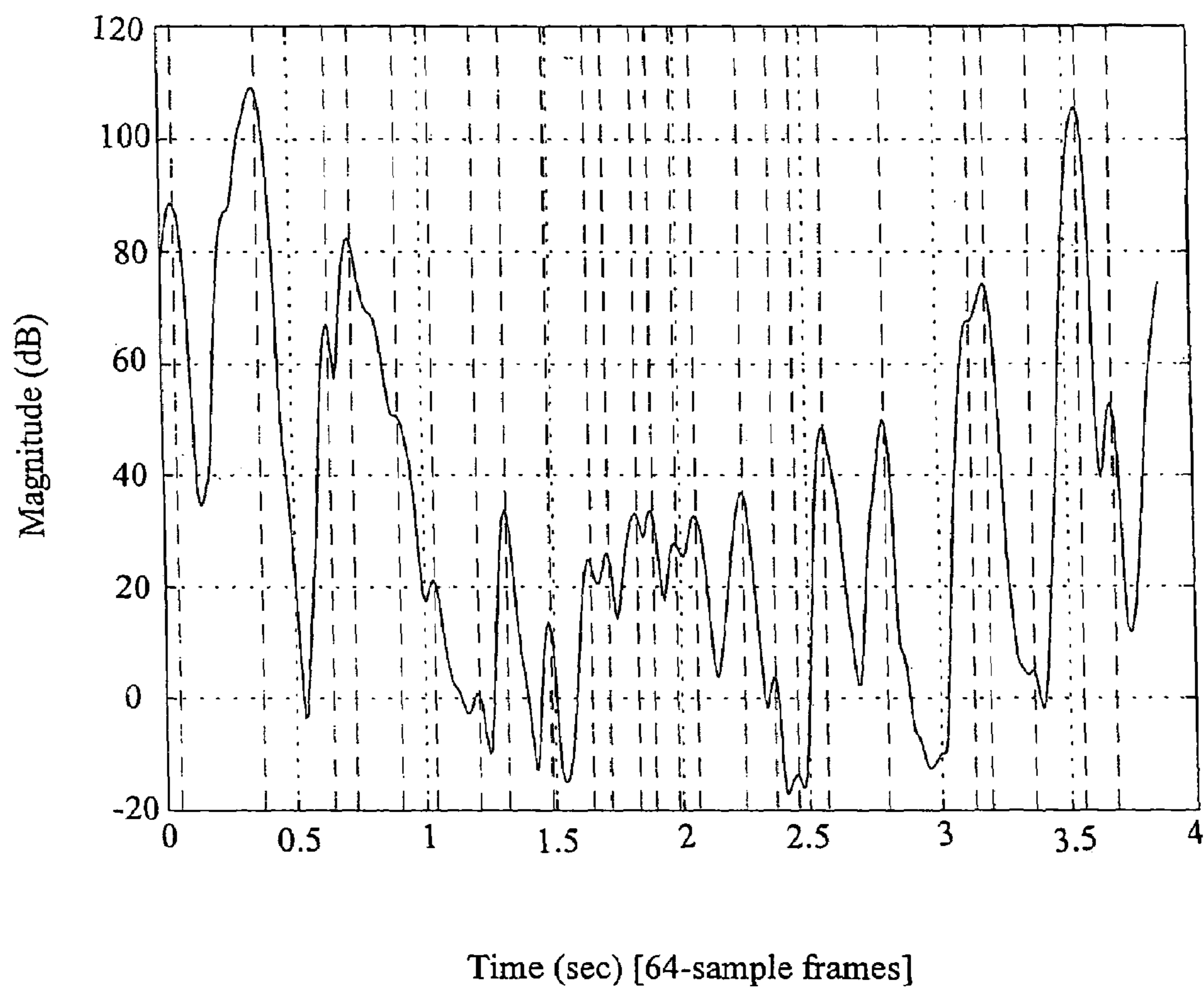
Landmarks in L4 Norm
